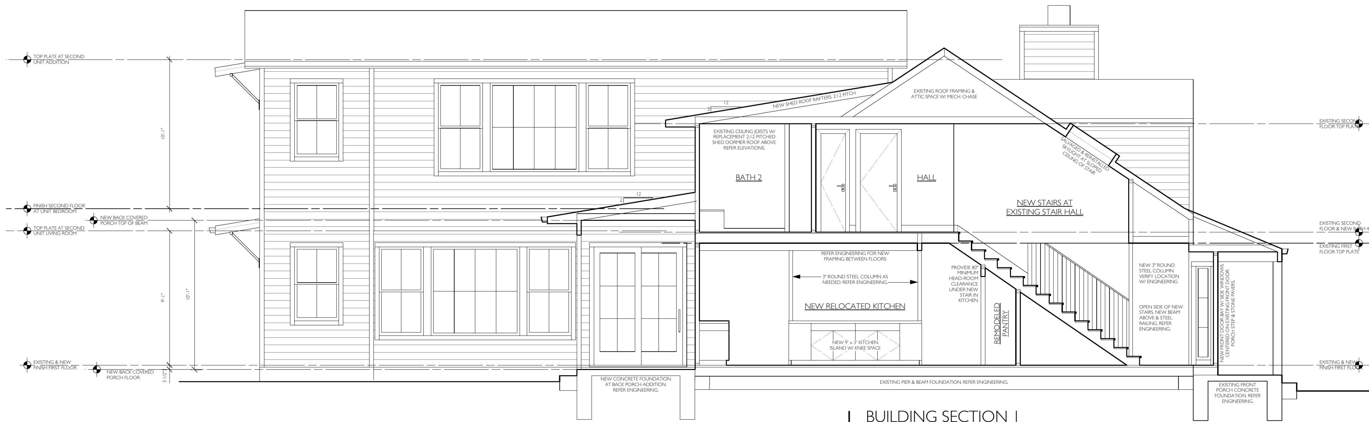
BUILDING SECTION 1 SCALE: 1/4" = 1'-0"
