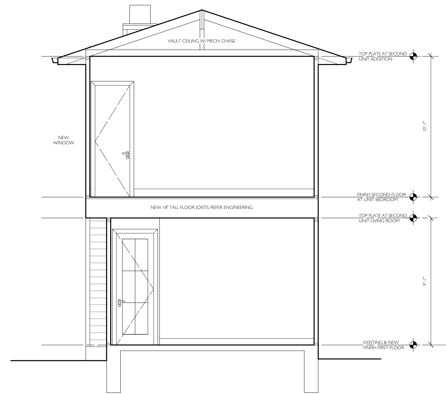
2 BUILDING SECTION 2 SCALE: 1/4" = 1'-0"
