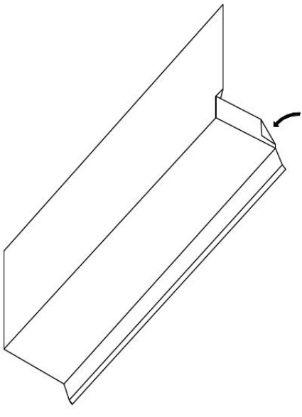
STEP 4 - FOLD OVER OUTER CORNER TO CREATE SAFETY EDGE - END DAM MUST EXTEND TO FACE OF CLADDING
