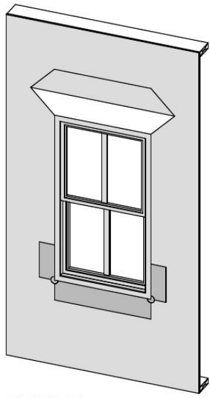
STEP 5 - INSTALL WINDOW PLUMB, LEVEL AND SQUARE PER MANUFACTURER'S INSTRUCTIONS
