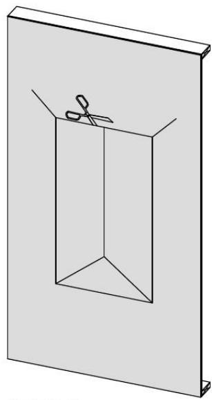
STEP 2 -MODIFY "1" CUT IN HOUSE WRAP
