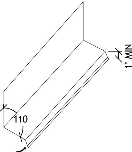
STEP 1 - FOLDED METAL FLASHING (MIN. 6% SLOPE) - FOLD FRONT FACE OF FLASHING TO CREATE SAFETY EDGE
