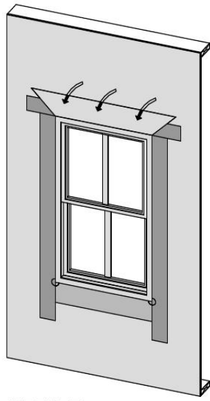
STEP 7 - FOLD DOWN HOUSEWRAP AT HEAD
