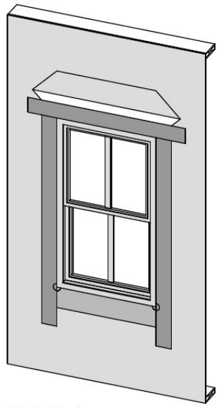
STEP 6 - INSTALL JAMB FLASHING FIRST THEN HEAD FLASHING
