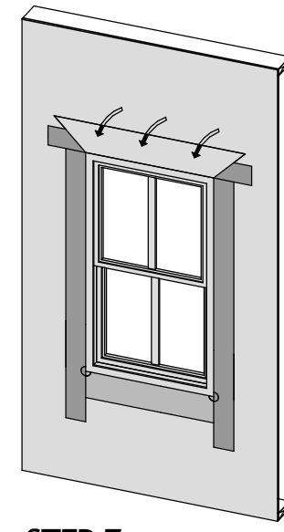
STEP 7 - FOLD DOWN HOUSEWRAP AT HEAD
