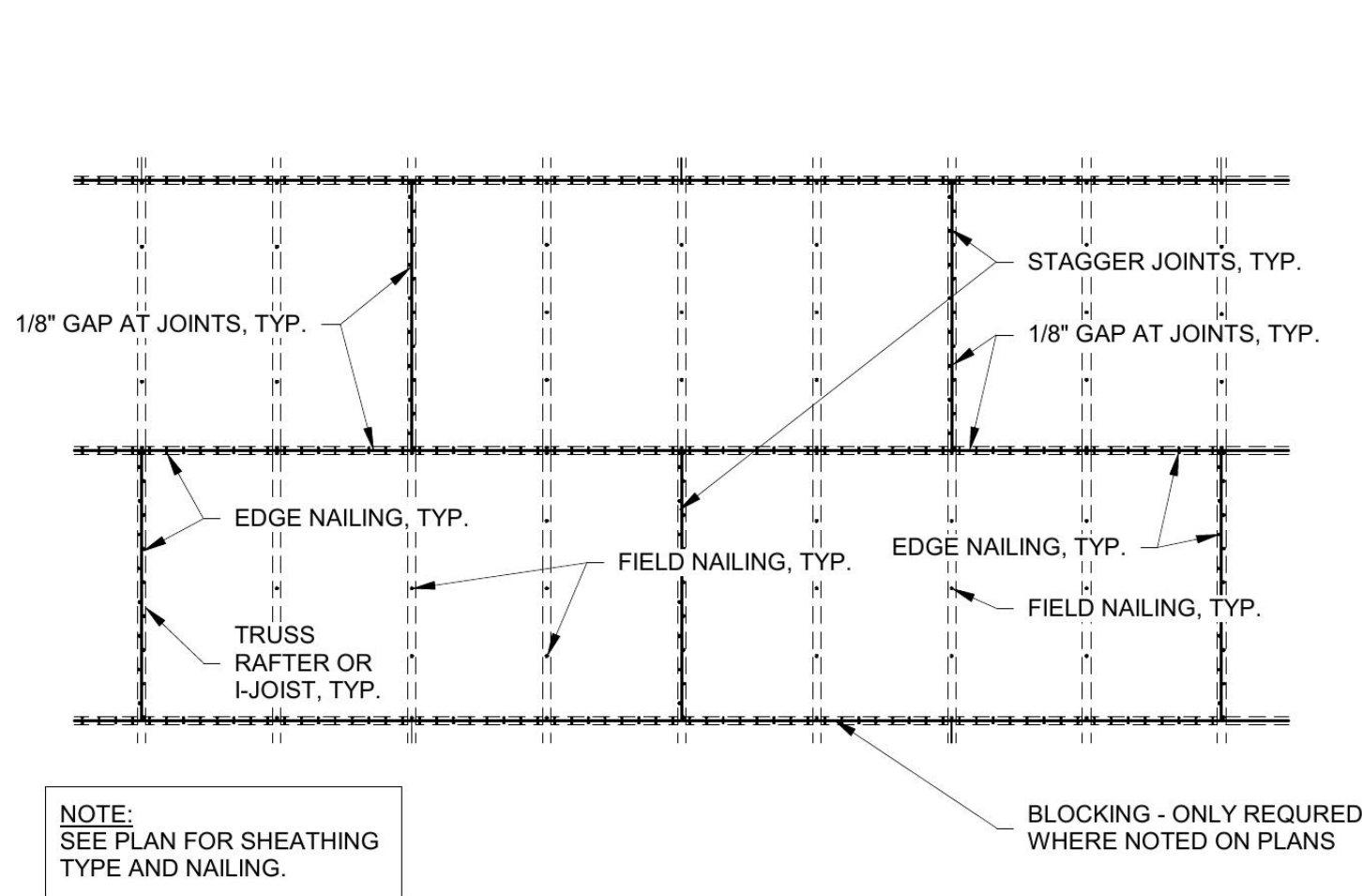
2 DIAPHRAGM NAILING 3/8" = 1'-0"
