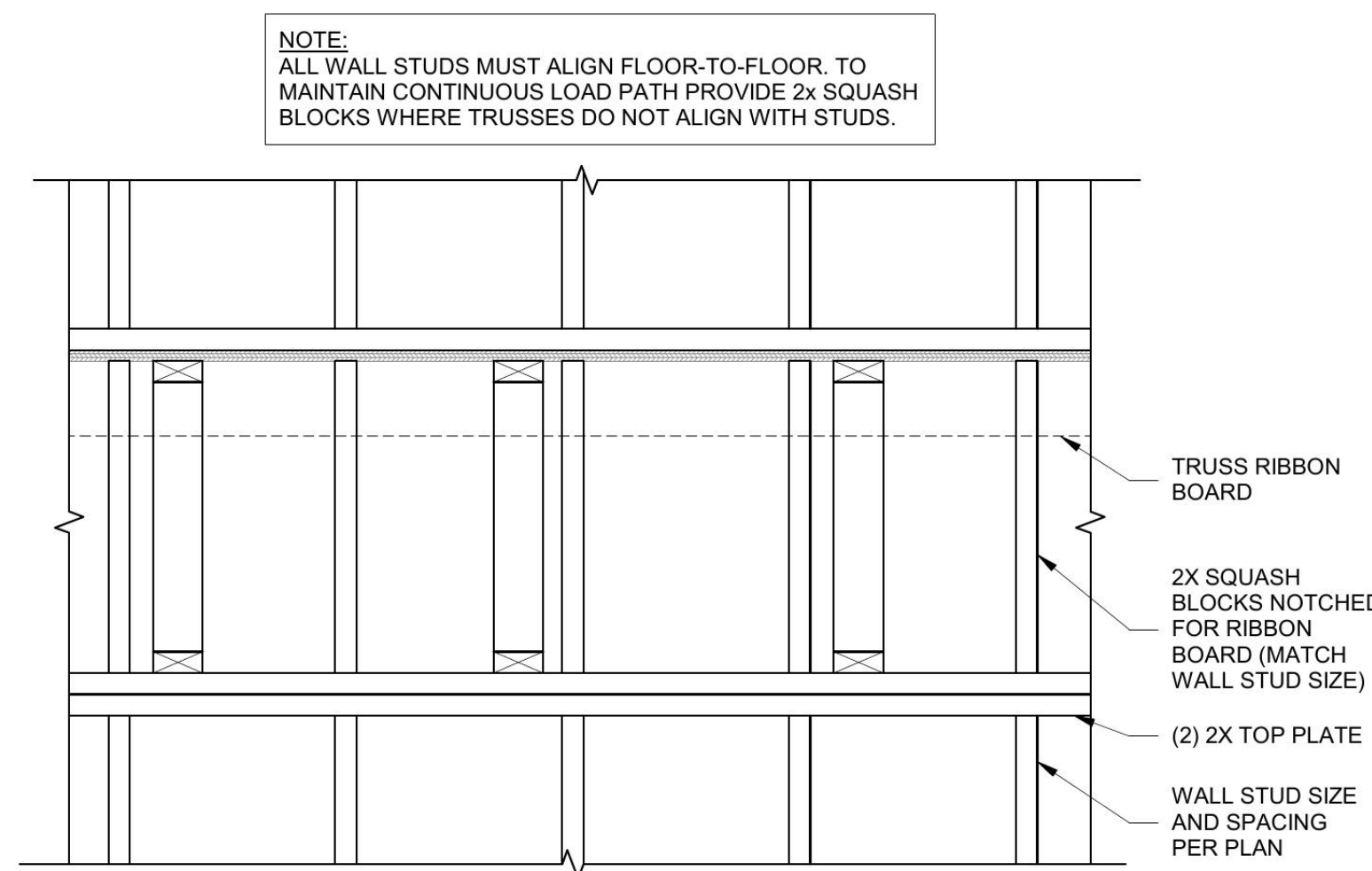
8 TYPICAL WALL FRAMING ELEVATION
