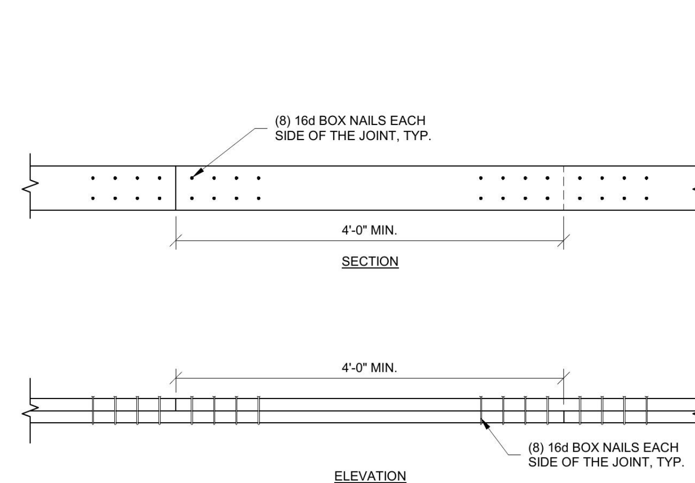
3 TOP PLATE SPLICE 1" = 1'-0"
