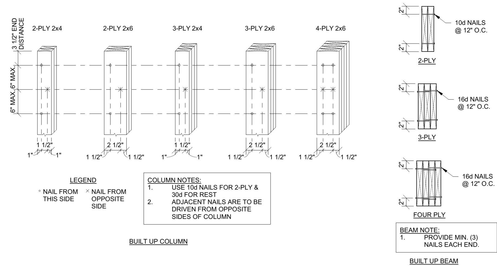
1 TYPICAL BUILT-UP MEMBERS 1" = 1'-0"
