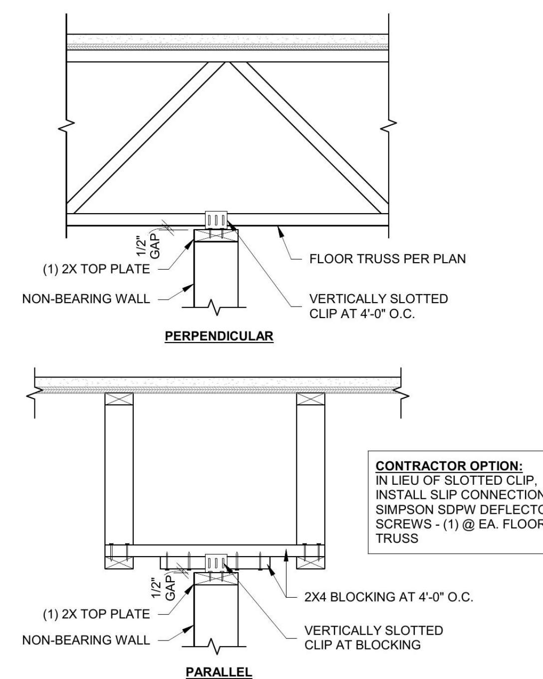
9 NON-BEARING WALL TO FLOOR TRUSS
