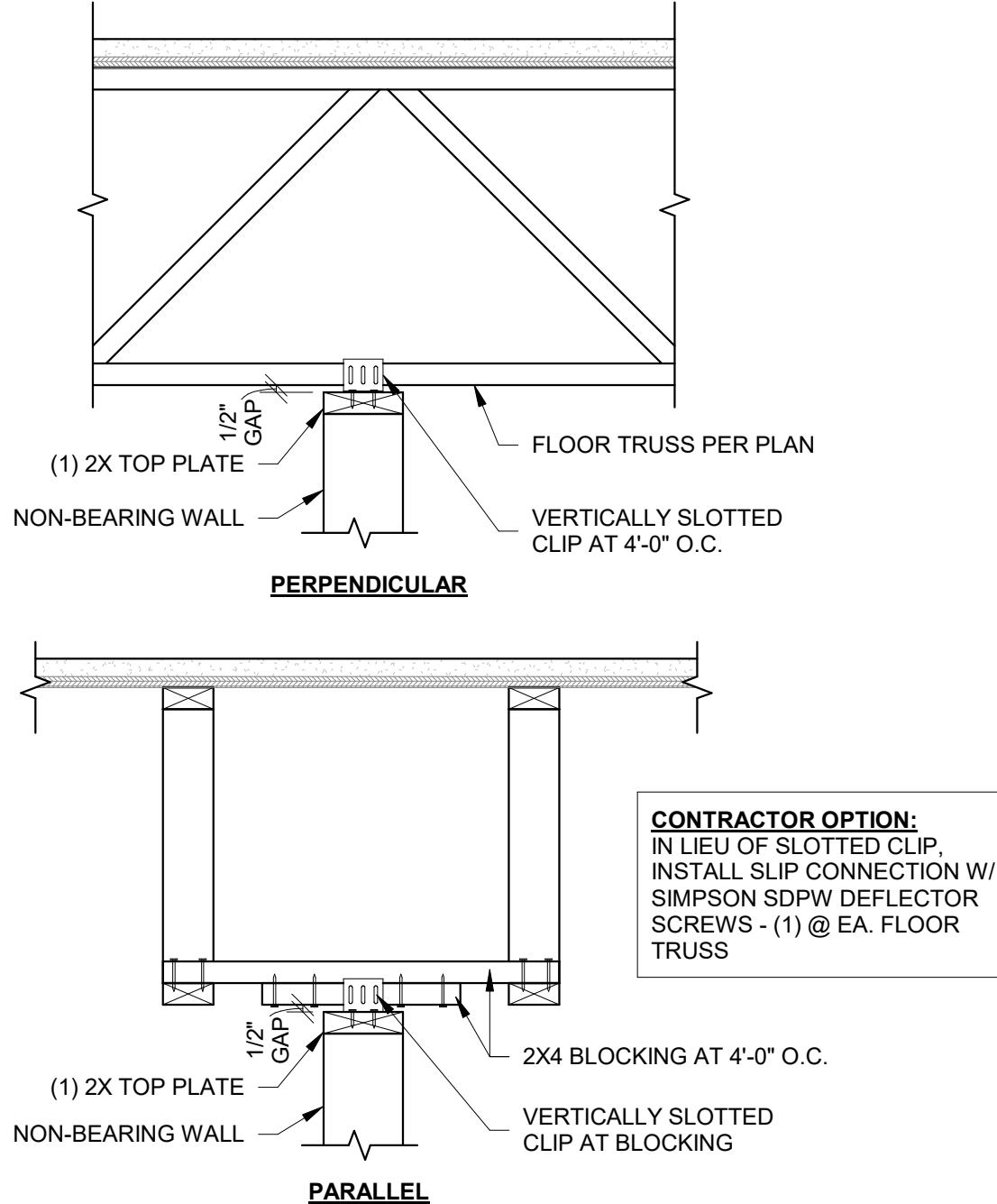
9 NON-BEARING WALL TO FLOOR TRUSS 1" = 1'-0"
