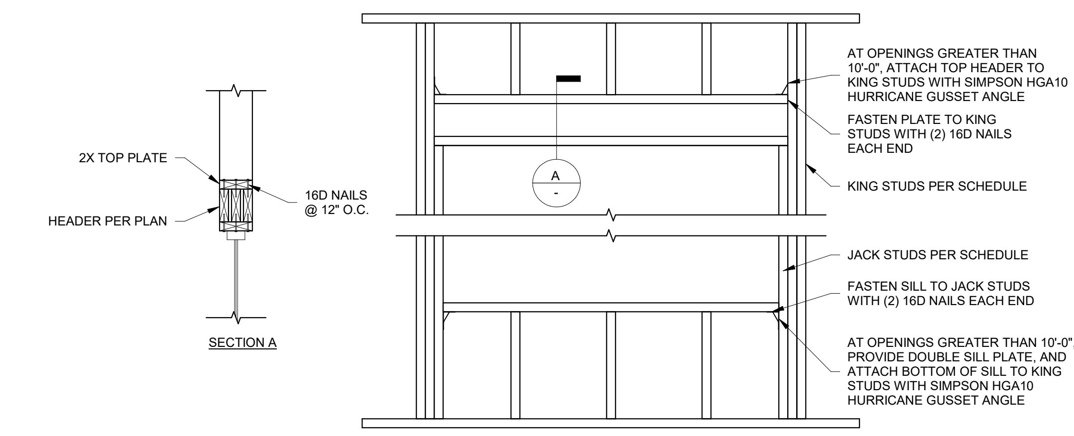
4 FRAMING AT OPENING 3/4" = 1'-0"
