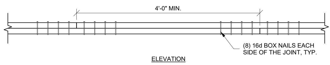
3 TOP PLATE SPLICE 1" = 1'-0"
