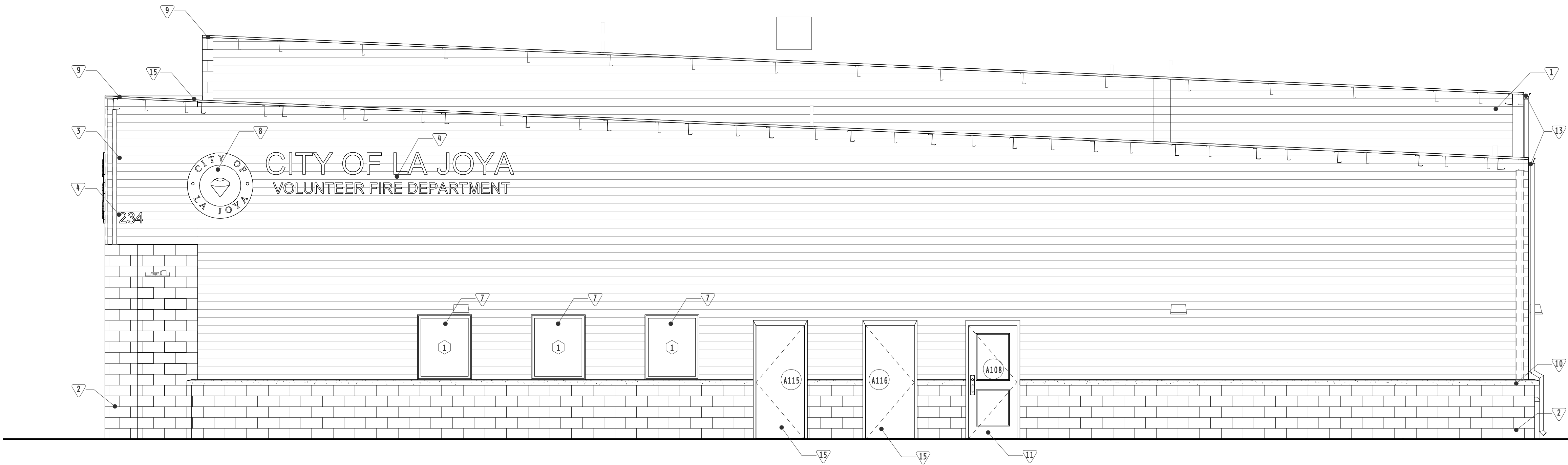
2 SOUTH ELEVATION 1/4" = 1'-0"
