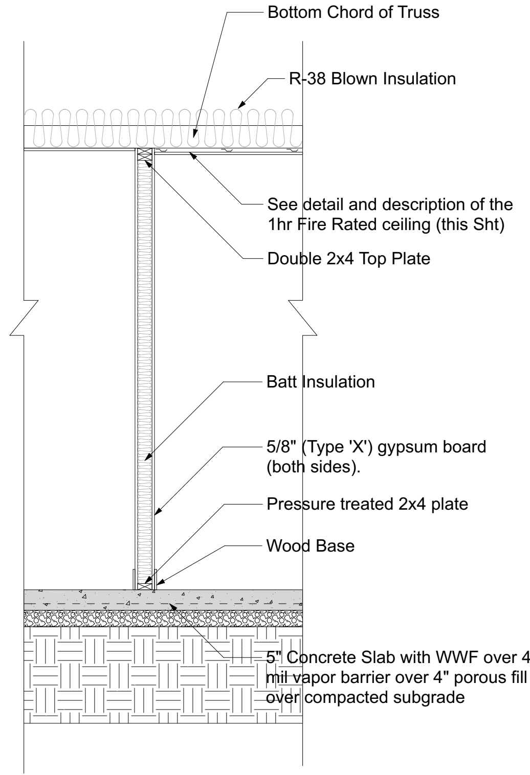
Section 2 Typical Interior Fire Rated Partition A5 UL Design U305 (See below)
