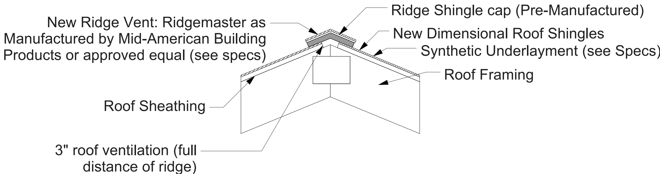
1 A4 Roof Detail 2 1 in = 1 ft
