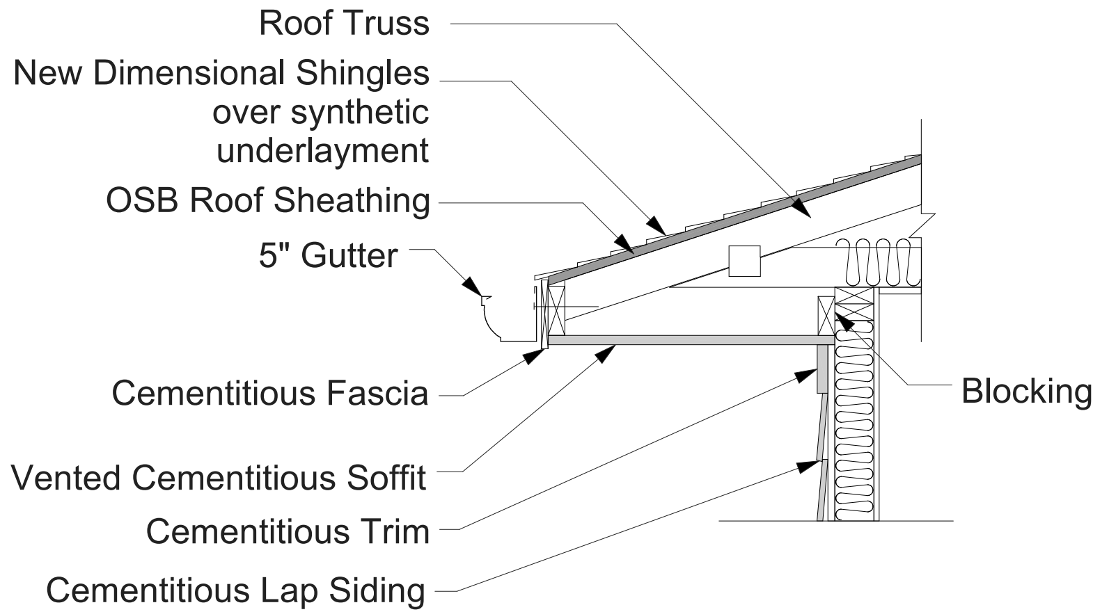
3 A4 Roof Eave Detail 1 in = 1 ft
