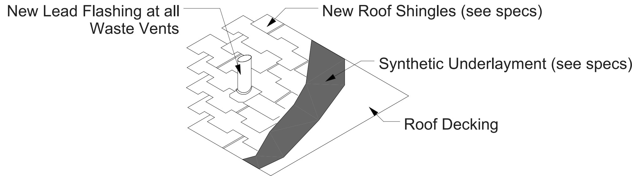
2 A4 Roof Detail 1 1 in = 1 ft
