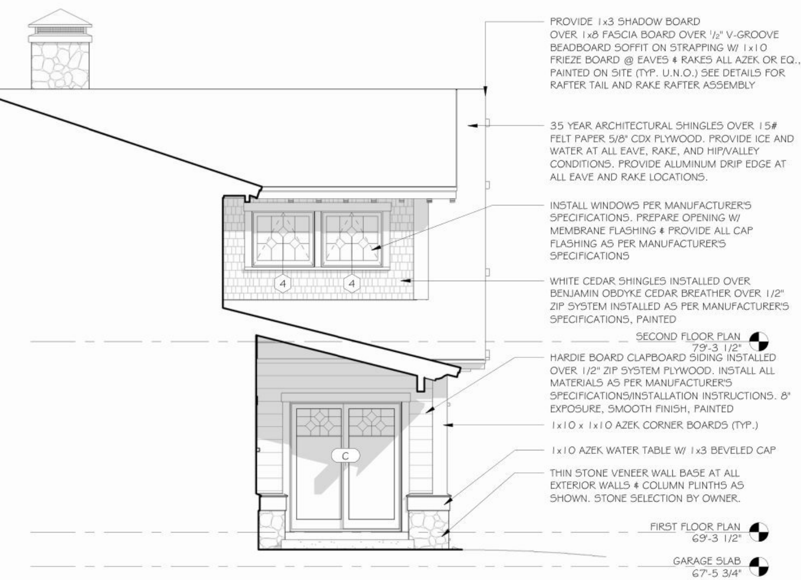
③ PARTIAL REAR ELEVATION 1/4" = 1'-0"
