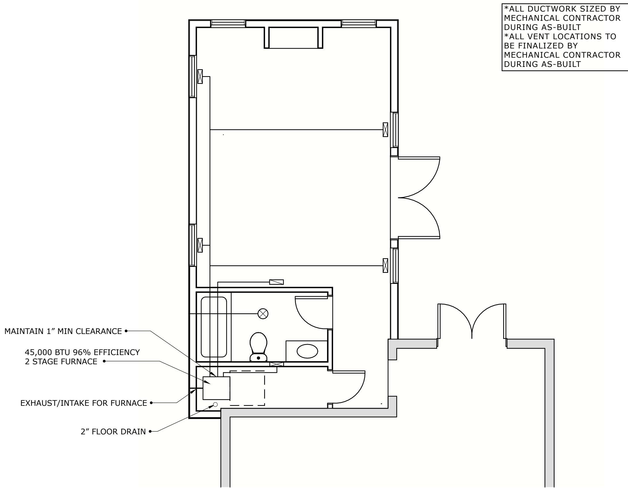
4 SECOND FLOOR MECHANICAL PLAN EM-10 SCALE: 1/4" = 1'-0"
