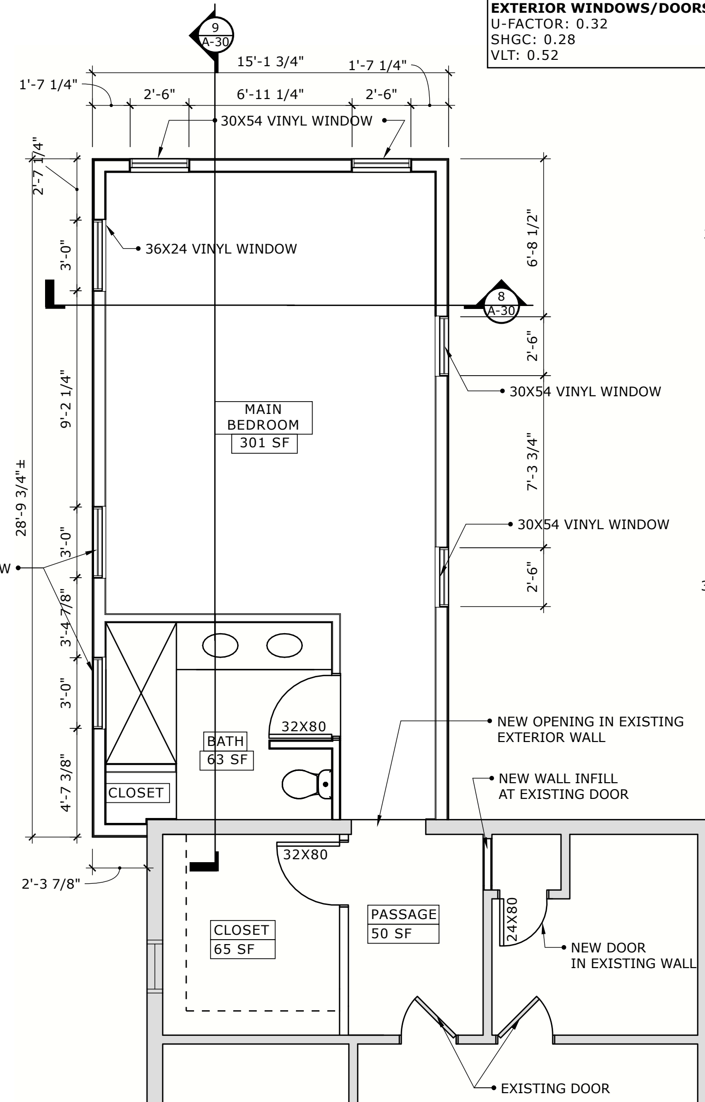
2 SECOND FLOOR PLAN A-10 SCALE: 1/4" = 1'-0"
