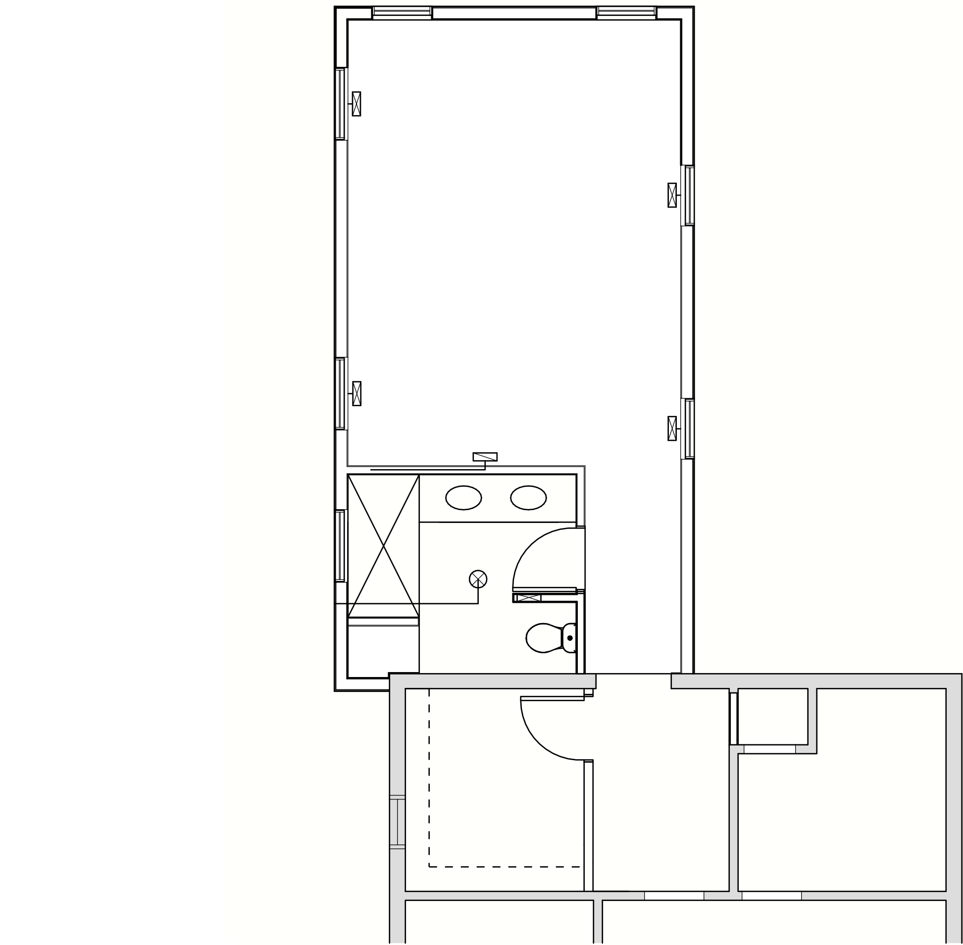
4 SECOND FLOOR MECHANICAL PLAN EM-10 SCALE: 1/4" = 1'-0"
