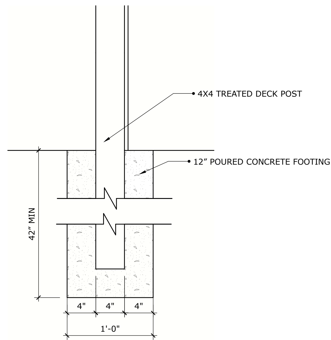
7 DECK POST FOOTING DETAIL A-00 SCALE: 1 1/2" = 1'-0"
