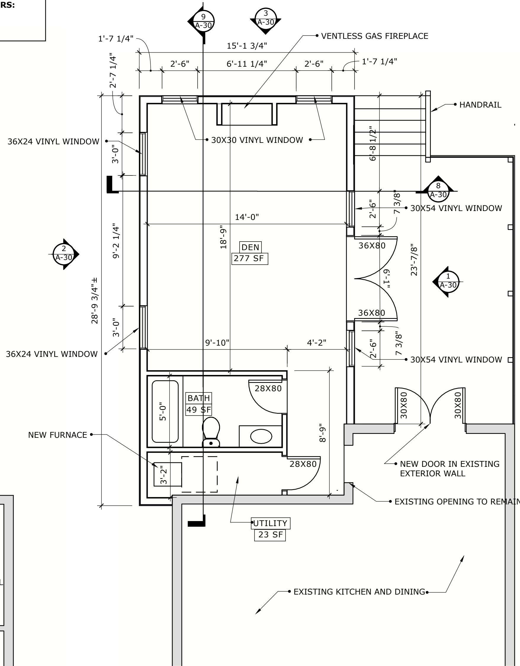
1 FIRST FLOOR PLAN A-10 SCALE: 1/4" = 1'-0"
