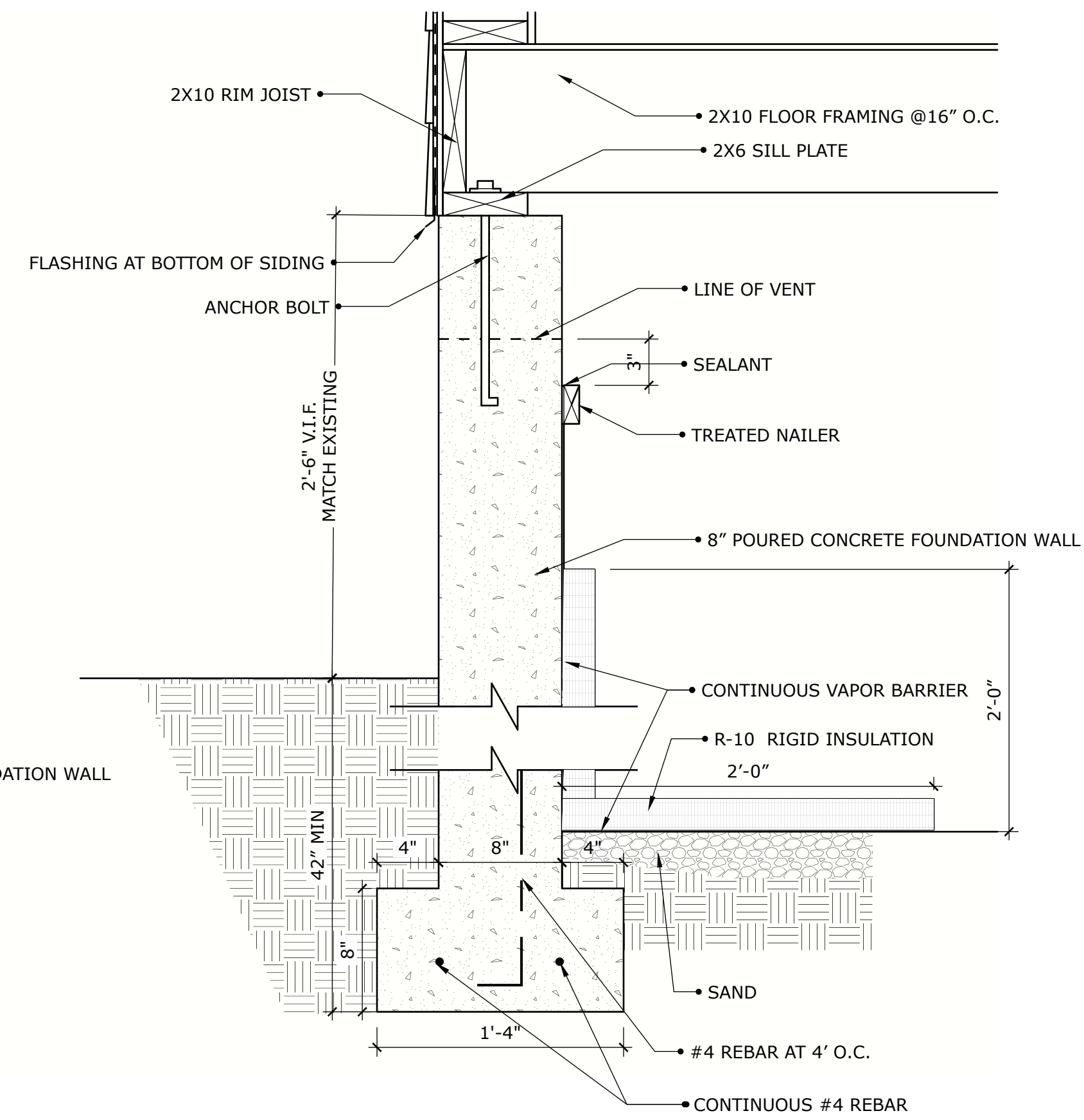
5 FOUNDATION DETAIL A-00 SCALE: 1 1/2" = 1'-0"
