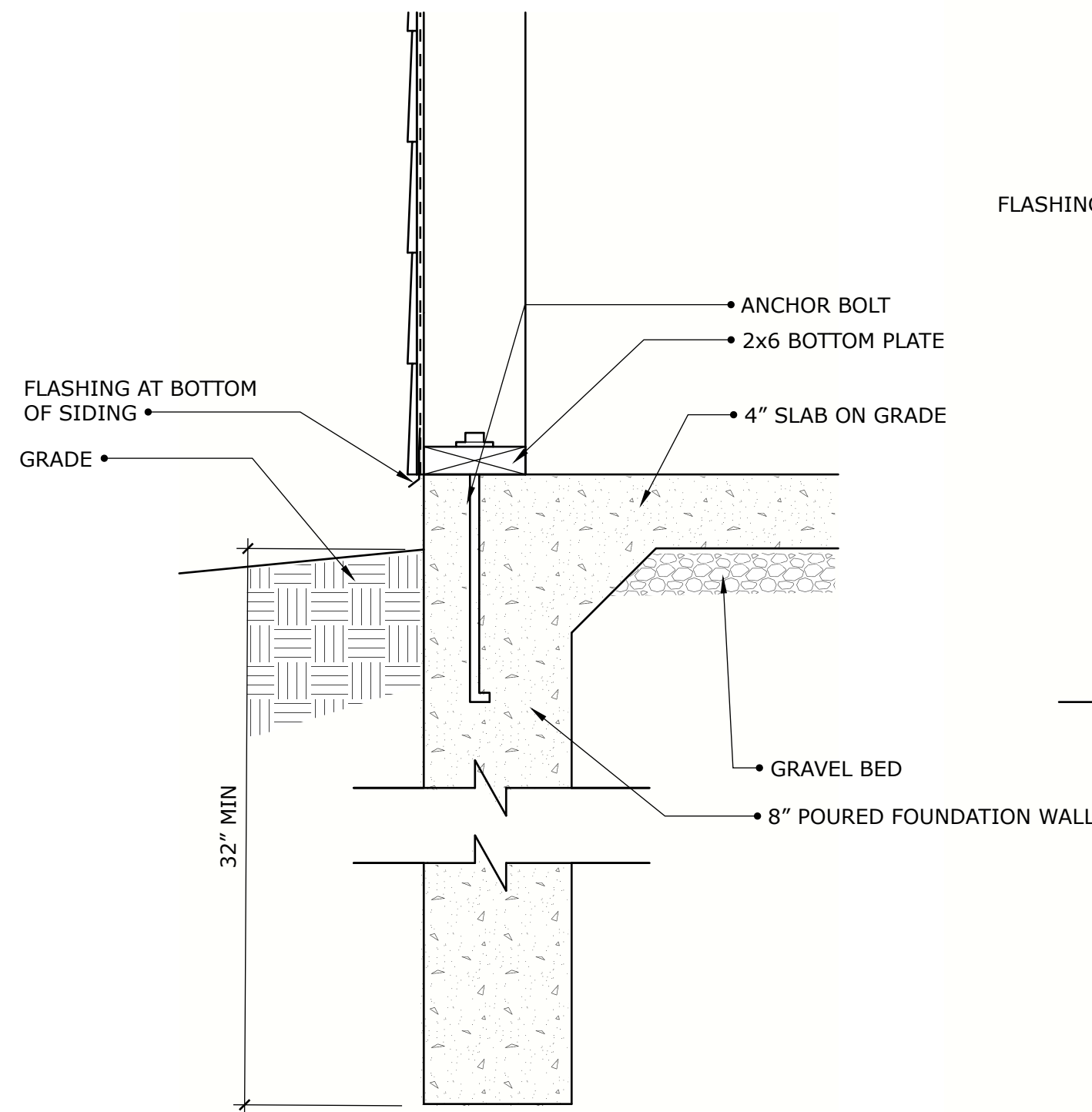
6 GARAGE FOUNDATION DETAIL A-00 SCALE: 1 1/2" = 1'-0"
