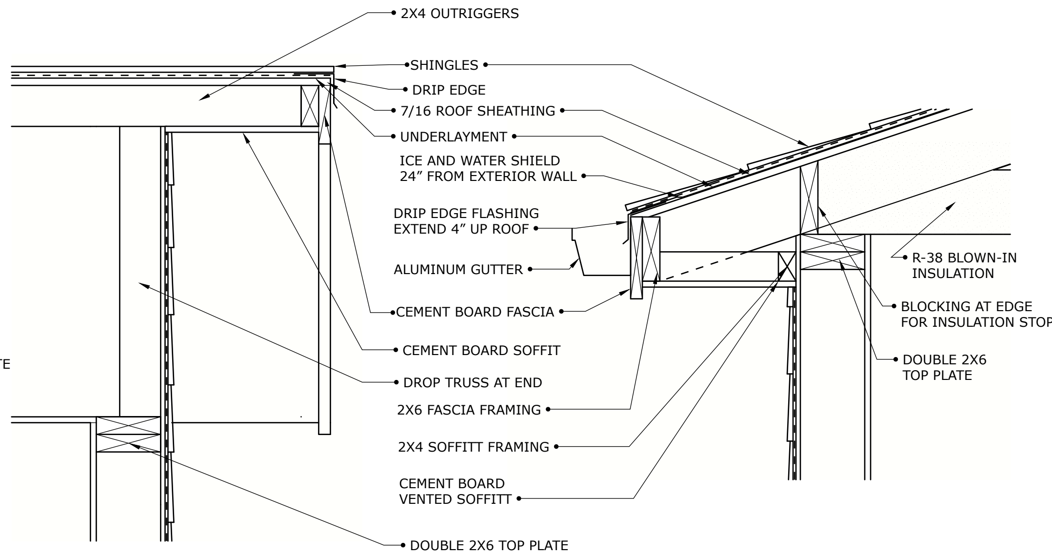
7 ADDITION ROOF EDGE DETAIL A-10 SCALE: 1 1/2" = 1'-0"
