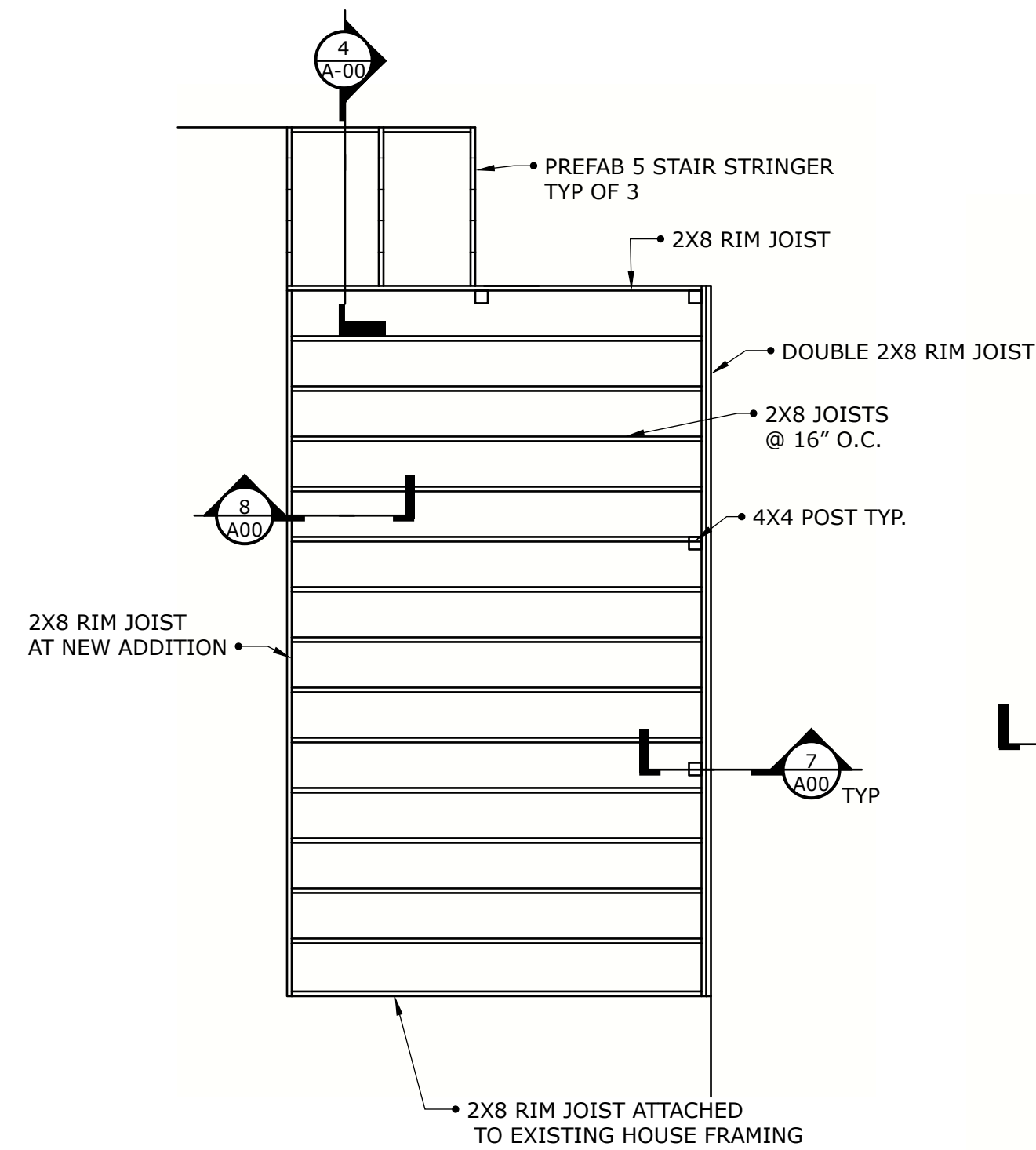
3 DECK FRAMING PLAN A-00 SCALE: 1/4" = 1'-0"
