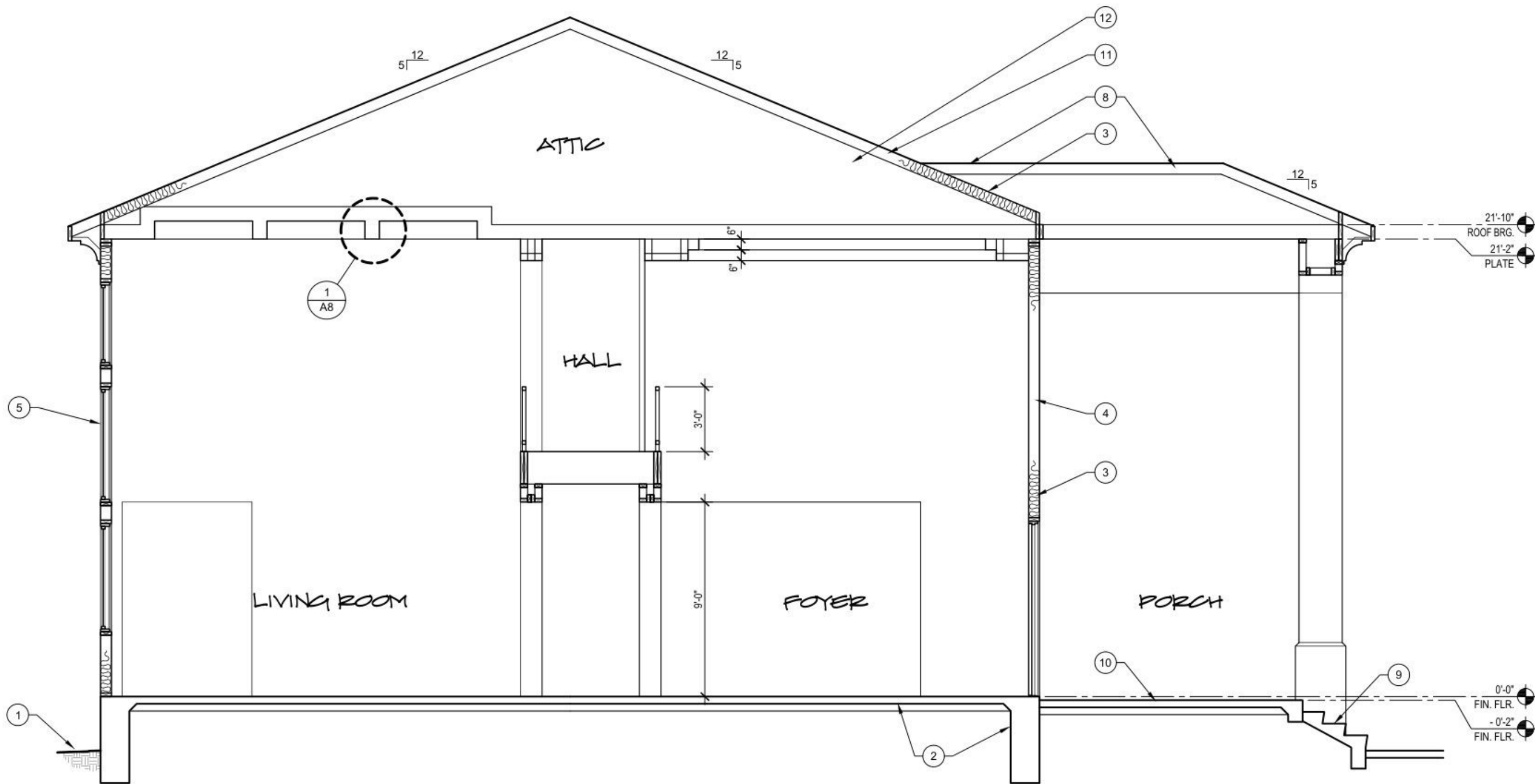
A BUILDING SECTION SCALE : 1/4" = 1'-0"
