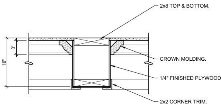
1 LIVING ROOM RECESSED TRIM SCALE : 1 1/2" = 1'-0"
