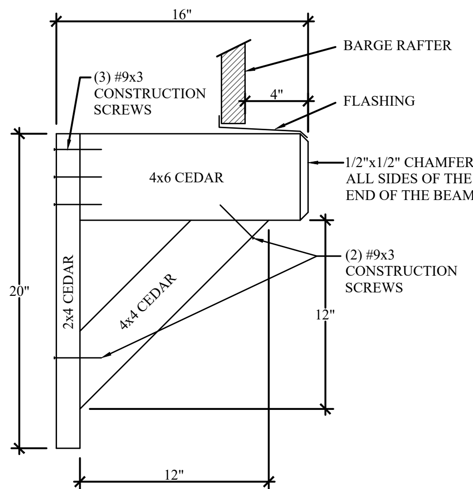
6 LOOKOUT BEAM SCALE: 2\"/>
