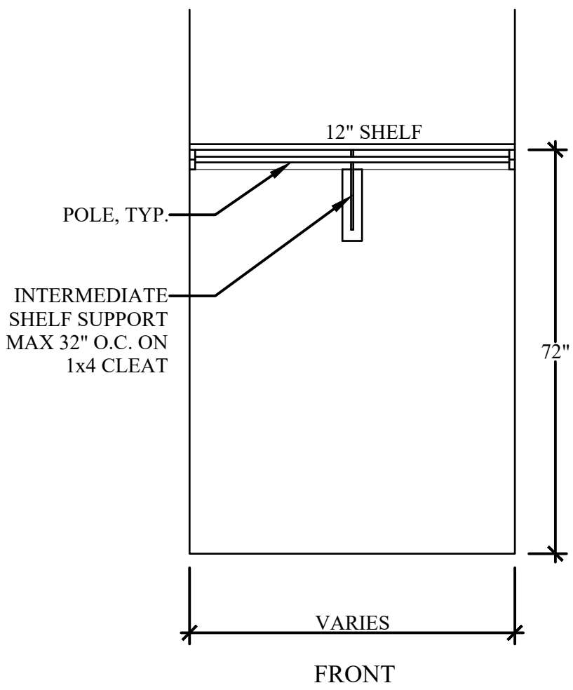
1a TYPICAL CLOSET SHELIVING SCALE: NTS
