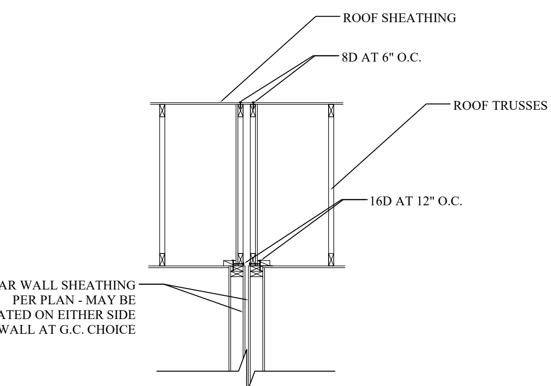
9 SHEAR TRANSFER AT TRUSSES SCALE: N.T.S.
