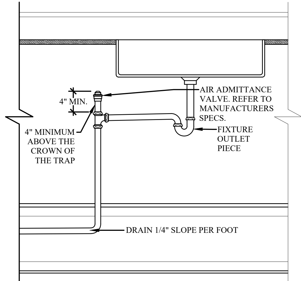
3 AIR ADMITTANCE VALVE DETAIL SCALE: 2 inch = 1'-0 inch
