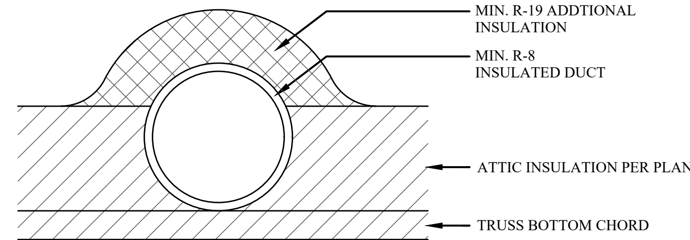
8 DEEPLY BURIED DUCT SCALE: 1\"/>
