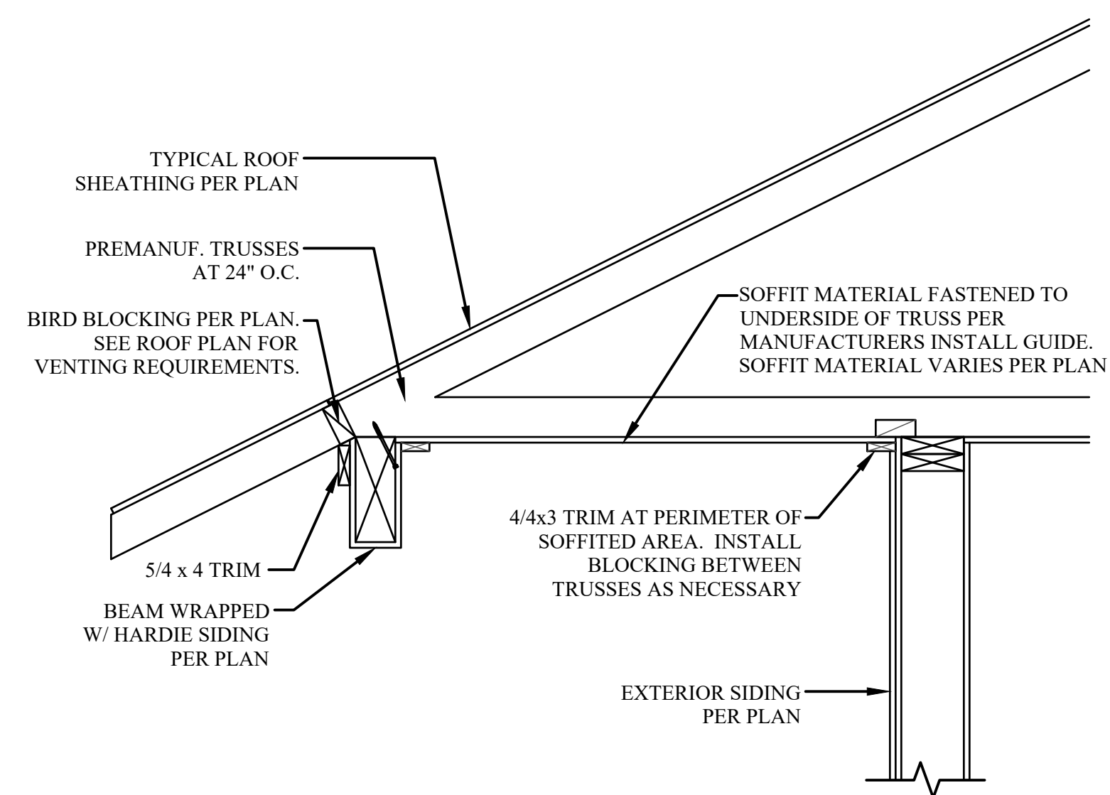
3 EXTERIOR SOFFIT ATTACHMENT SCALE: 1\"/>
