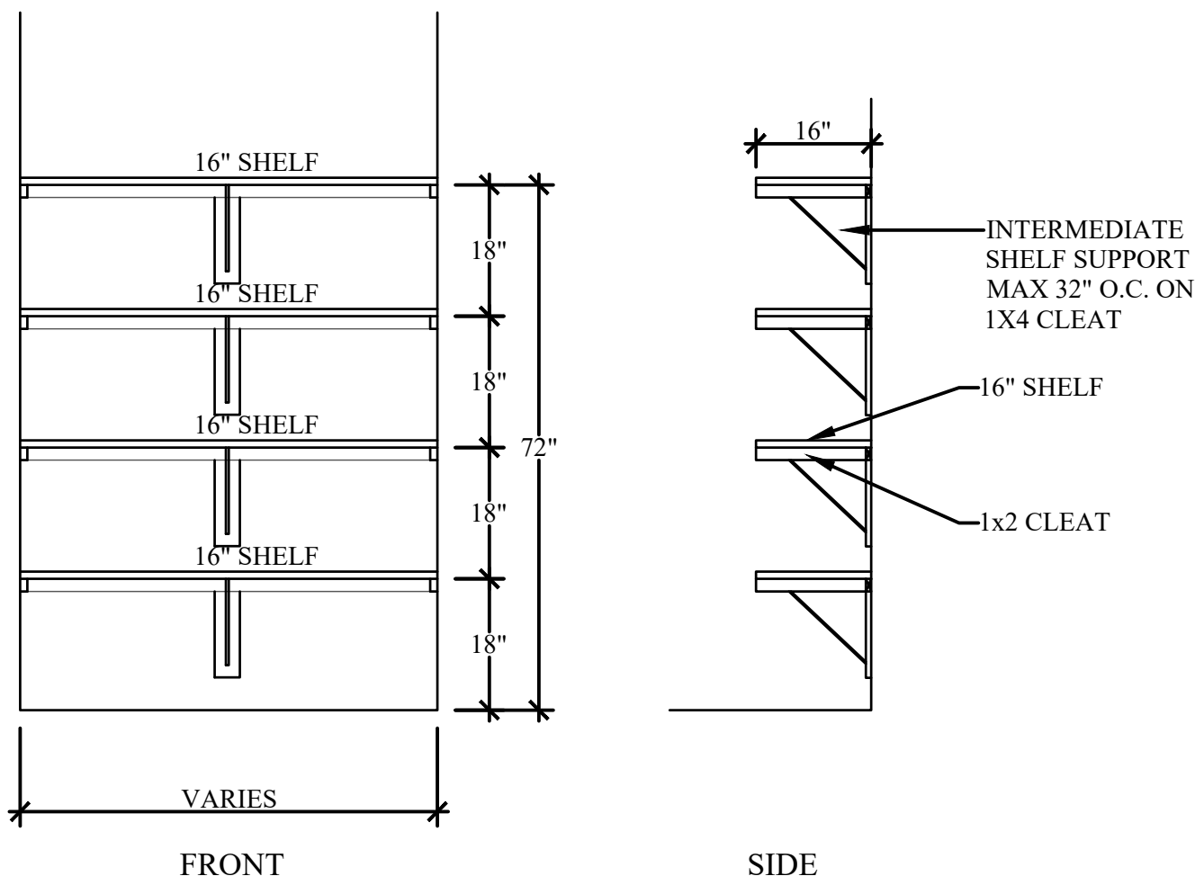
1b TYPICAL PANTRY/LINEN SHELIVING SCALE: NTS 4 SHELVES
