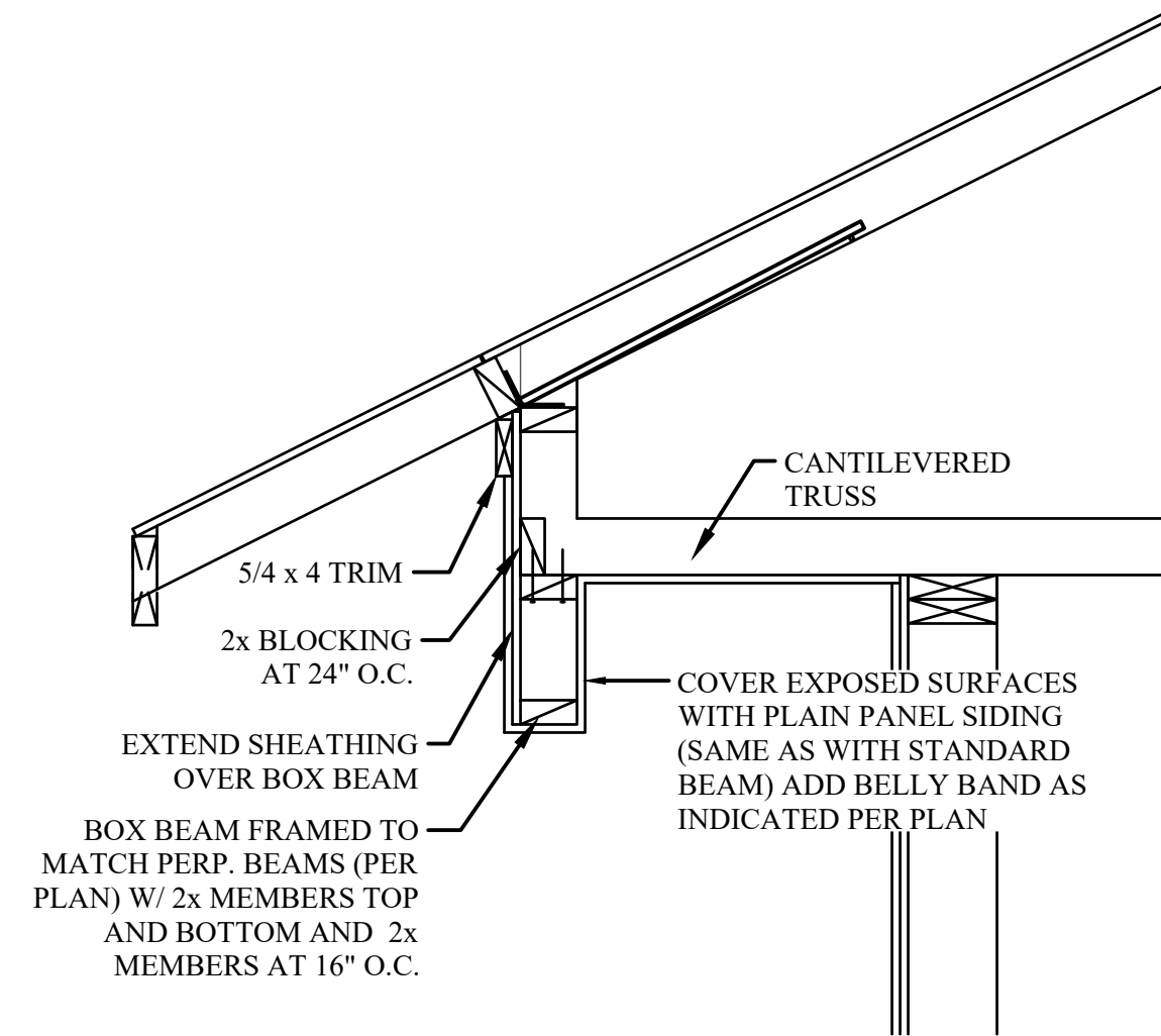
4 BOX BEAM DETAIL - EAVE SCALE: 1\"/>
