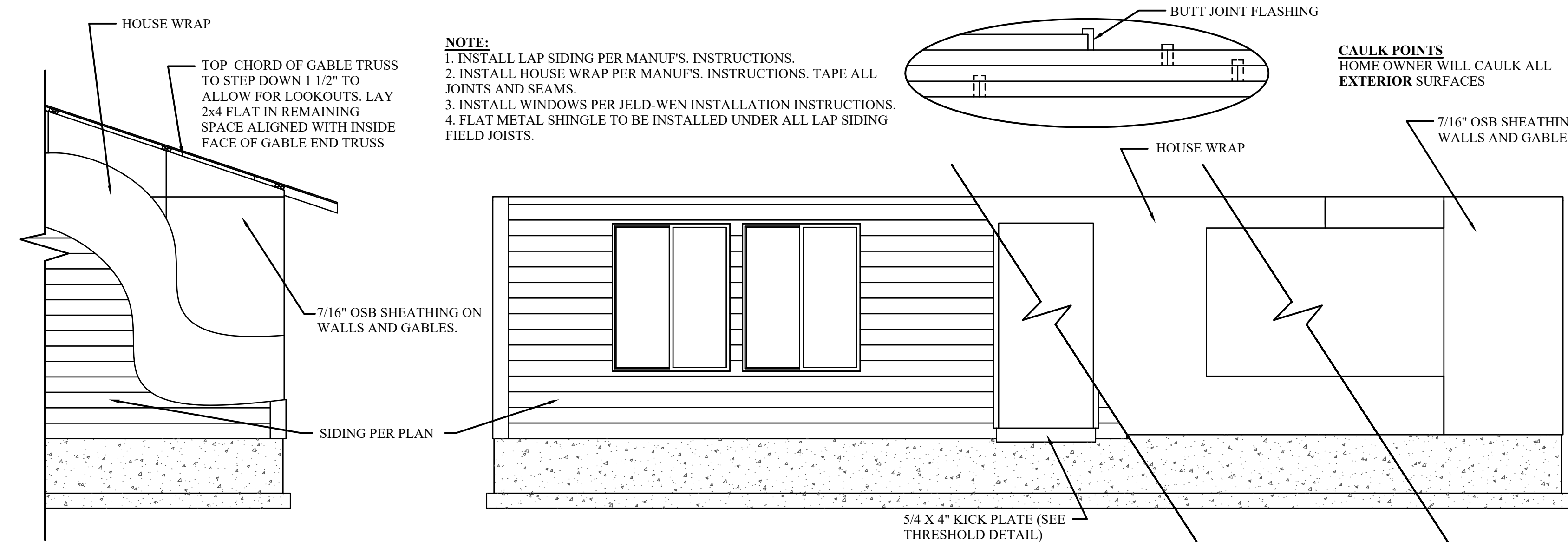
1 SIDING AND SHEATHING SCALE: NTS
