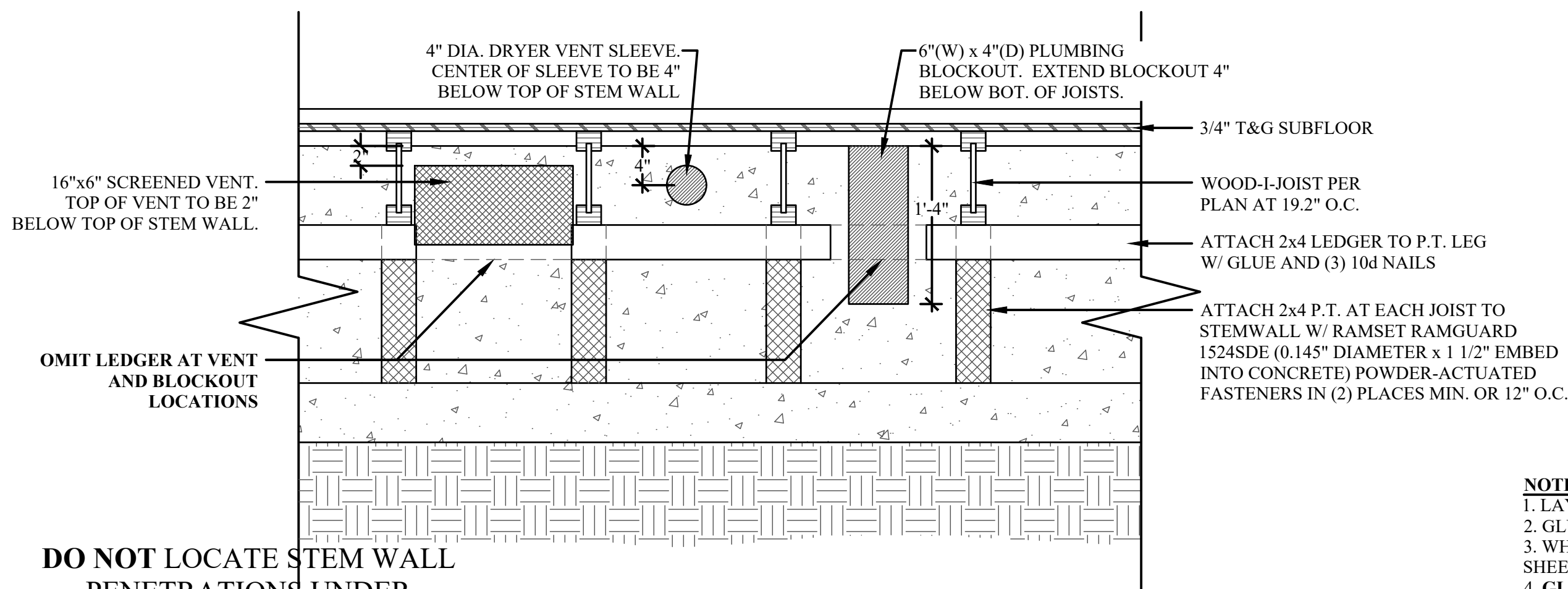
7 FOUNDATION VENTS & BLOCKOUTS SCALE: 1" = 1'-0"
