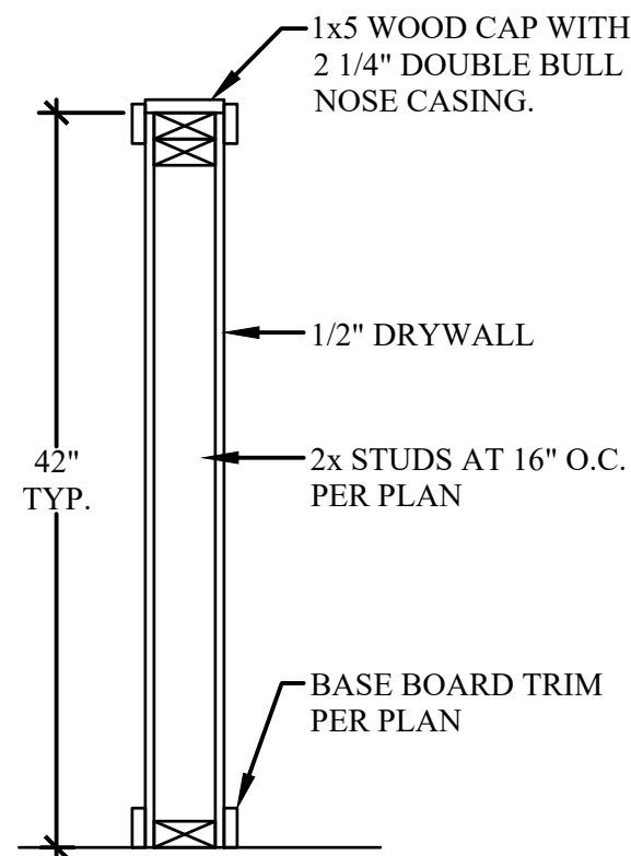
2 1/2 WALL WITH WOOD CAP SCALE: 1/2 inch = 1'-0 inch STANDARD MODERN OR CRAFTSMAN
