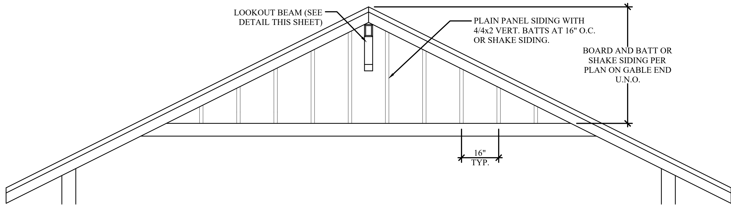
2 GABLE END DETAILING SCALE: NTS
