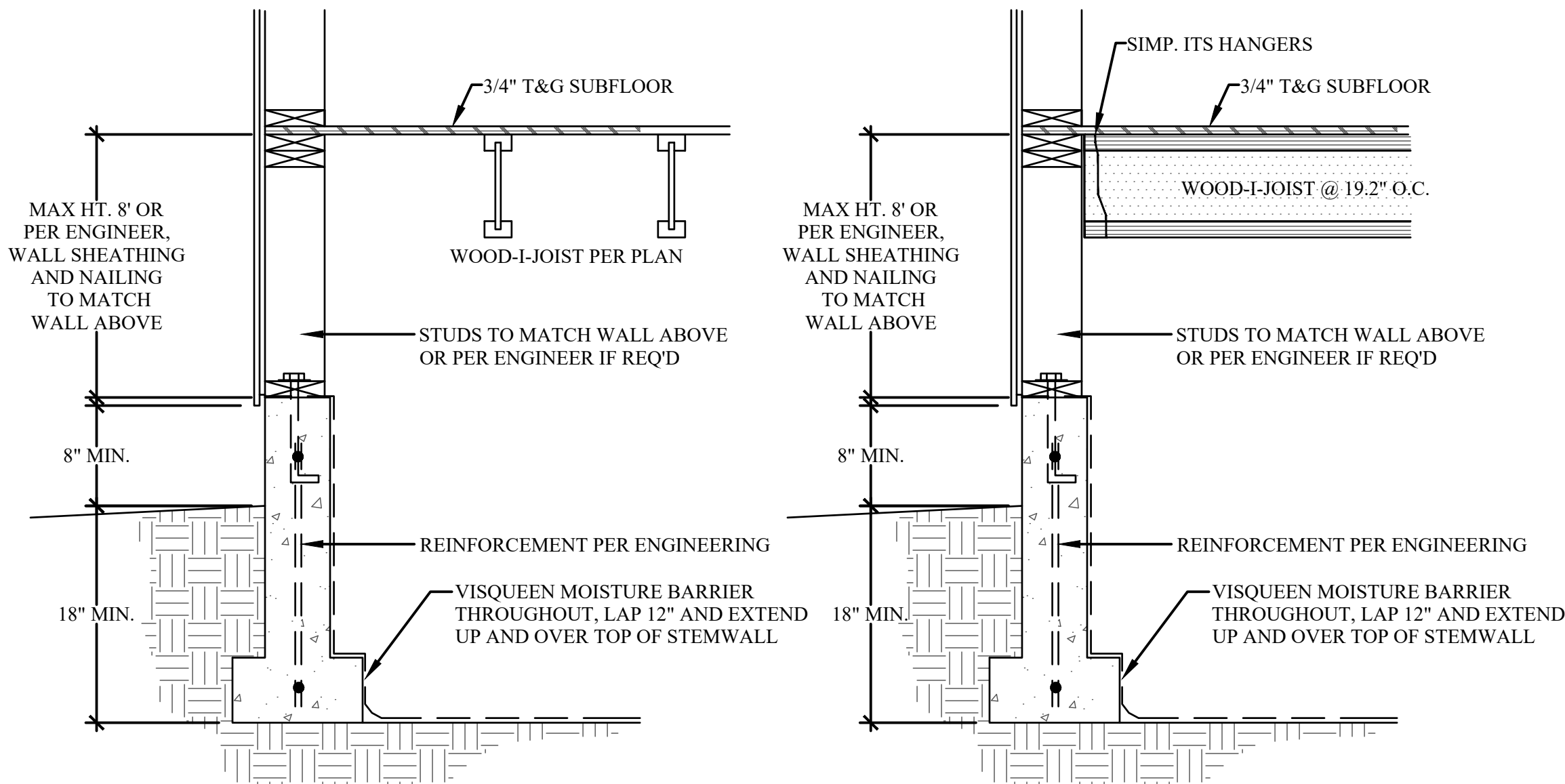
5a STEPPED FOUNDATION SCALE: 1/4" = 1'-0" PARALLEL JOISTS AS NEEDED
