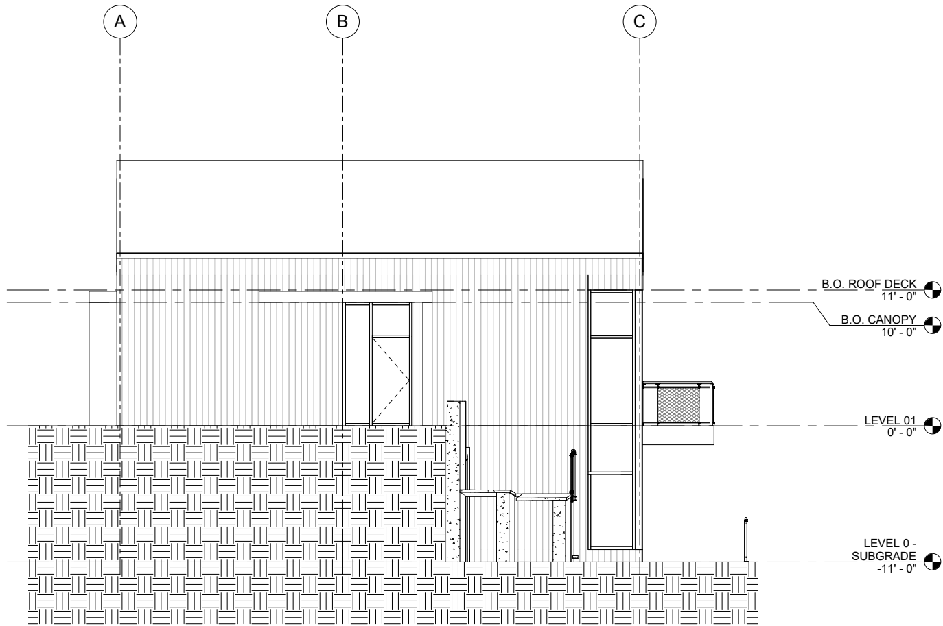
1 ELEVATION EAST 3/16" = 1'-0"
