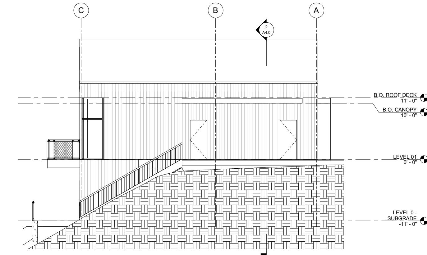
2 ELEVATION WEST 3/16" = 1'-0"
