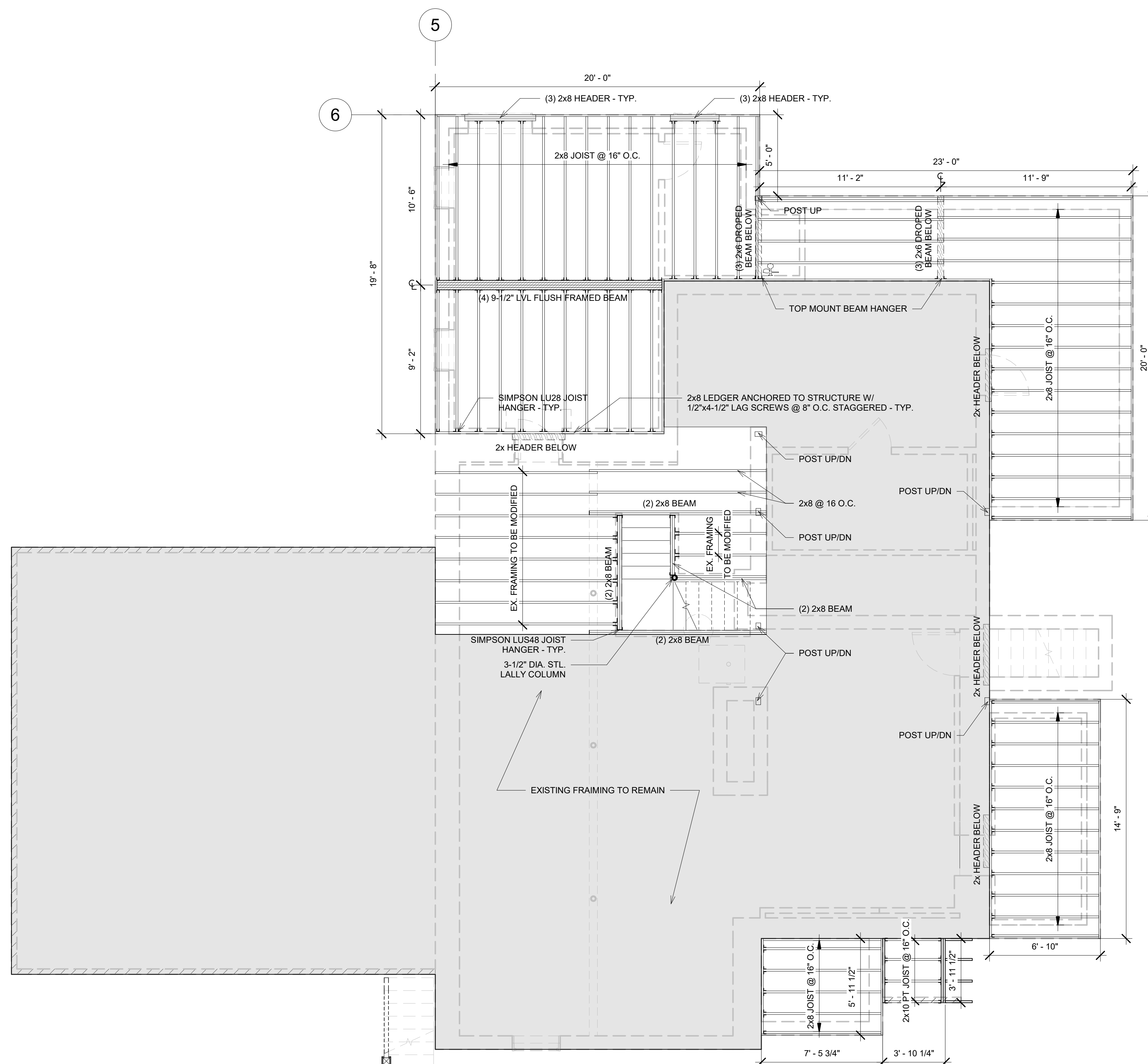
1 FIRST FLOOR FRAMING PLAN 1/4" = 1'-0"
