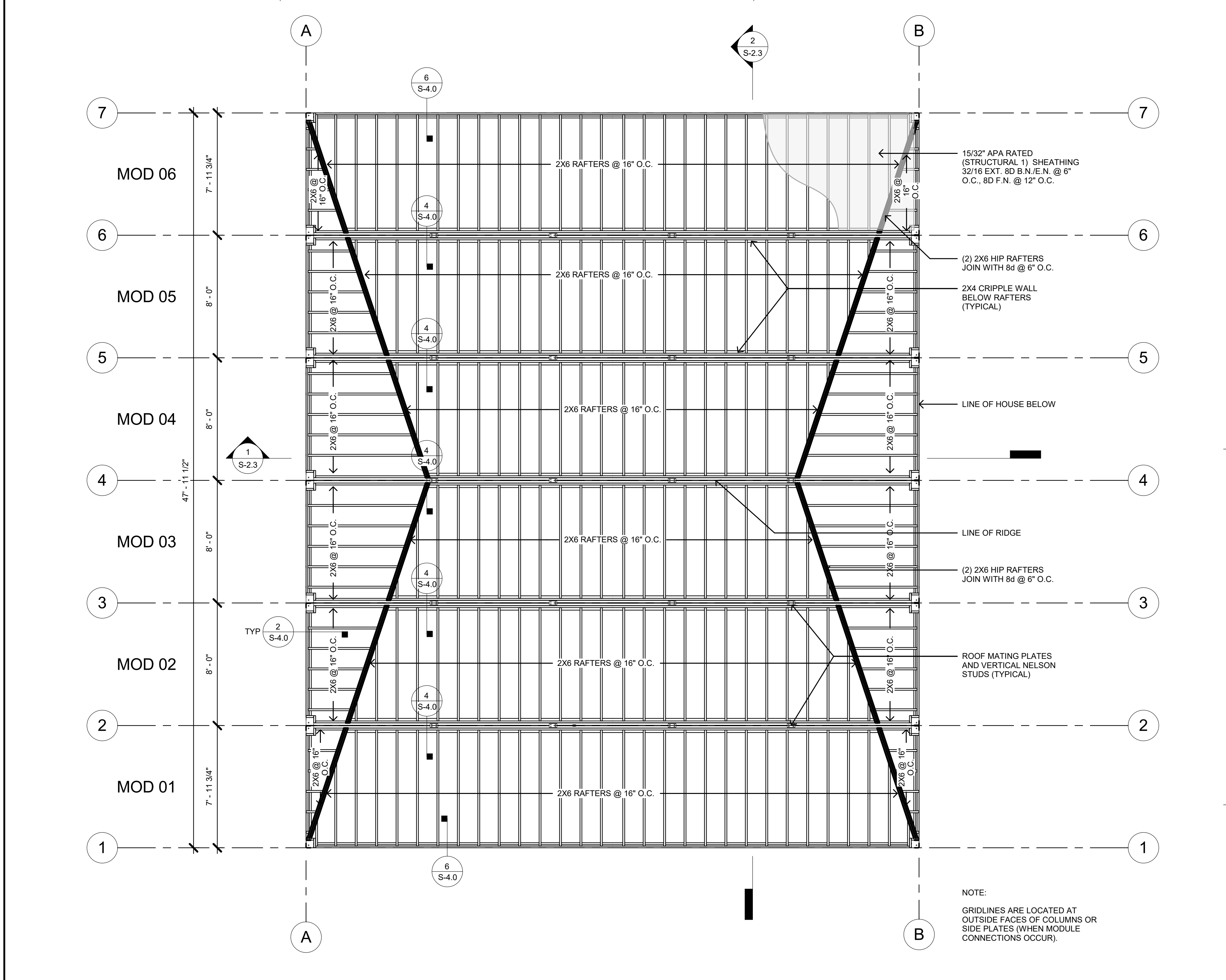
S - STRUCTURAL ROOF FRAMING PLAN - FACTORY BUILT 1/4" = 1'-0"
