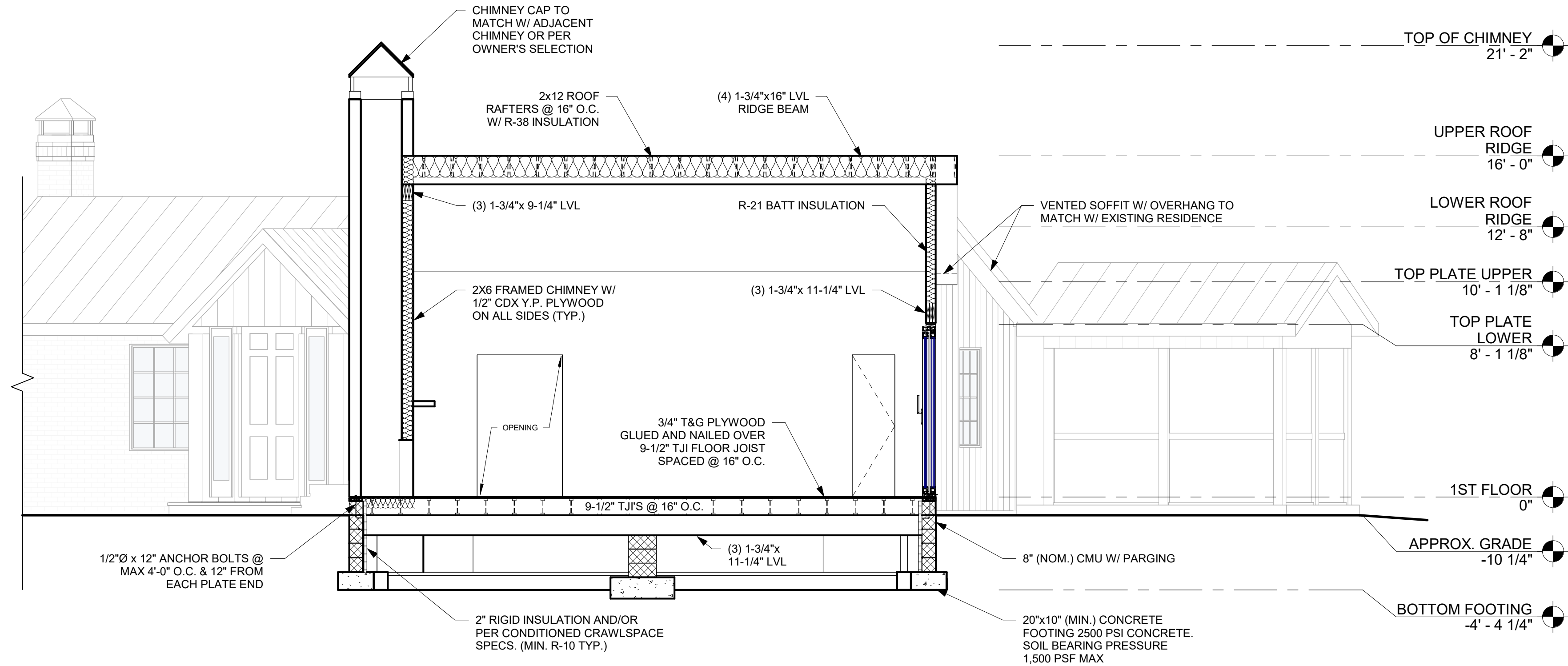
1 TRANVERSE SECTION @ GREAT ROOM ADDITION A5 SCALE:1/4" = 1'-0"
