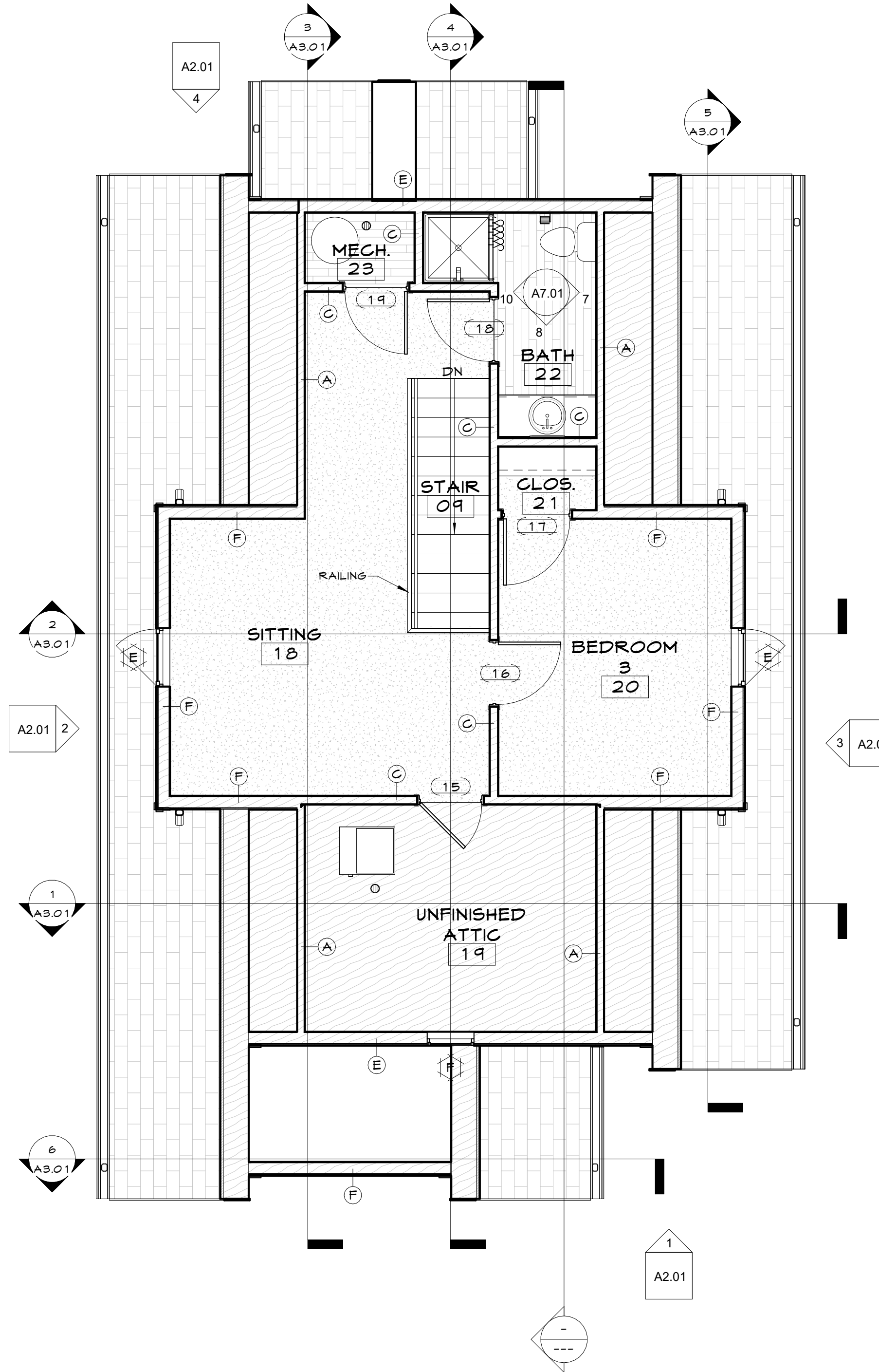
3 SECOND FLOOR REFERENCE PLAN A1.03 1/4" = 1'-0"
