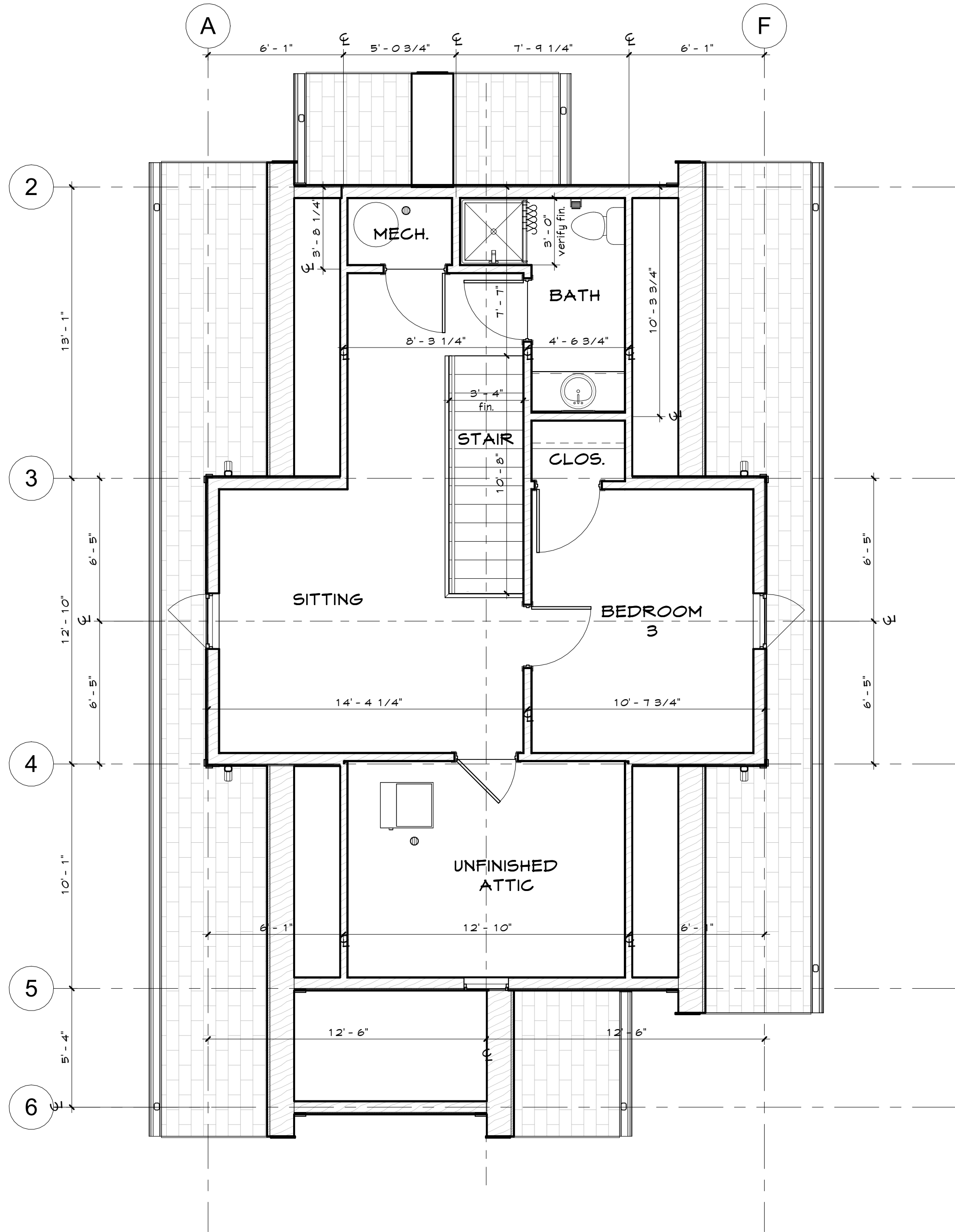
2 SECOND FLOOR DIMENSION PLAN A1.02 1/4" = 1'-0"
