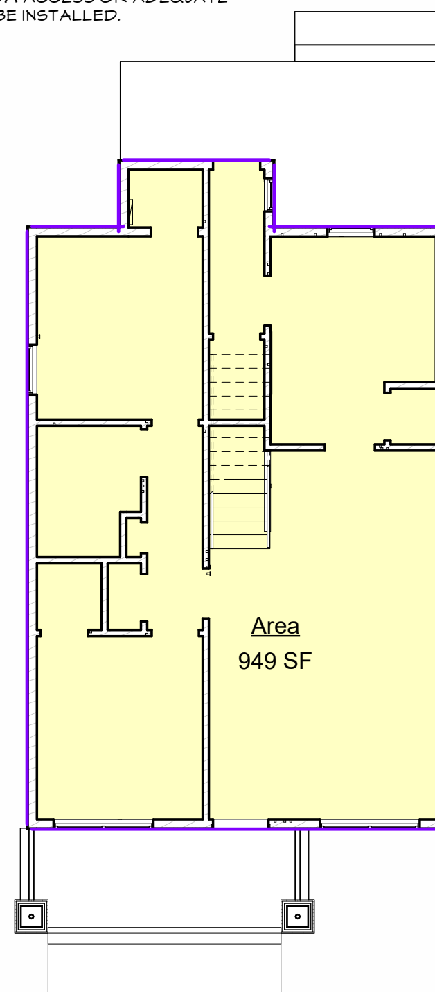
5 A2.01 FIRST FLOOR AREA 1/8" = 1'-0"
