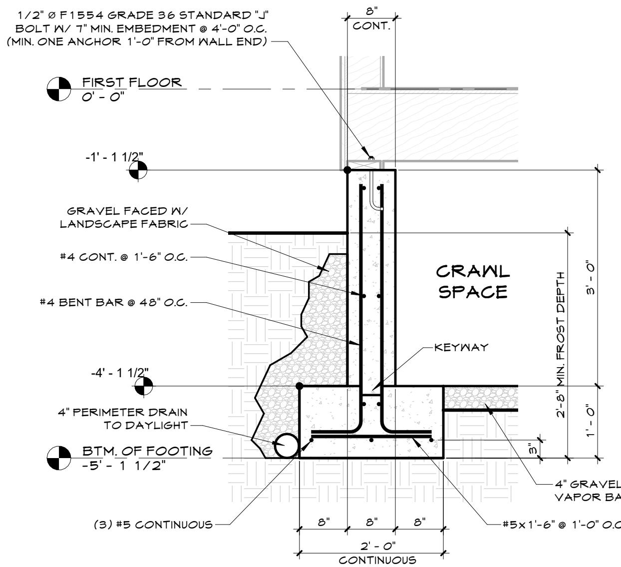
2 HOUSE FOOTING DETAIL 3/4" = 1'-0"
