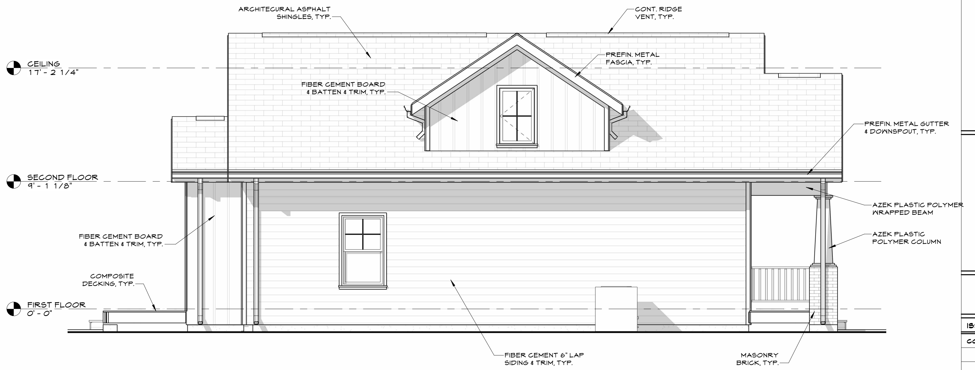
2 A2.01 LEFT SIDE ELEVATION 1/4" = 1'-0"
