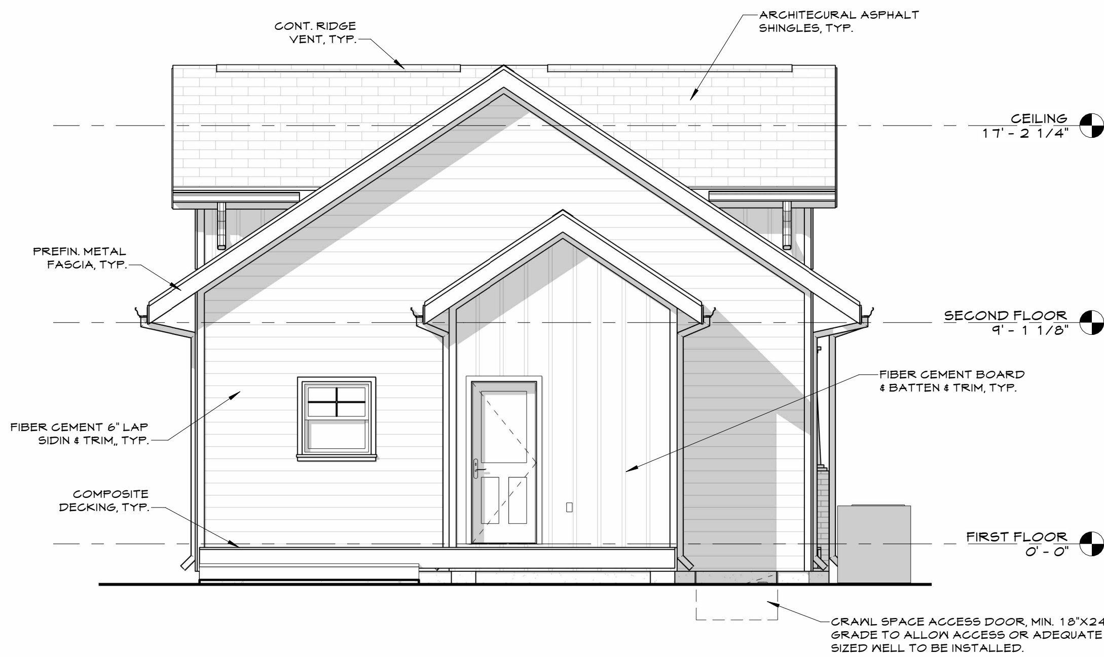
4 A2.01 BACK ELEVATION 1/4" = 1'-0"
