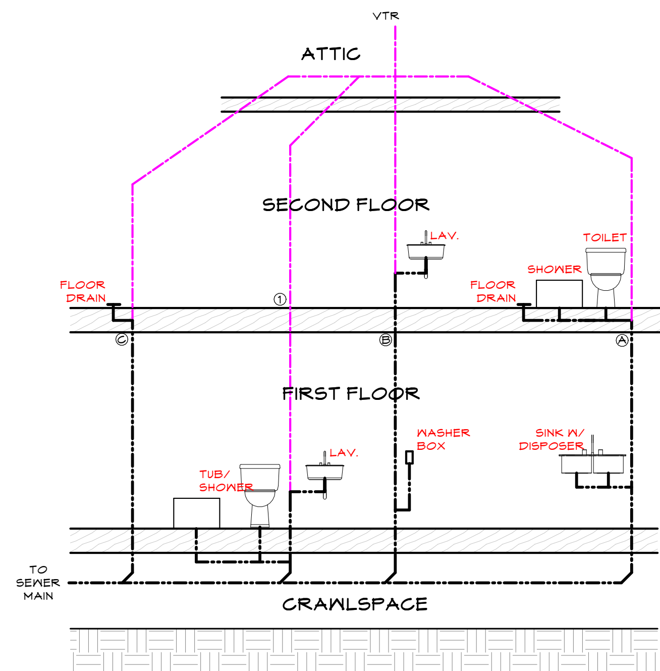
SCHEMATIC RISER DIAGRAM 1/4" = 1'-0"
