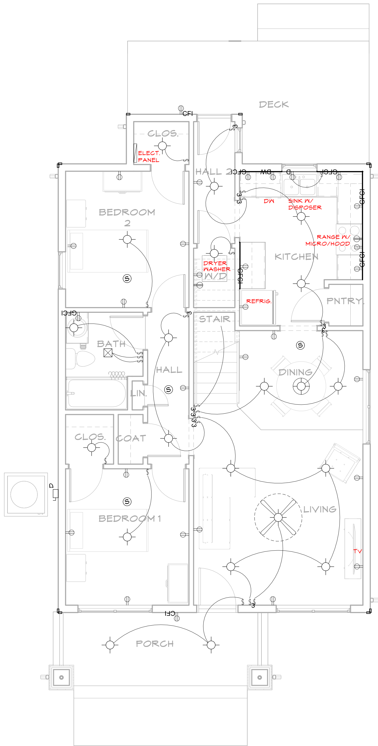
1 E1.01 ELECTRICAL PLAN - FIRST FLOOR 1/4" = 1'-0"
