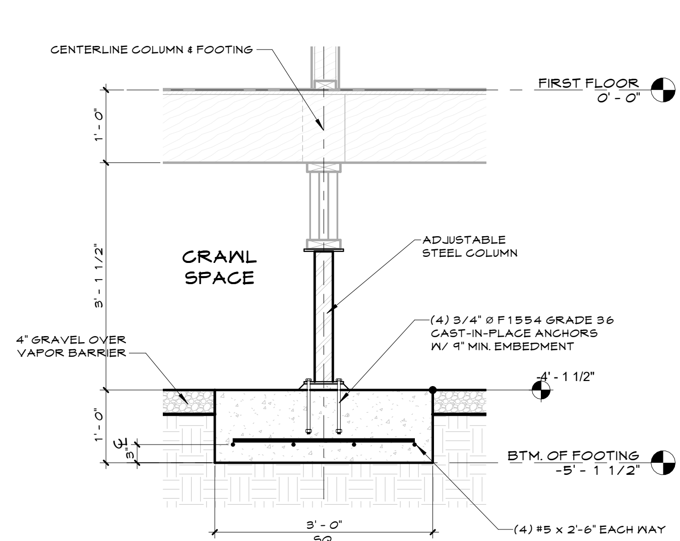
3 CRAWLSPACE COLUMN FOOTING DETAIL 3/4" = 1'-0"
