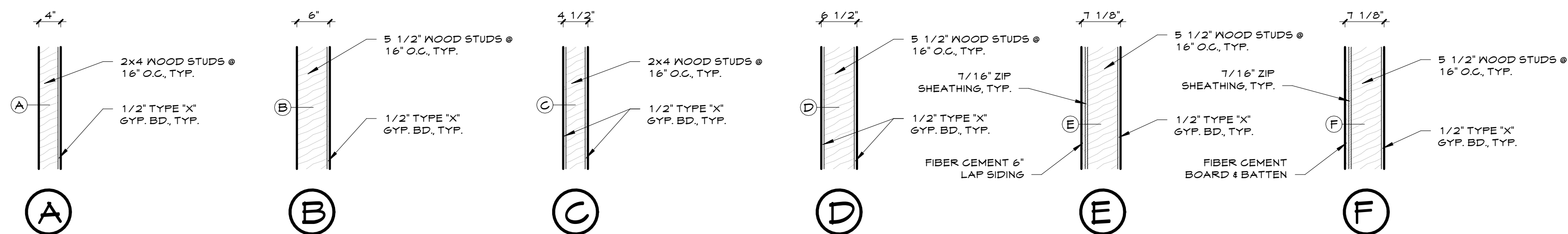
2 WALL TYPES A1.03 3/4" = 1'-0"
