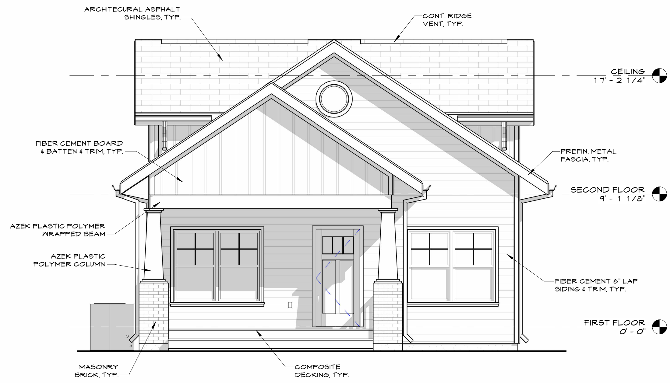
1 A2.01 FRONT ELEVATION 1/4" = 1'-0"
