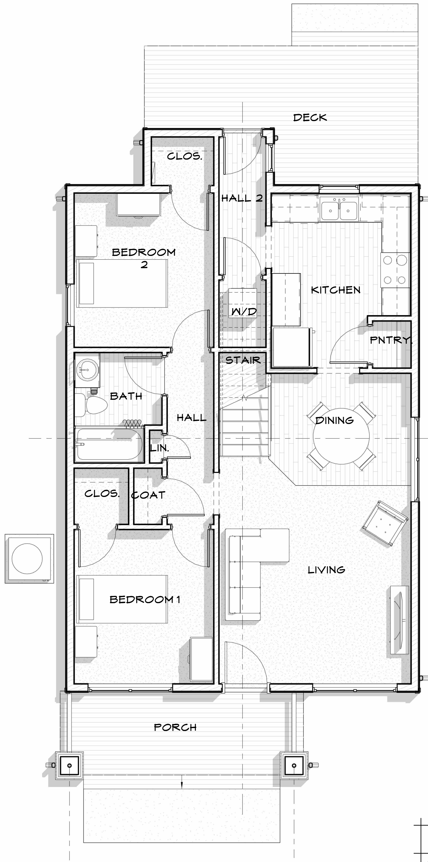
1 FIRST FLOOR PLAN A1.01 1/4" = 1'-0"
