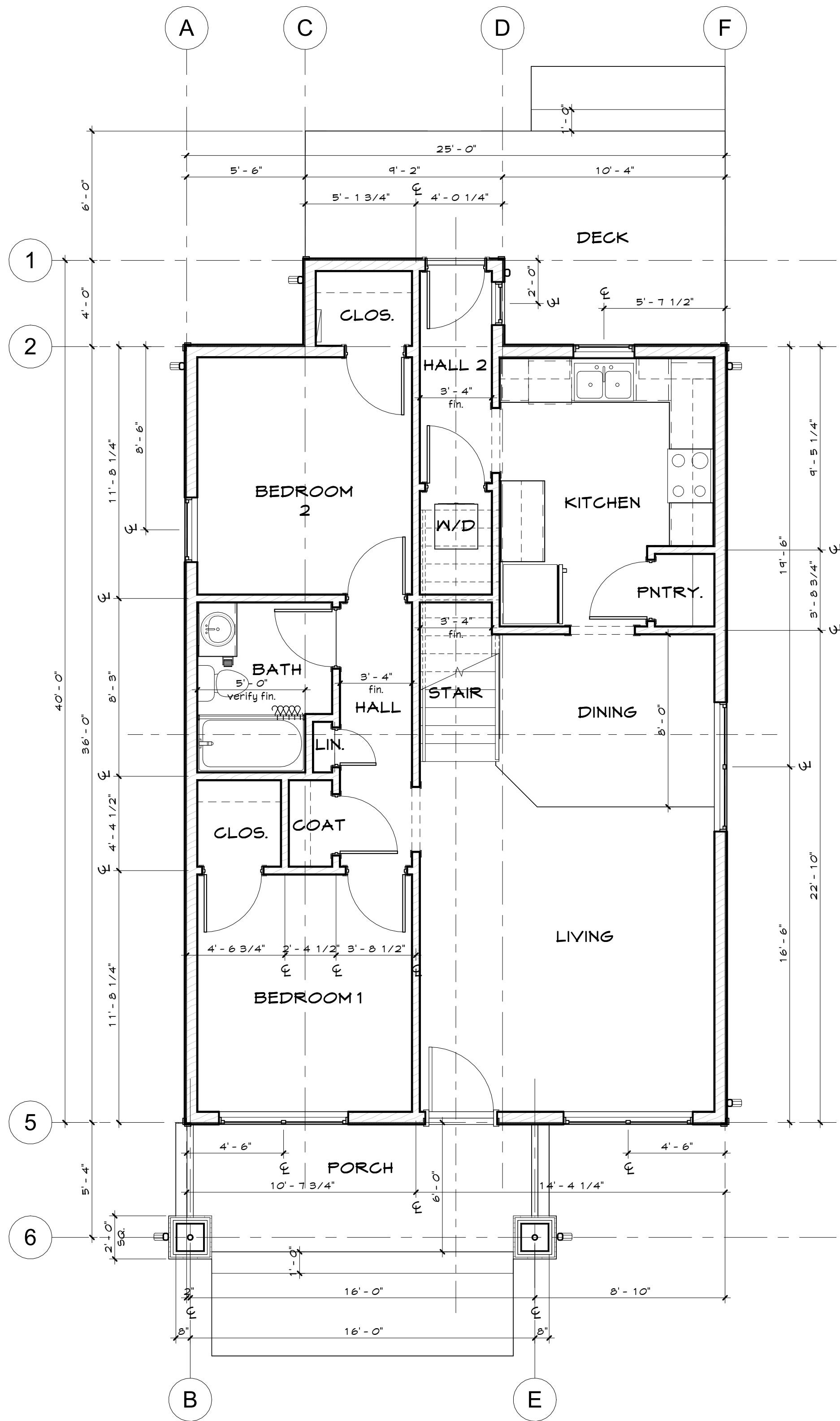
1 FIRST FLOOR DIMENSION PLAN A1.02 1/4" = 1'-0"
