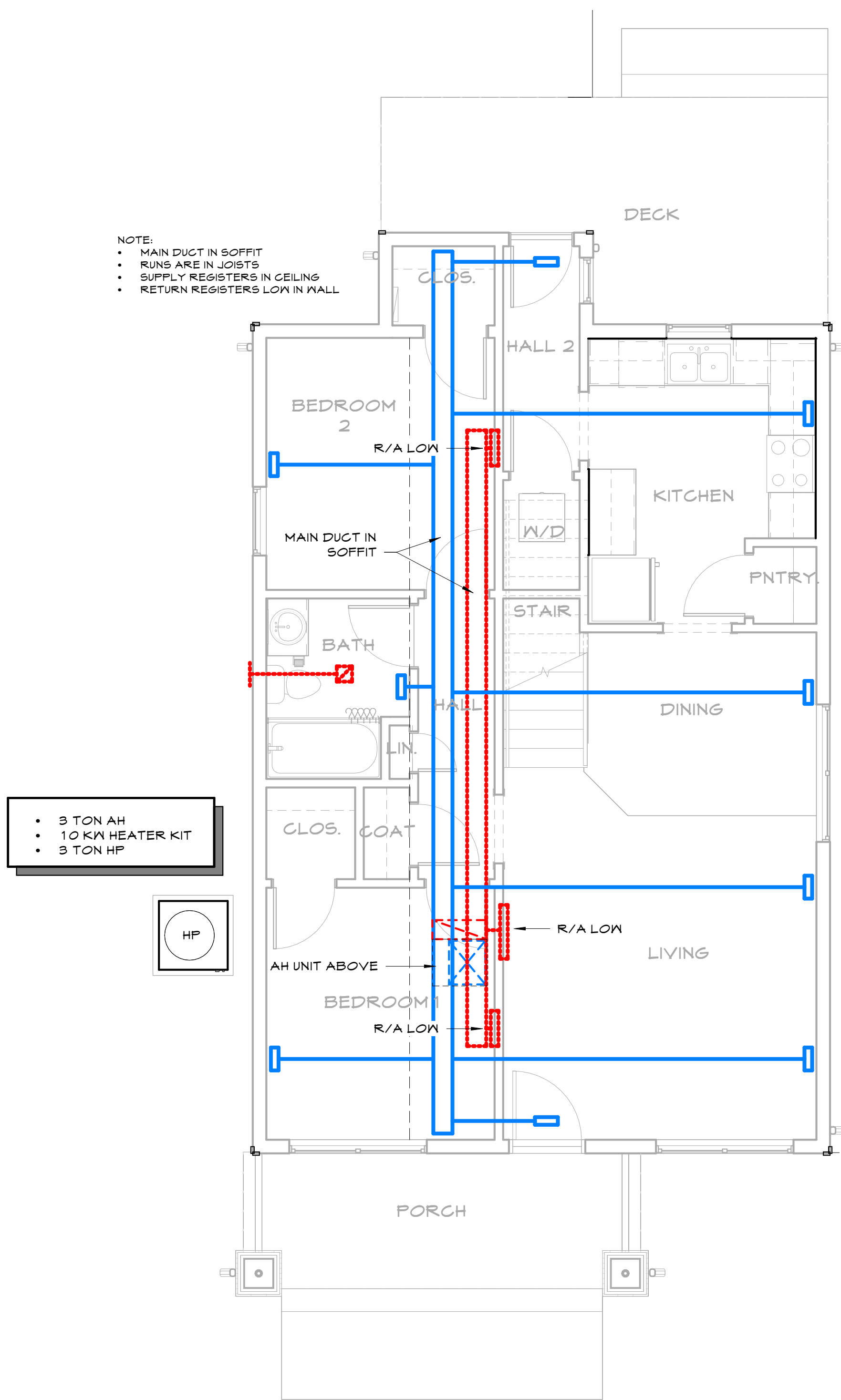
1 HVAC PLAN - FIRST FLOOR M1.01 1/4" = 1'-0"
