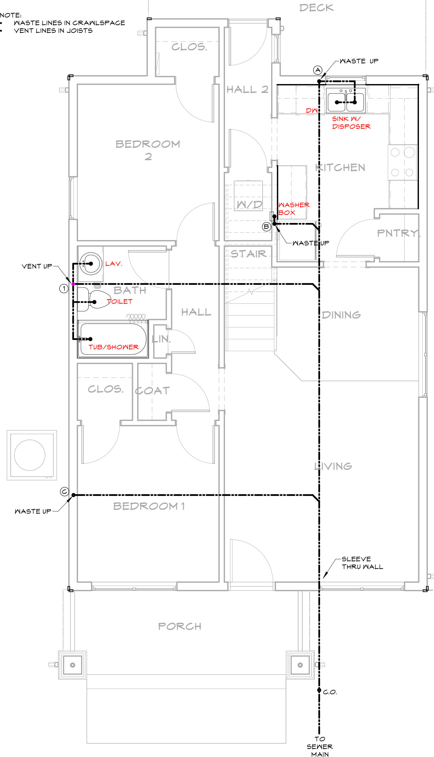
1 P.1.02 SEWER PLAN - FIRST FLOOR 1/4" = 1'-0"
