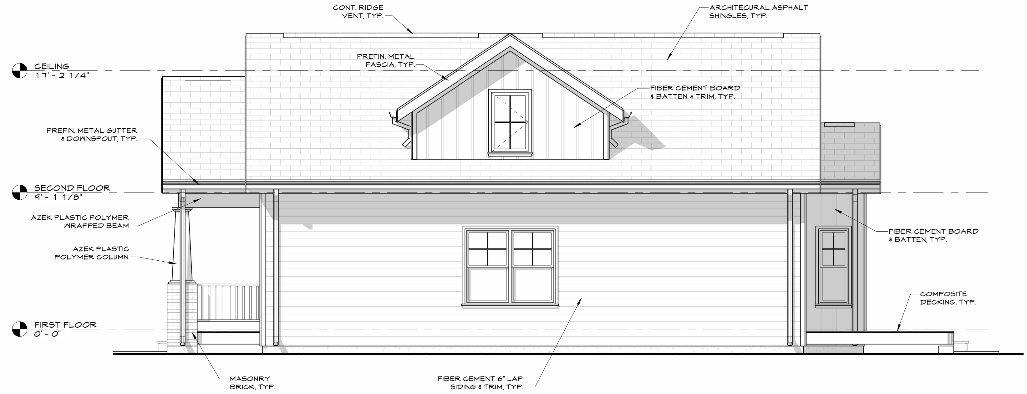
3 A2.01 RIGHT SIDE ELEVATION 1/4" = 1'-0"
