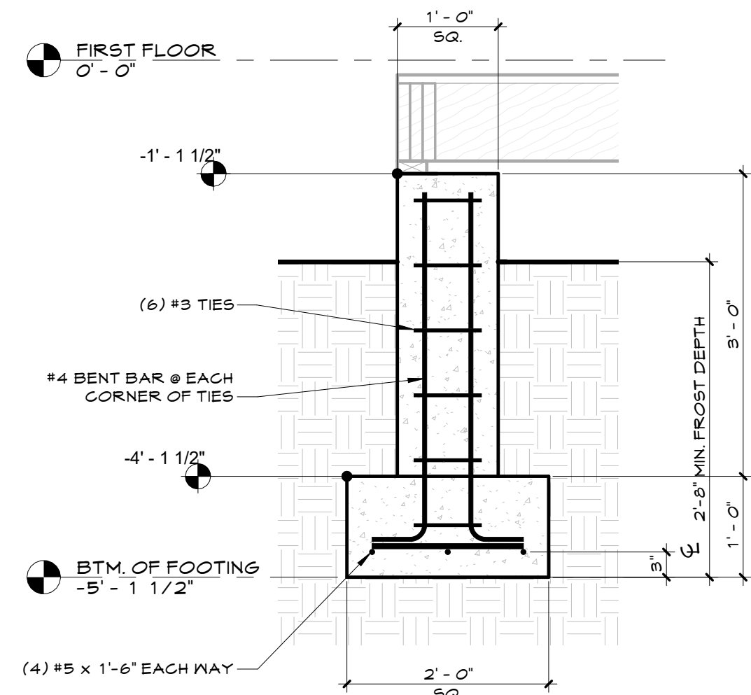
5 DECK COLUMN FOOTING DETAIL 3/4" = 1'-0"
