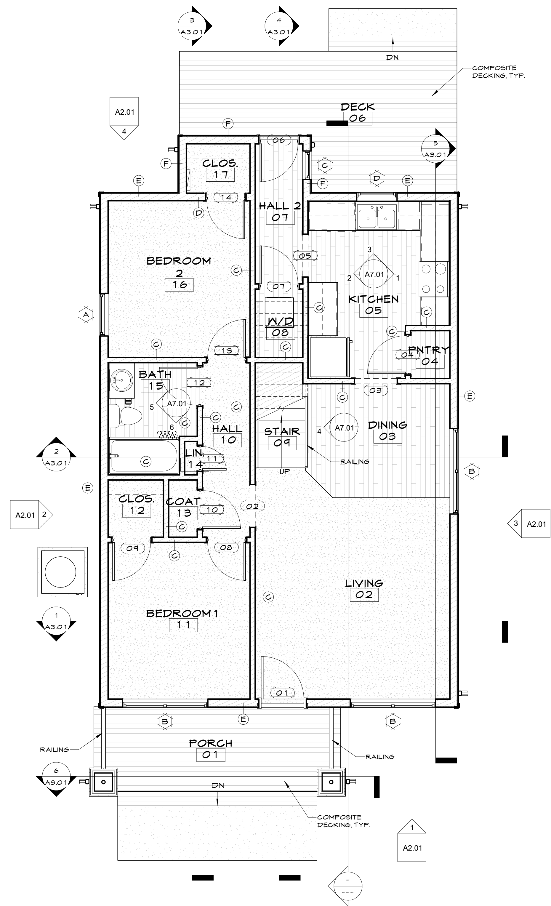
1 FIRST FLOOR REFERENCE PLAN A1.03 1/4" = 1'-0"
