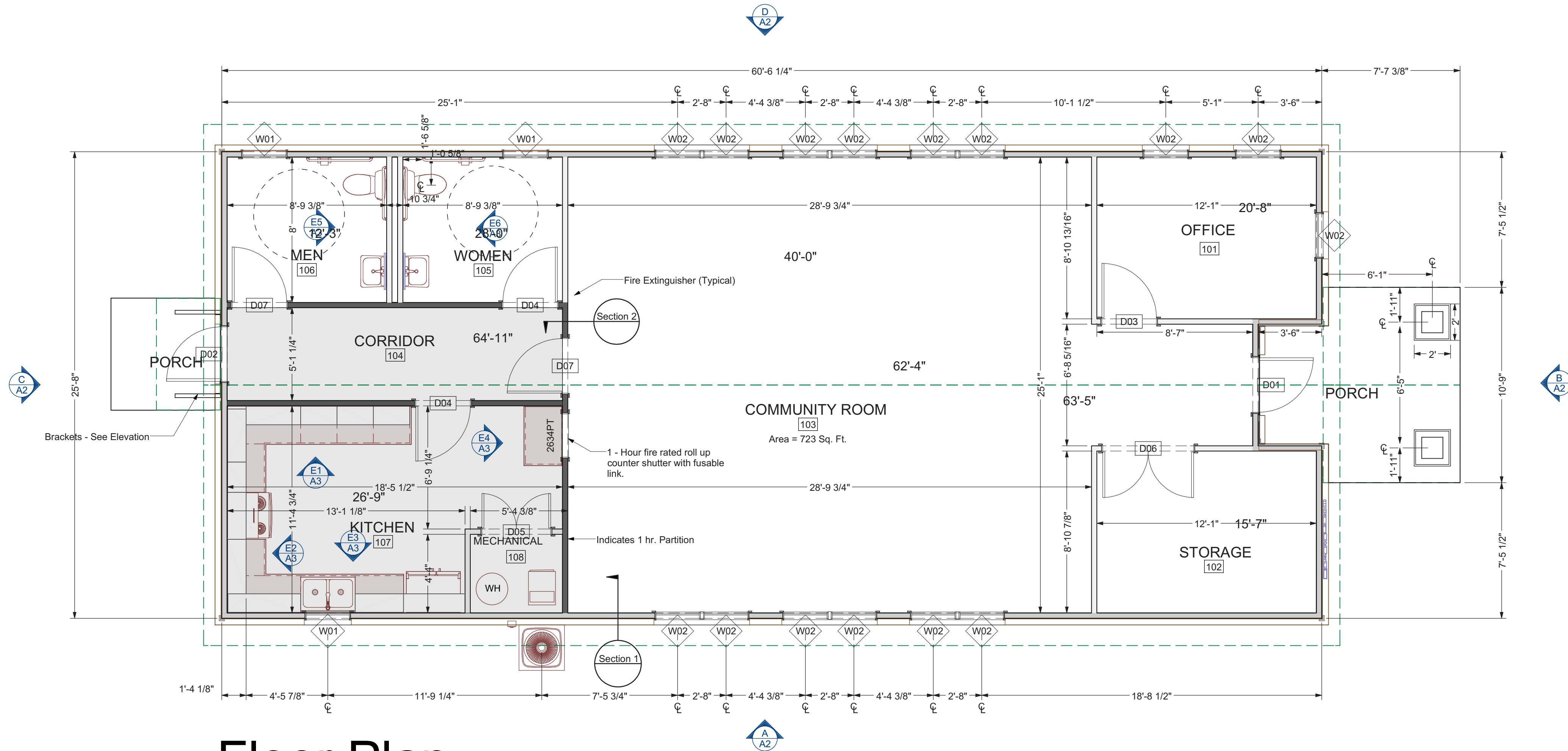
Floor Plan 1/4" = 1' - 0" (when printed on 24x36)
