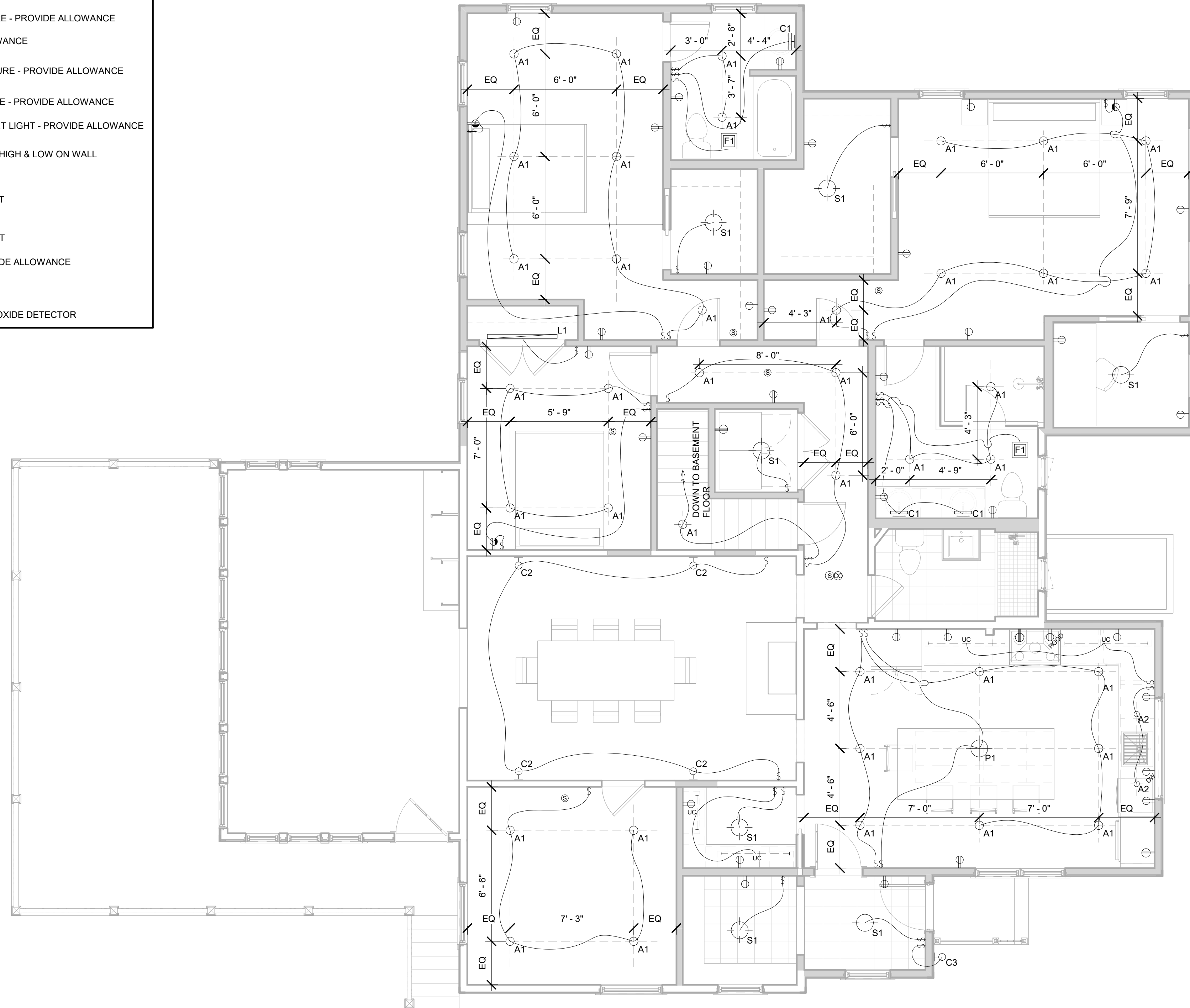
1 FIRST FLOOR REFLECTED CEILING PLAN 1/4" = 1'-0"
