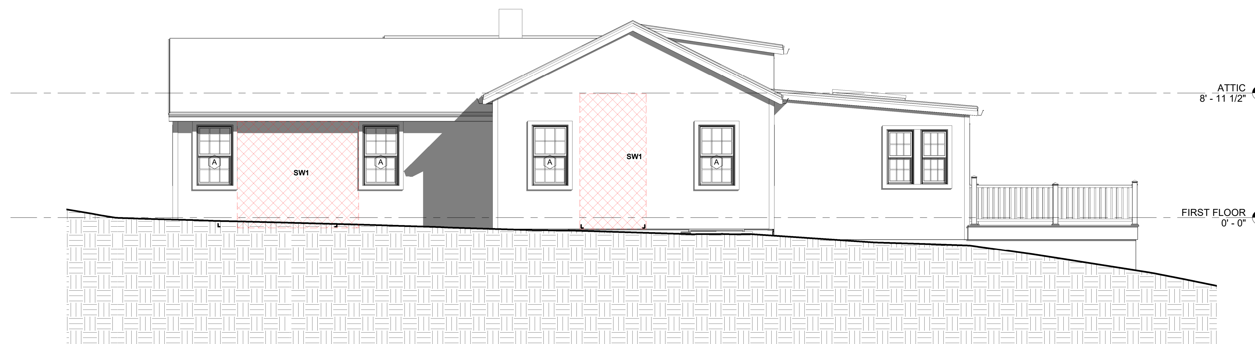
1 NORTH ELEVATION 1/4" = 1'-0"
