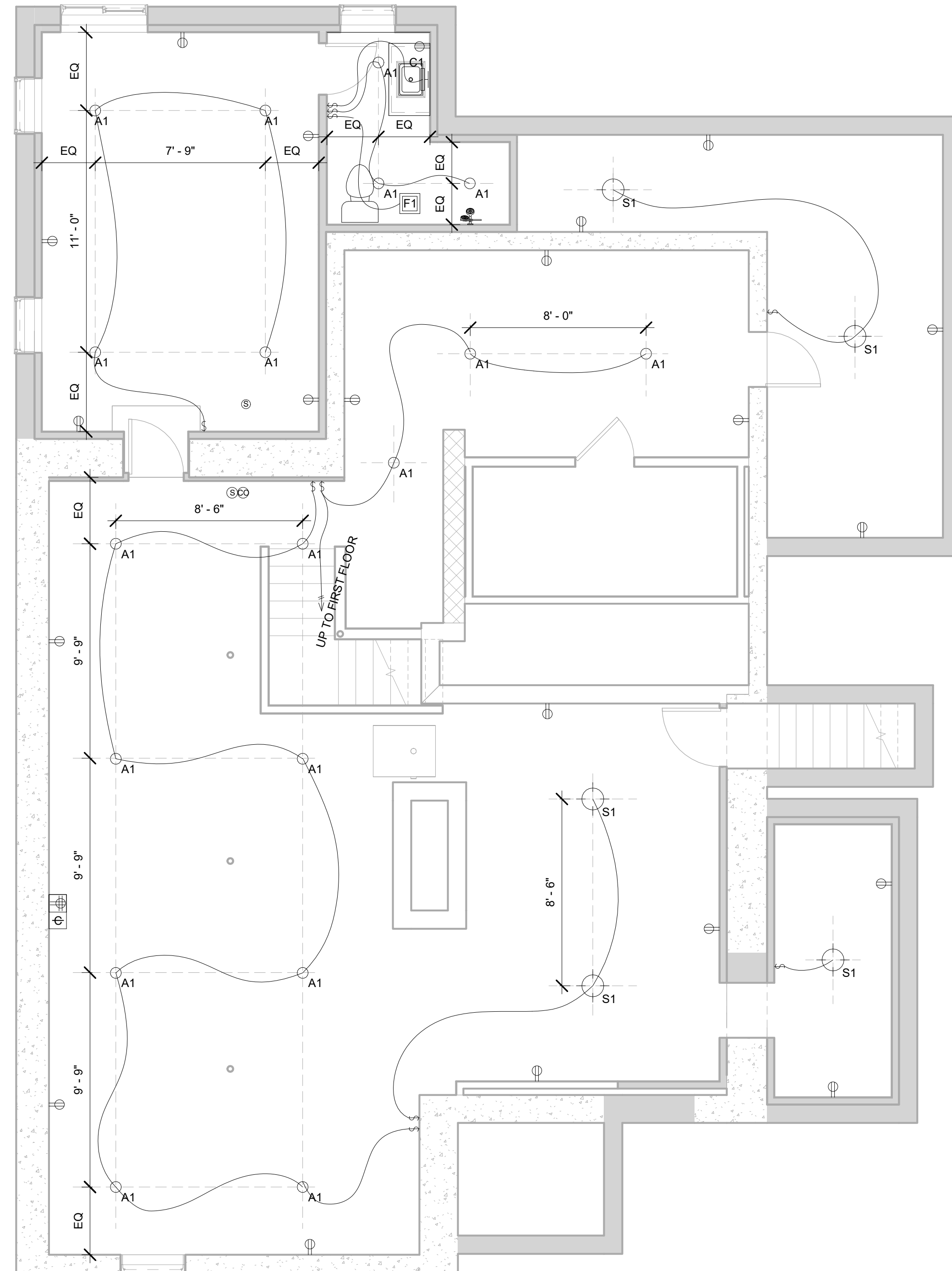
1 BASEMENT REFLECTED CEILING PLAN 1/4" = 1'-0"
