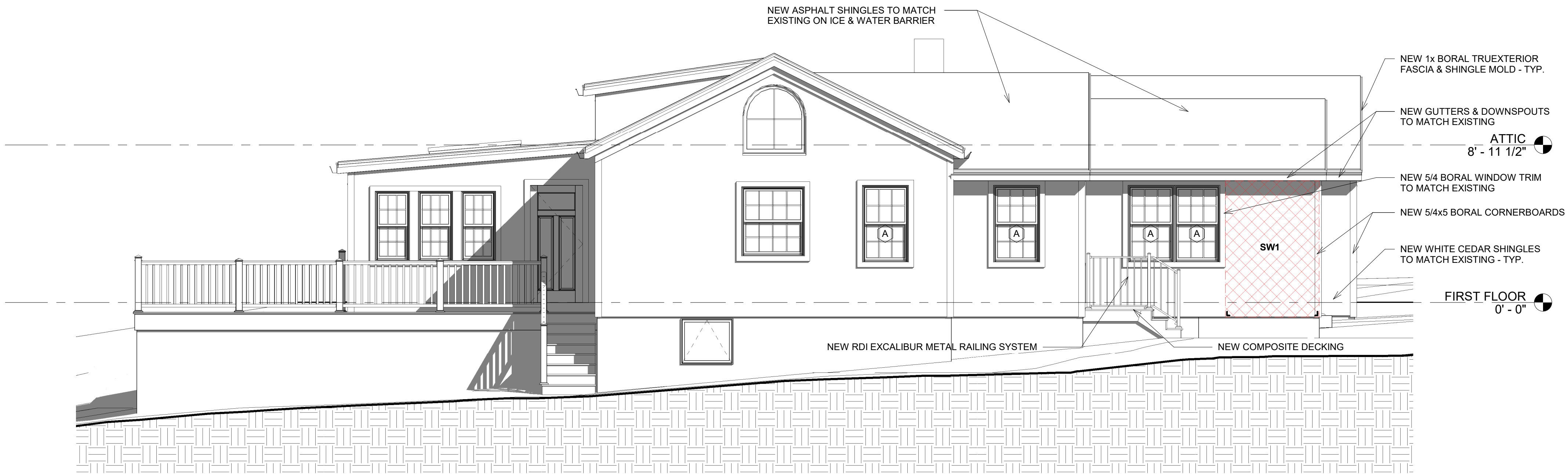
① SOUTH ELEVATION 1/4" = 1'-0"
