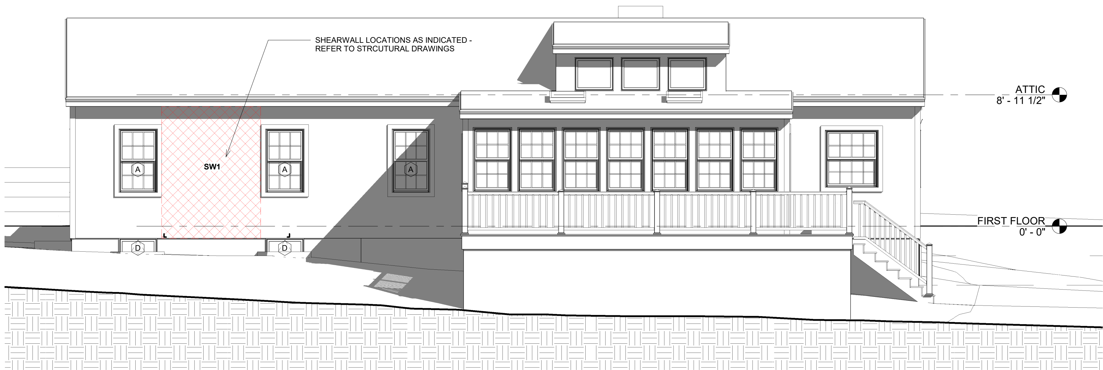
② WEST ELEVATION 1/4" = 1'-0"
