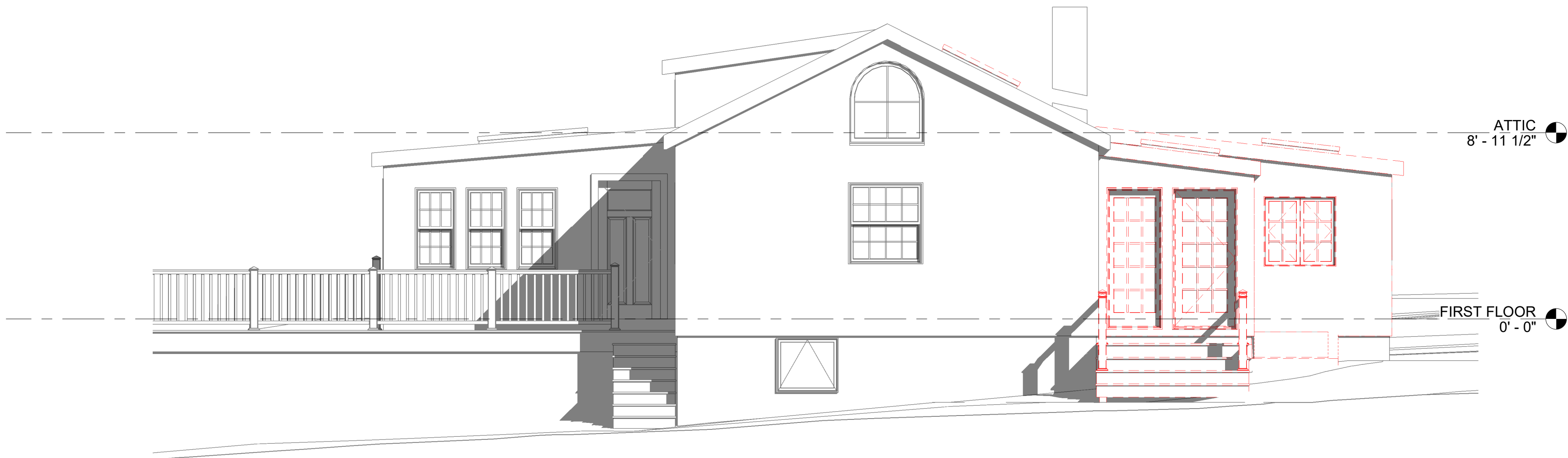
② SOUTH ELEVATION - EC/DEMO 1/4" = 1'-0"
