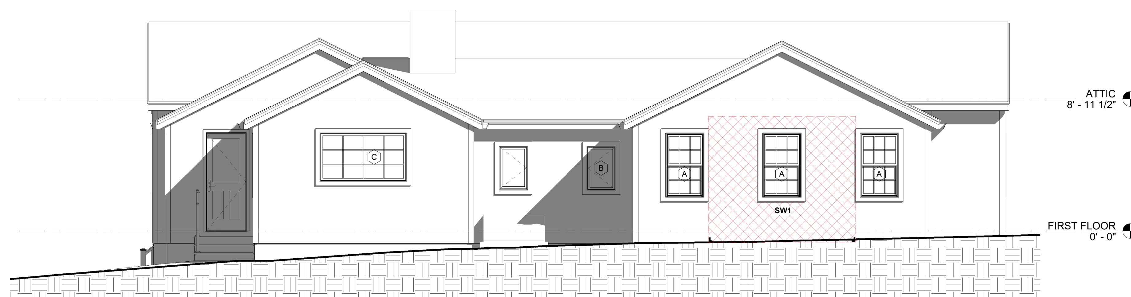
② EAST ELEVATION 1/4" = 1'-0"
