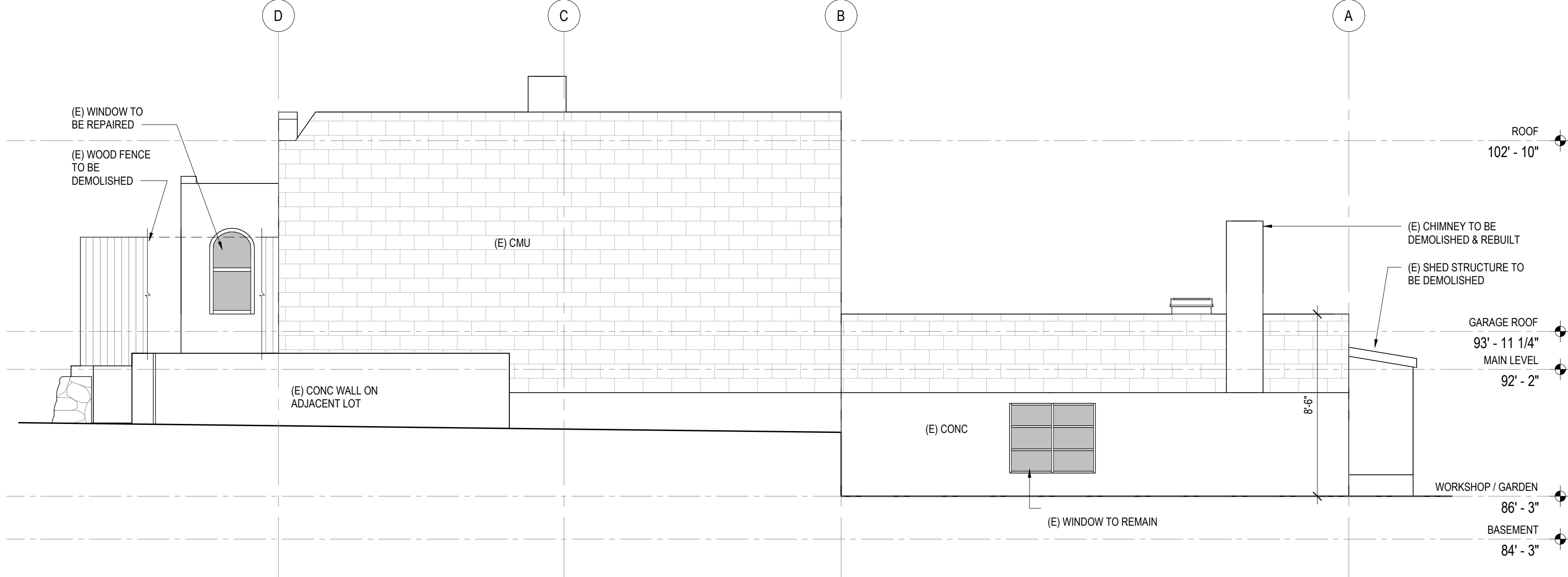
4 NORTH ELEVATION - EXISTING CONDITION SCALE: 1/4" = 1'-0"
