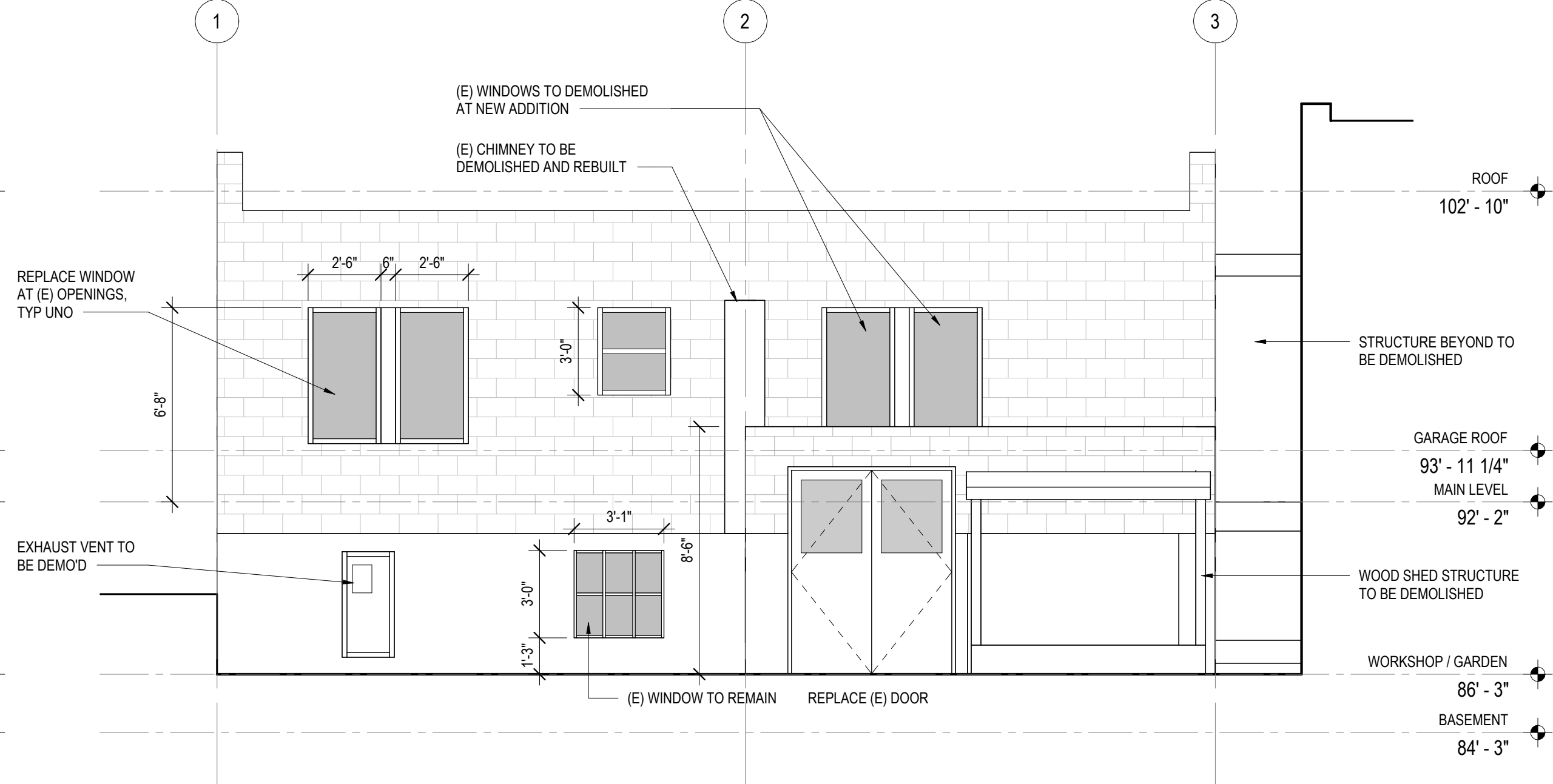
3 WEST ELEVATION - EXISTING CONDITION SCALE: 1/4" = 1'-0"
