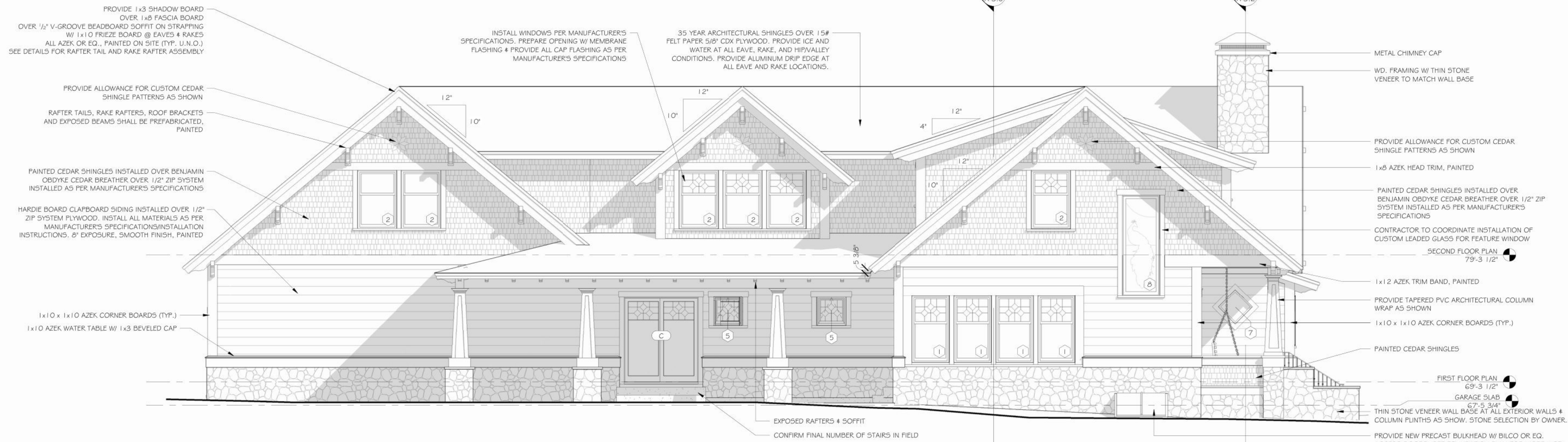
2 LEFT SIDE ELEVATION 1/4" = 1'-0"
