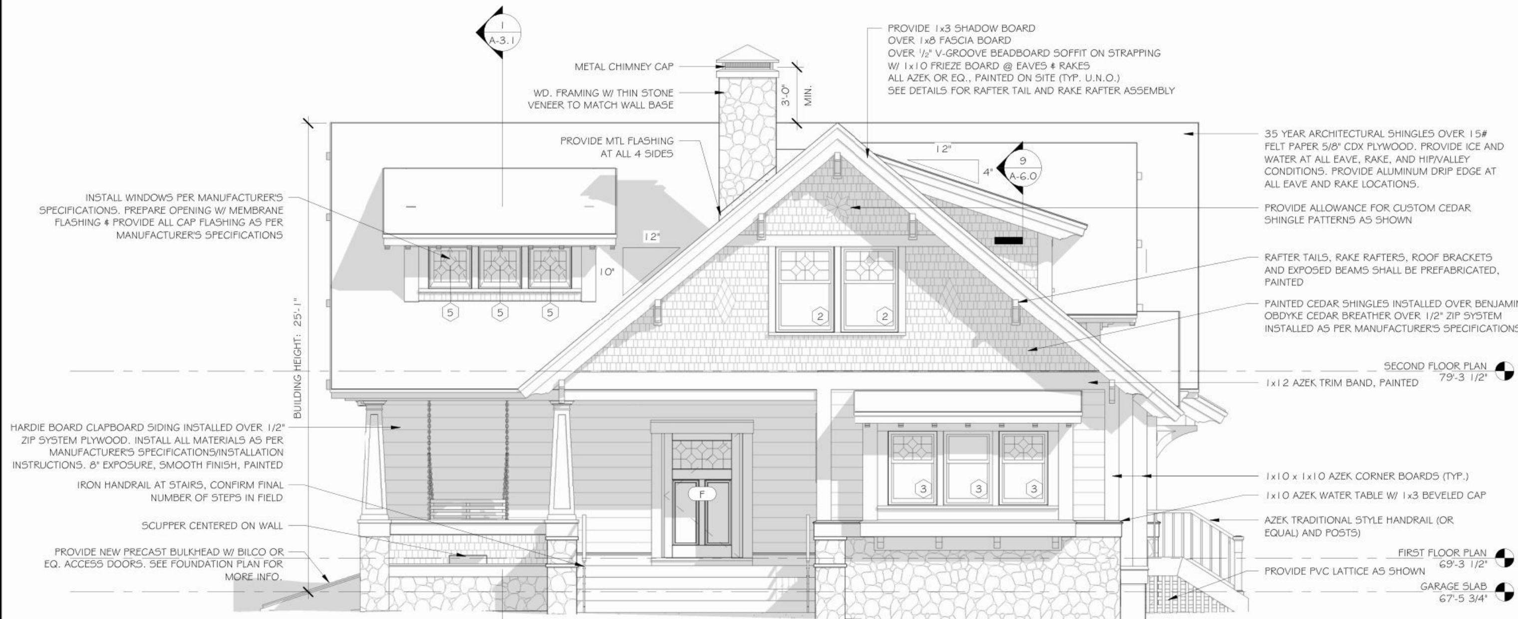
1 FRONT ELEVATION 1/4" = 1'-0"
