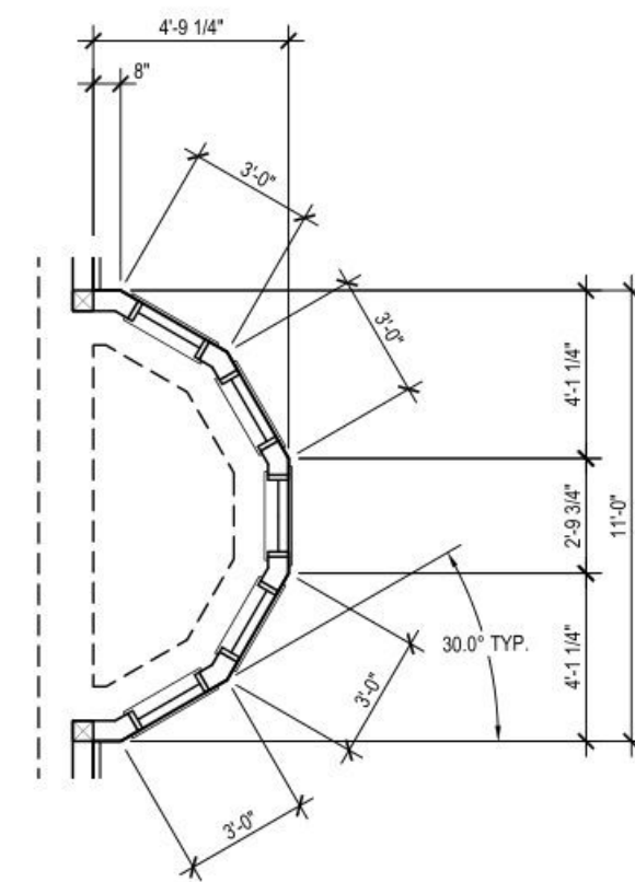
TYP. BAY WINDOW DIMENSIONS SCALE: 1/4" = 1'-0"
