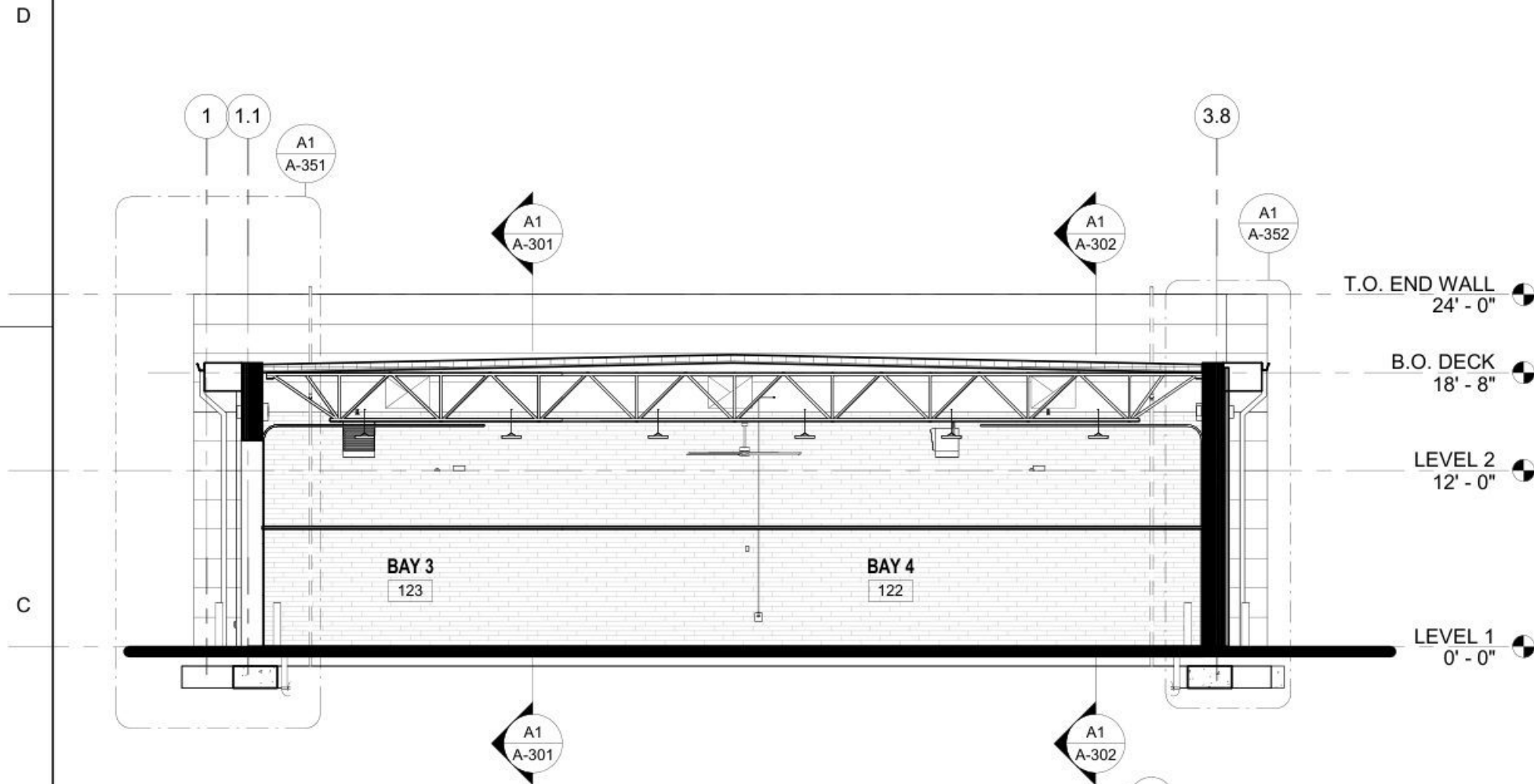
C1 BUILDING SECTION - EAST SCALE: 1/8" = 1'-0"
