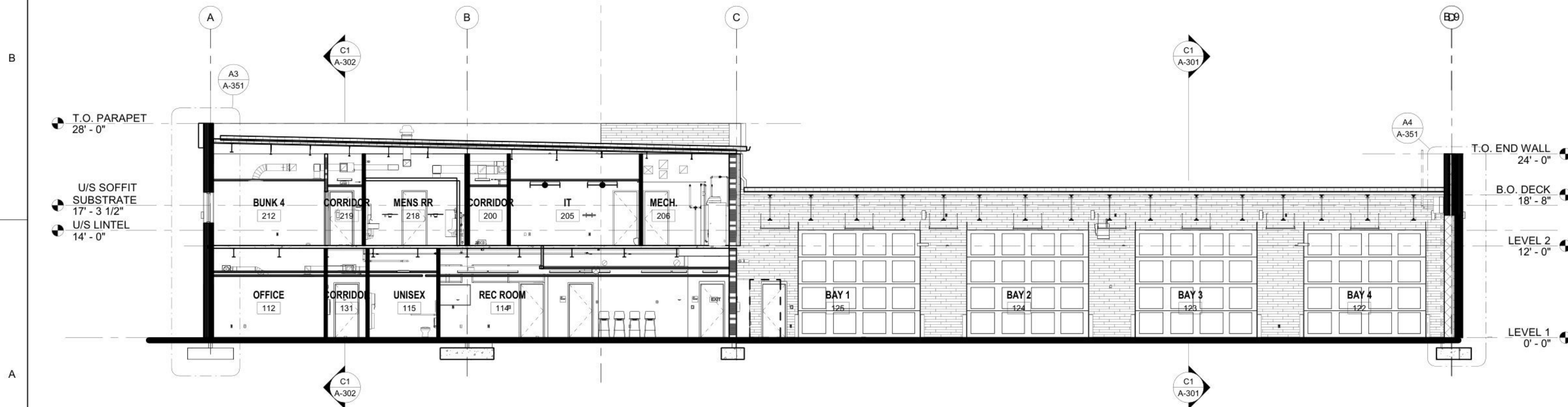
A1 BUILDING SECTION - NORTH SCALE: 1/8" = 1'-0"
