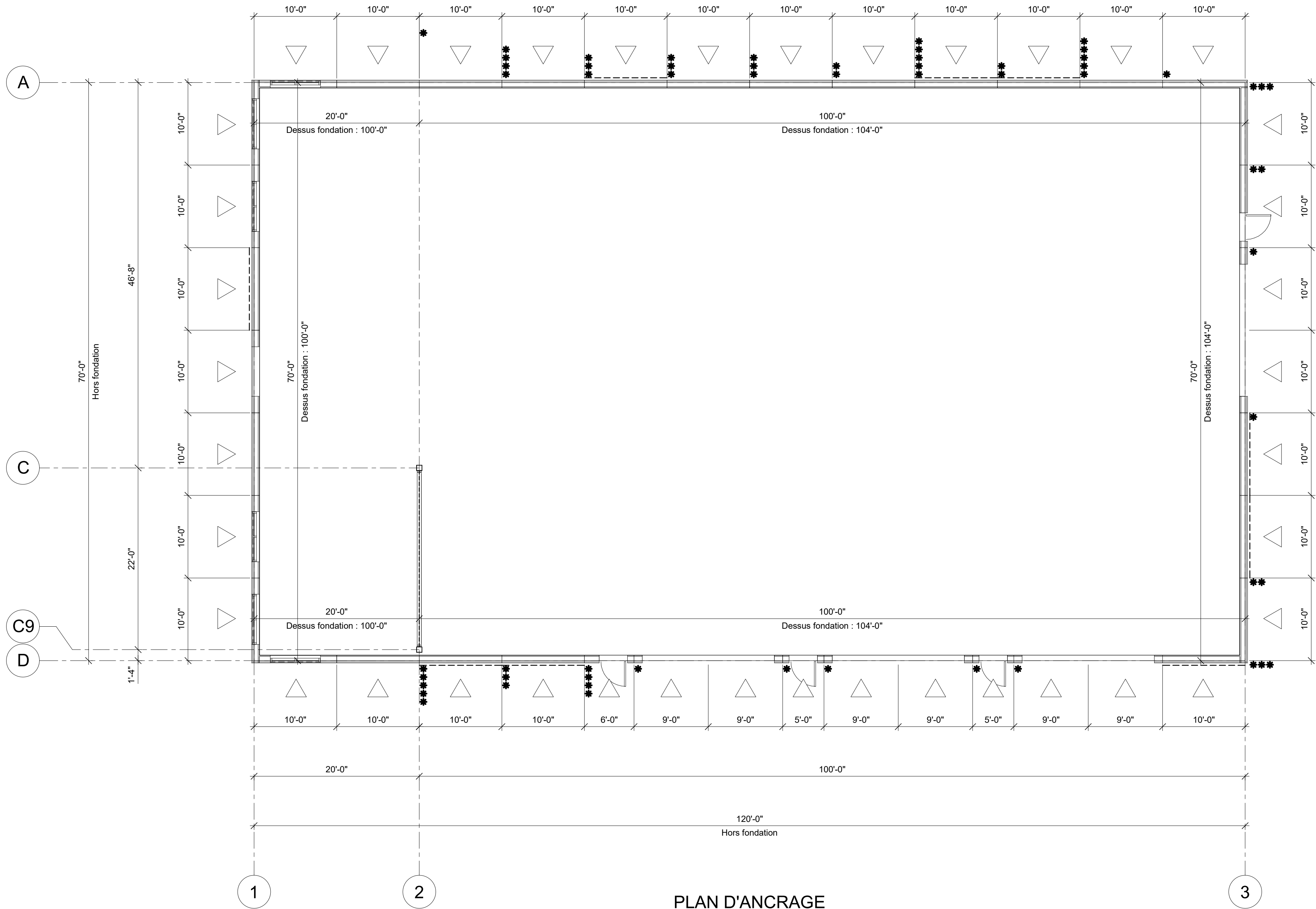
PLAN D'ANCRAGE 1/8" = 1'-0"
