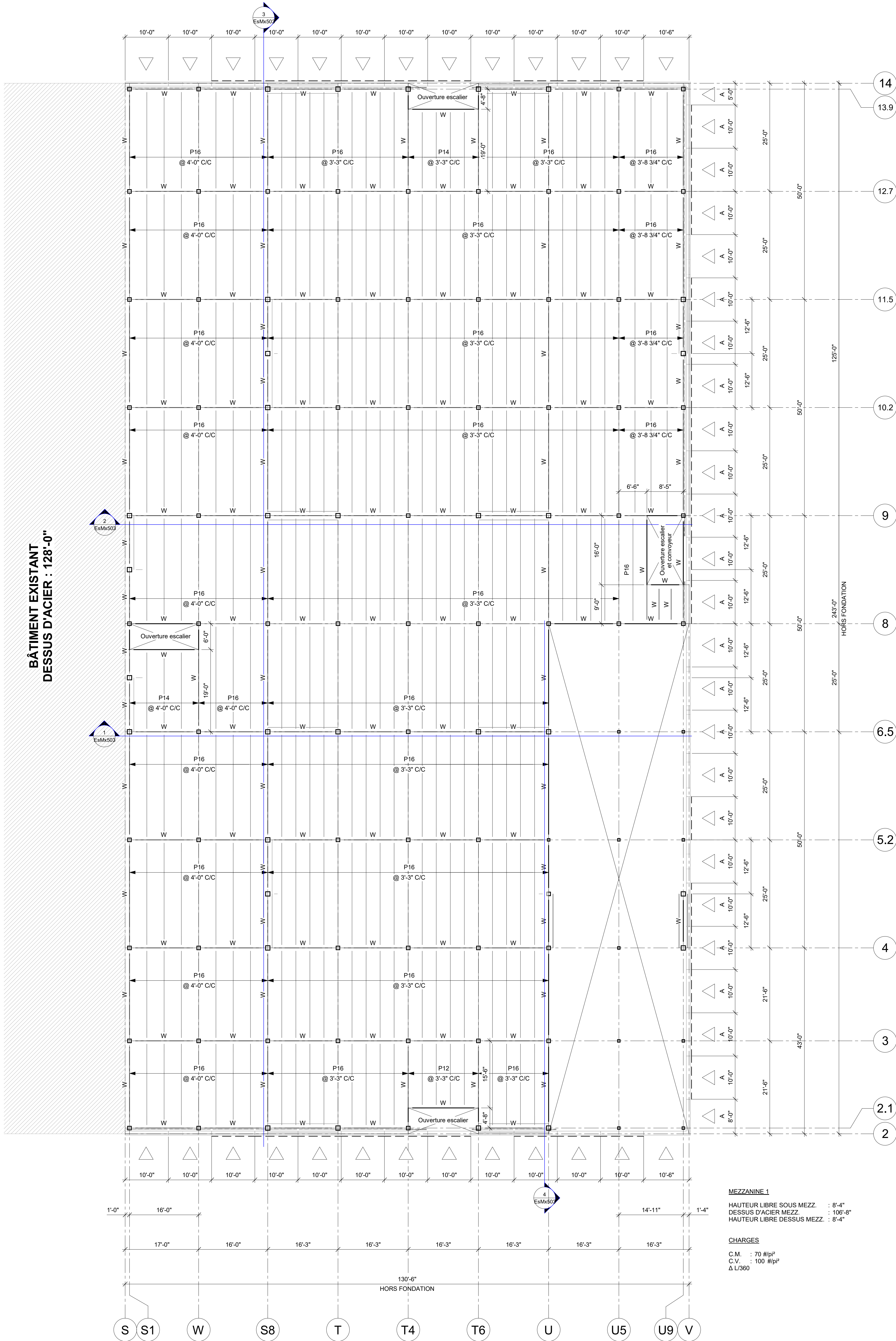
PLAN DE MEZZANINE 1 3/32" = 1'-0"
