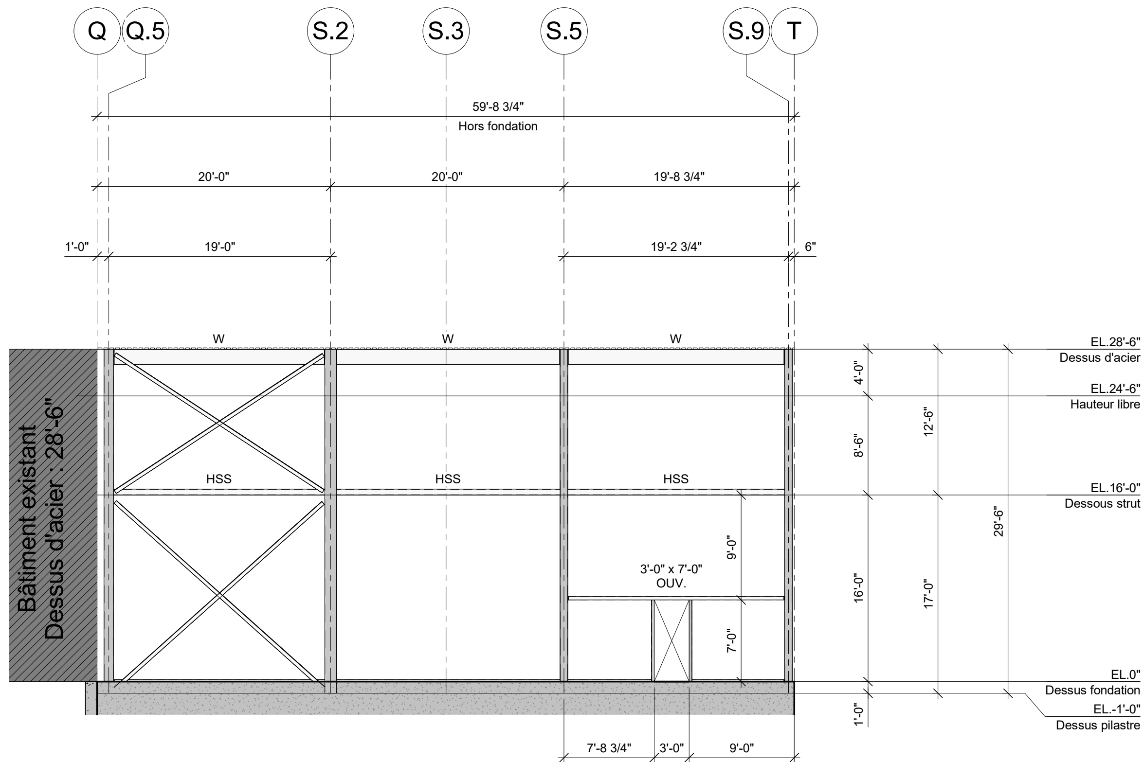
ELEVATION AXE 25 (EST) 1/8" = 1'-0"
