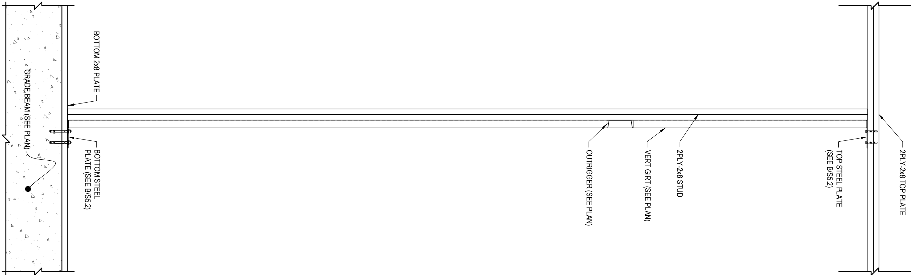
2 S5.2 SECTION SCALE : 3/4"=1'-0"
