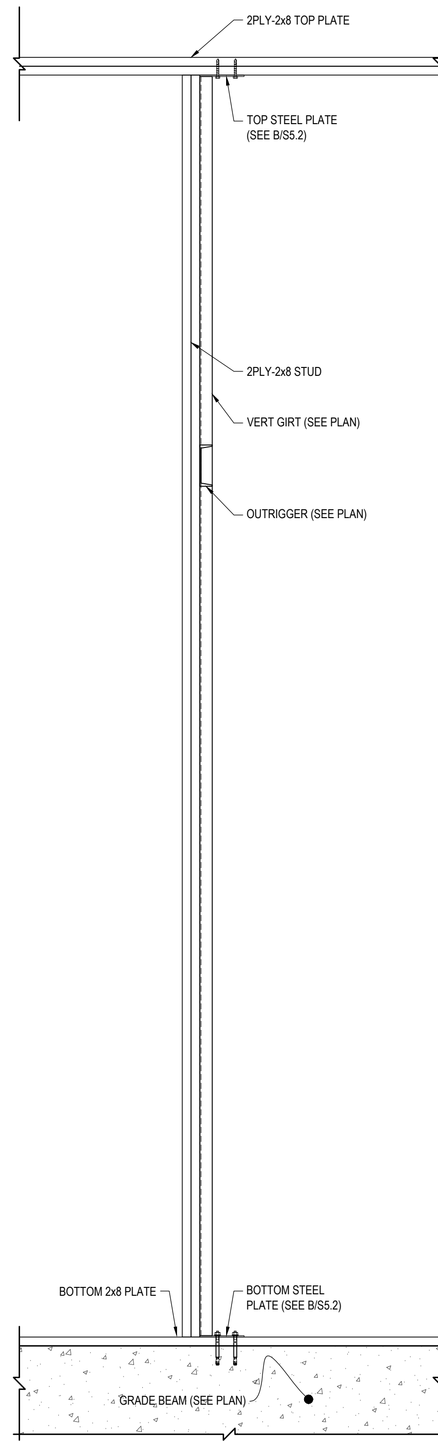
2 S5.2 SECTION SCALE : 3/4"=1'-0"
