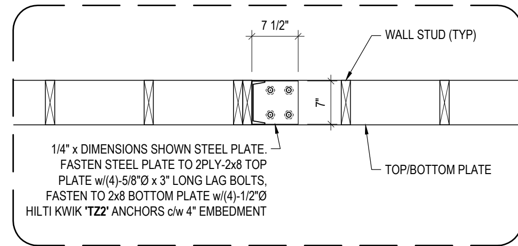
B S5.2 DETAIL SCALE : 3/4"=1'-0"
