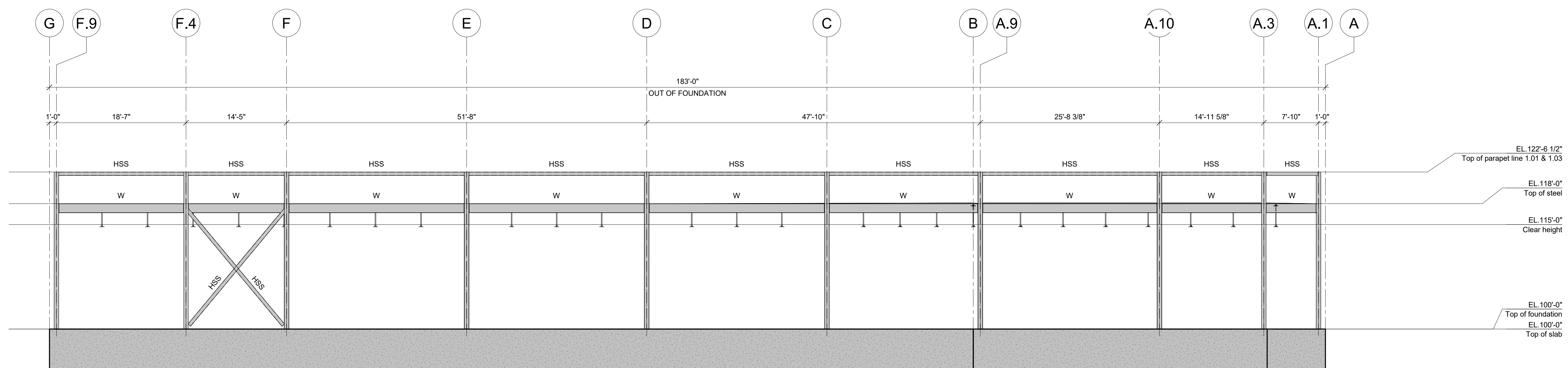
ELEVATION LINE 1.01 & 1.03 (NORTH) 1/8" = 1'-0"
