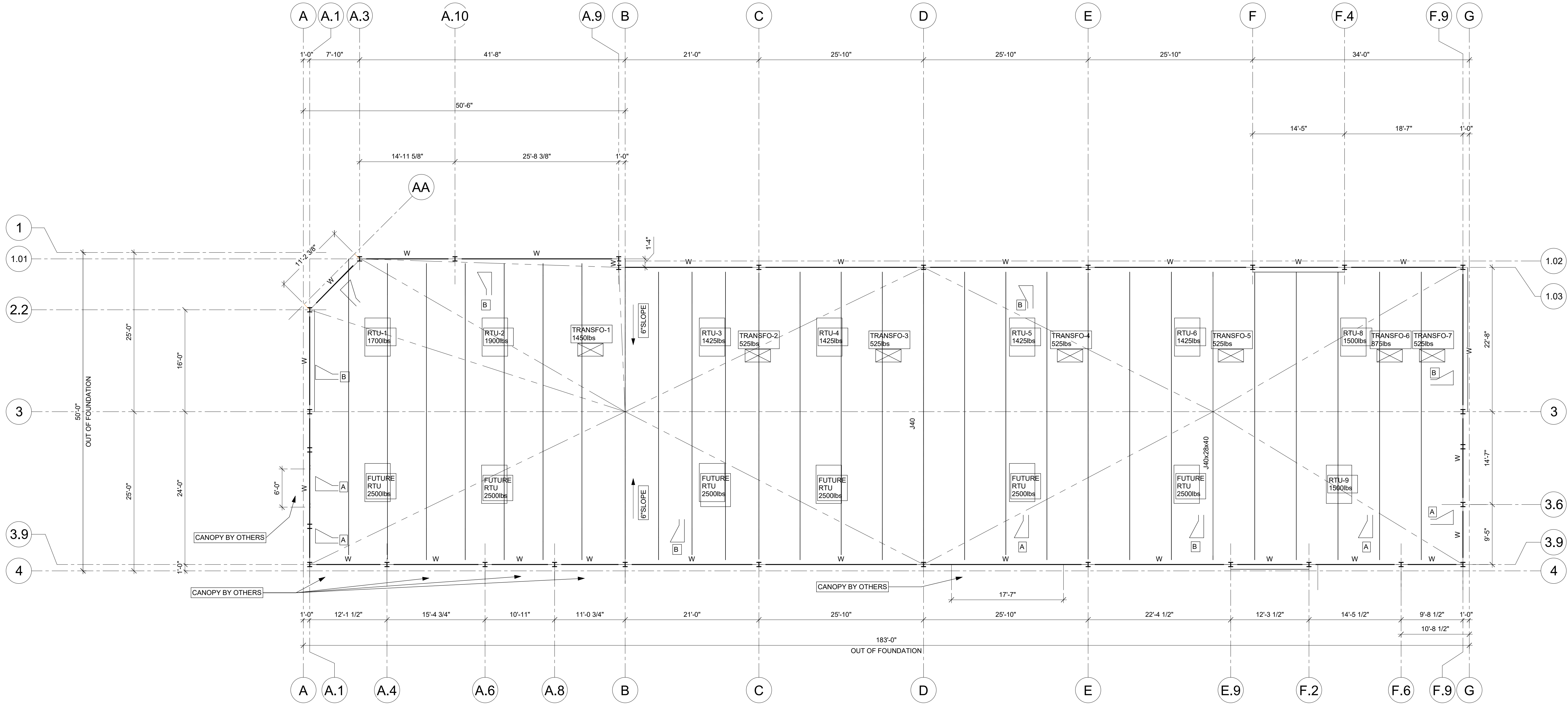
ROOF PLAN 1/8" = 1'-0"
