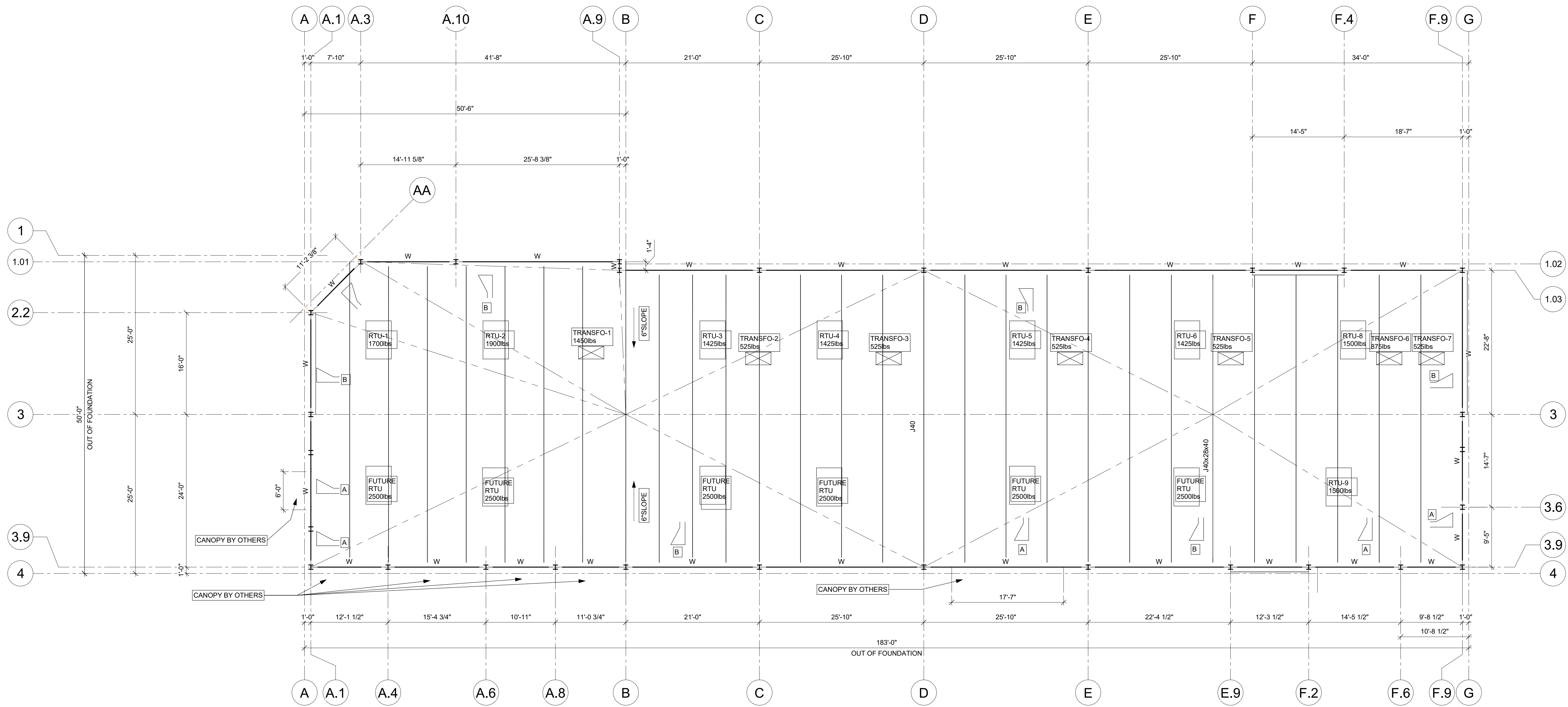
ROOF PLAN 1/8" = 1'-0"
