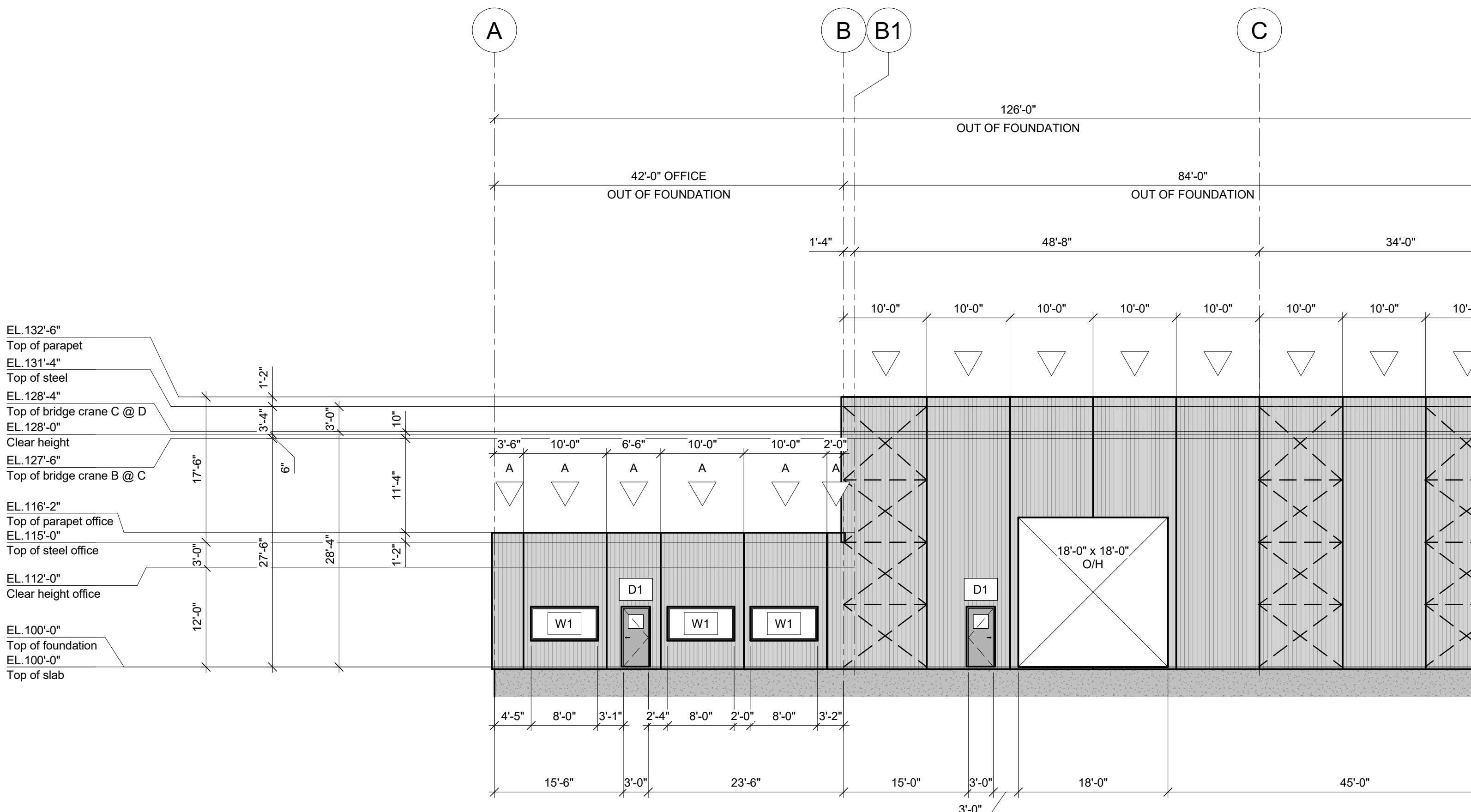
ELEVATION LINE 1 (SOUTH) 3/32" = 1'-0"
