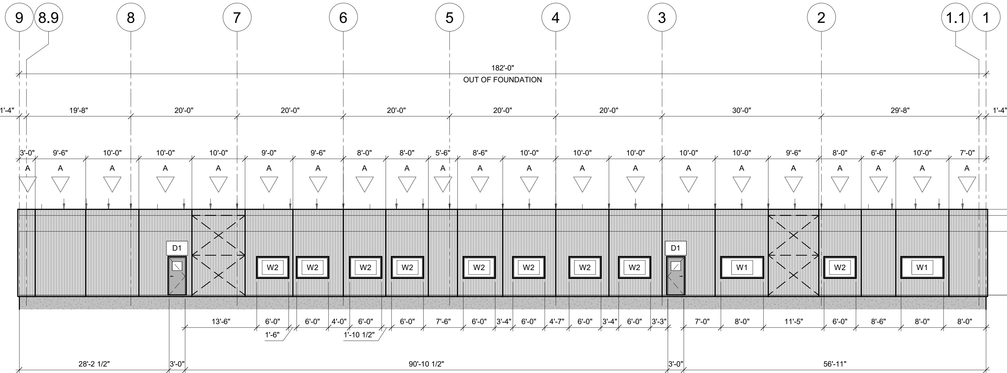
ELEVATION LINE A (WEST) 3/32" = 1'-0"
