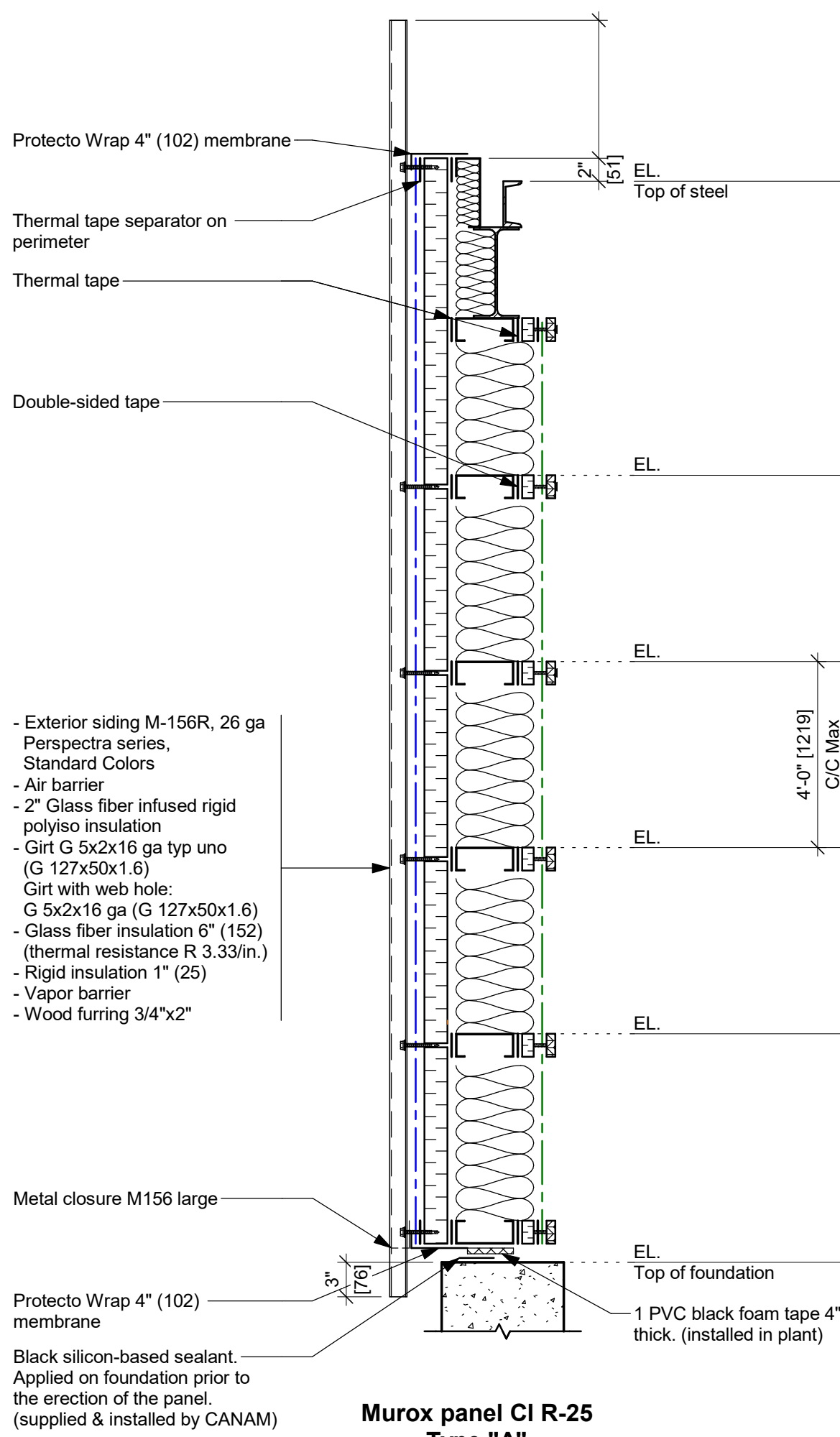
Murox panel CI R-25 Type "A"
