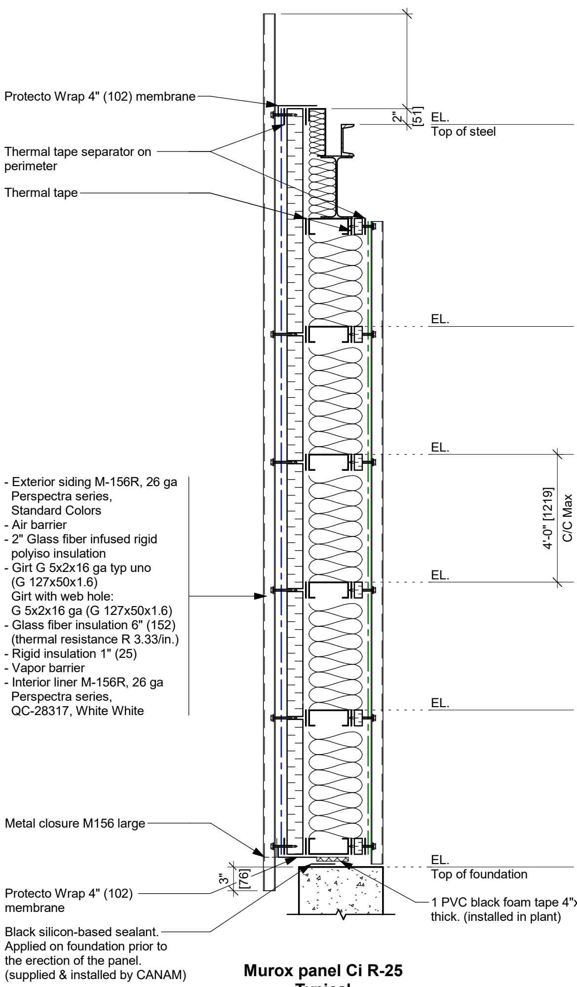
Murox panel CI R-25 Typical
