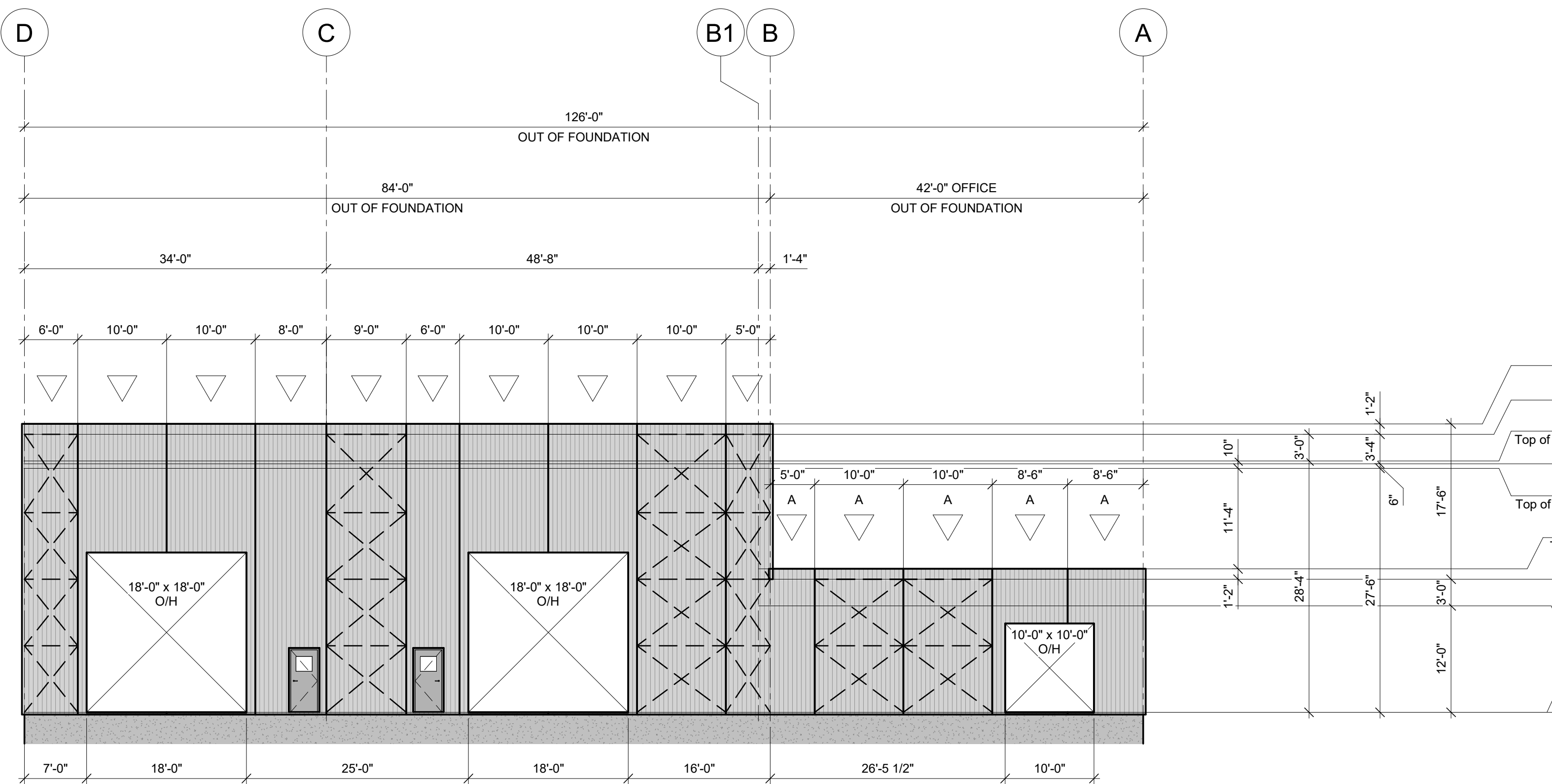
ELEVATION LINE 9 (NORTH) 3/32" = 1'-0"
