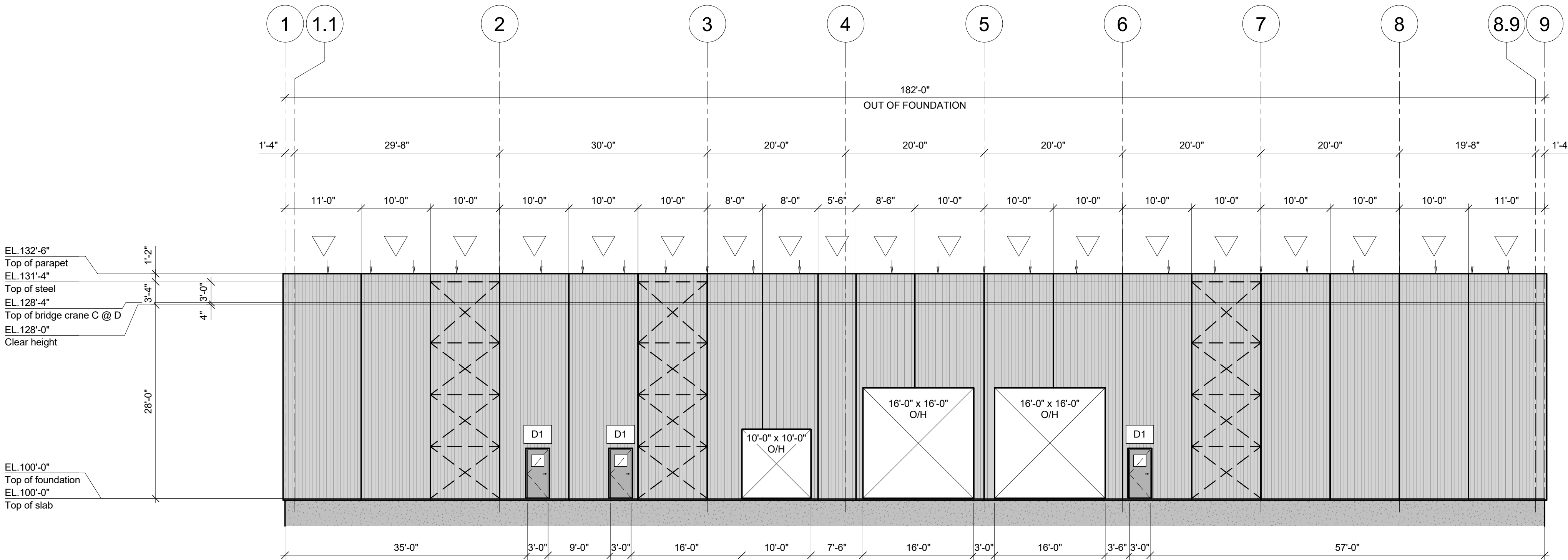
ELEVATION LINE D (EAST) 3/32" = 1'-0"
