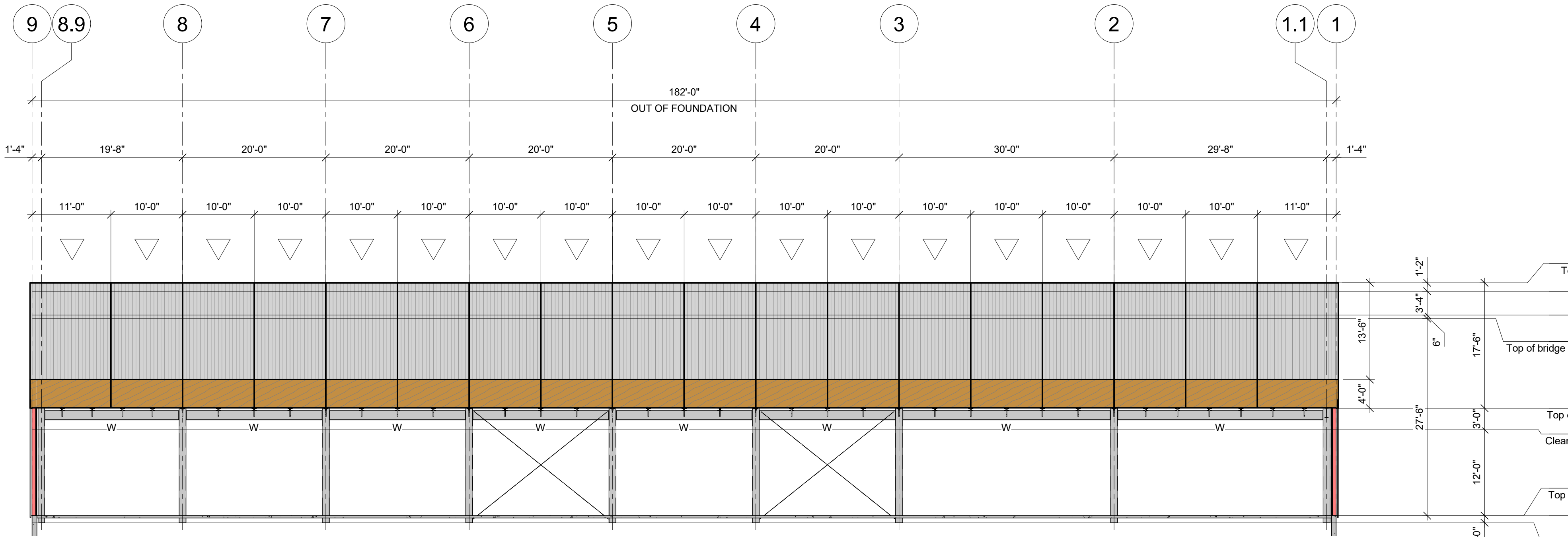
ELEVATION LINE B (WEST) 3/32" = 1'-0"
