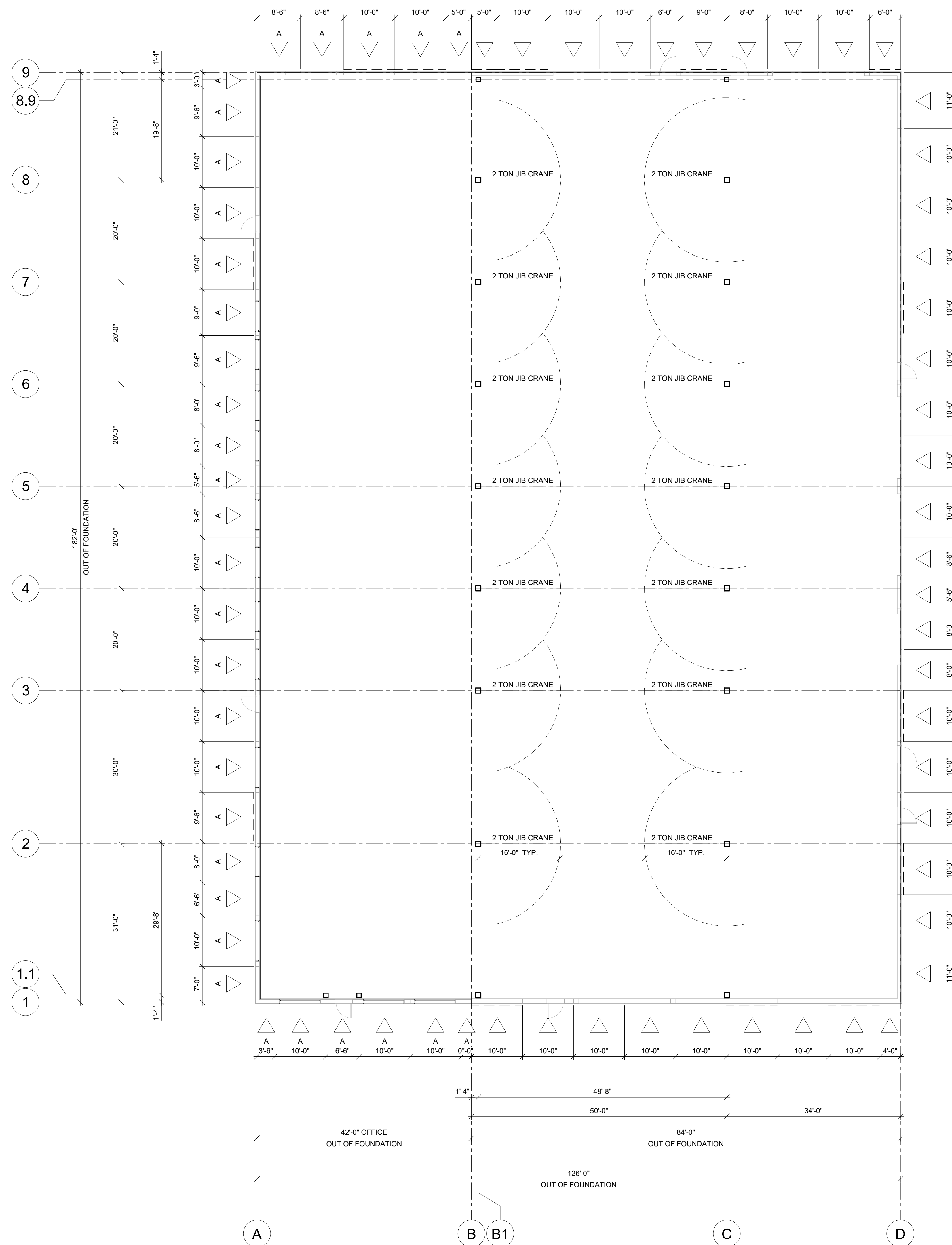
ANCHOR PLAN 3/32" = 1'-0"
