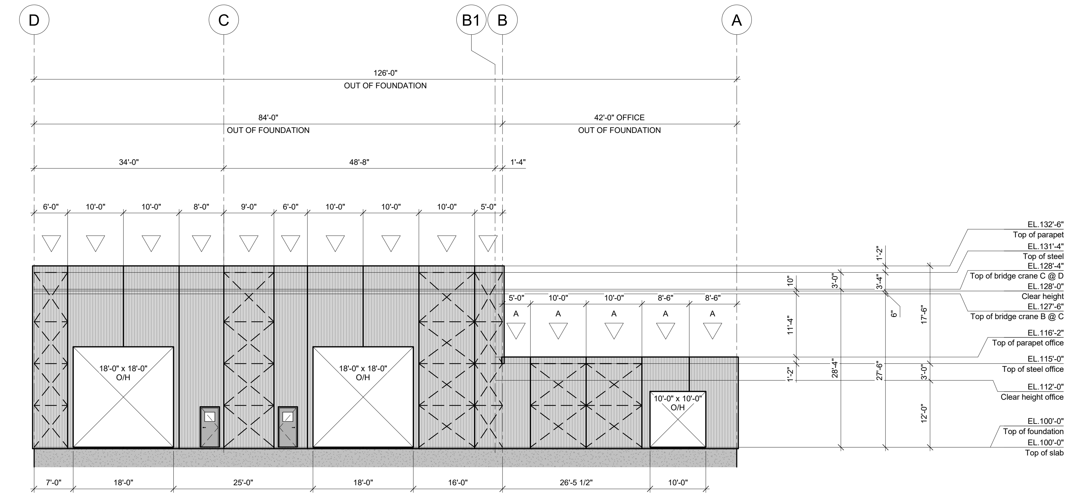
ELEVATION LINE 9 (NORTH)
