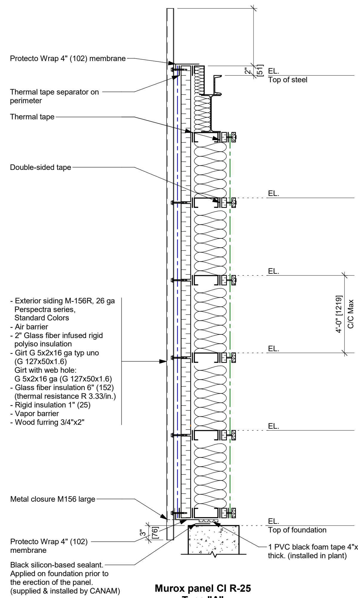
Murox panel CI R-25 Type "A"
