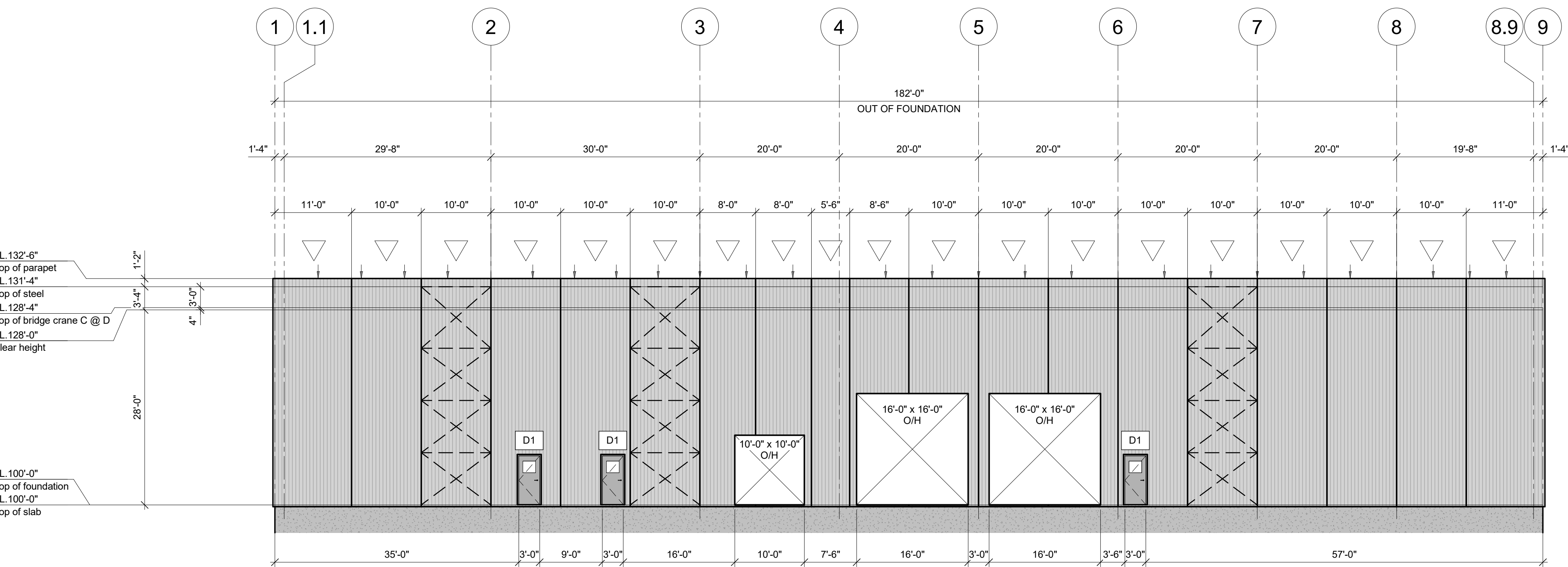
ELEVATION LINE D (EAST)
