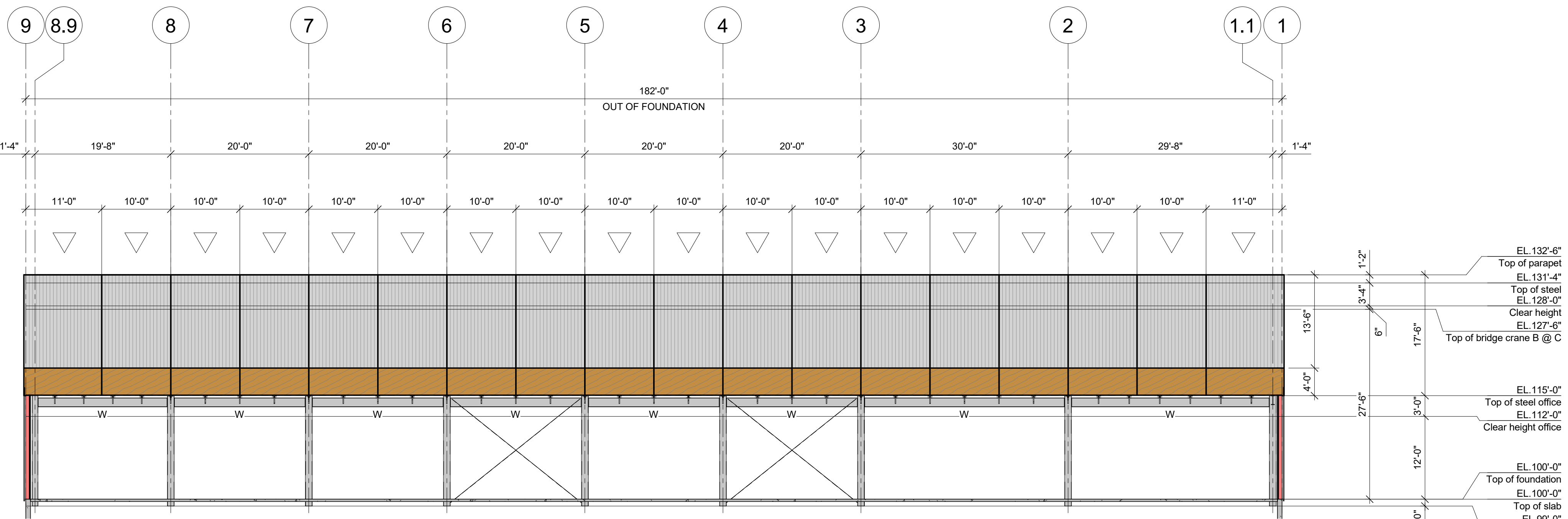
ELEVATION LINE B (WEST)
