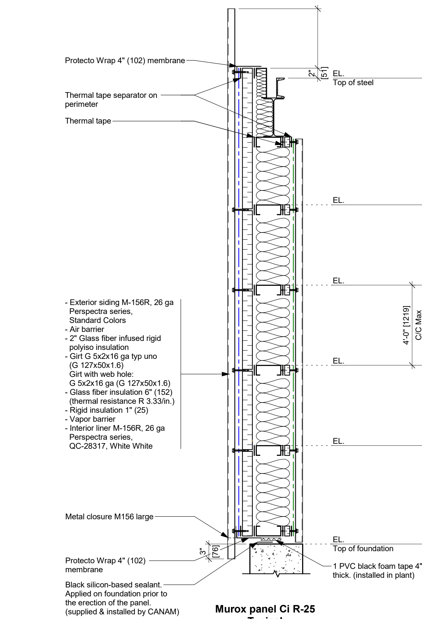
Murox panel CI R-25 Typical
