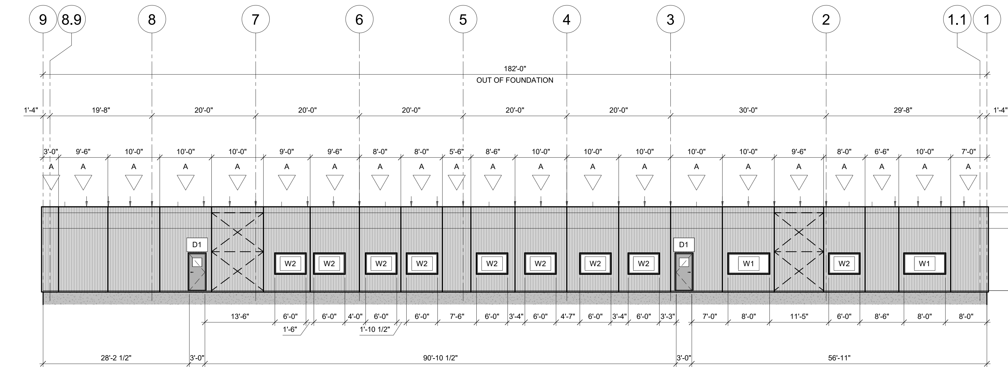
ELEVATION LINE A (WEST)
