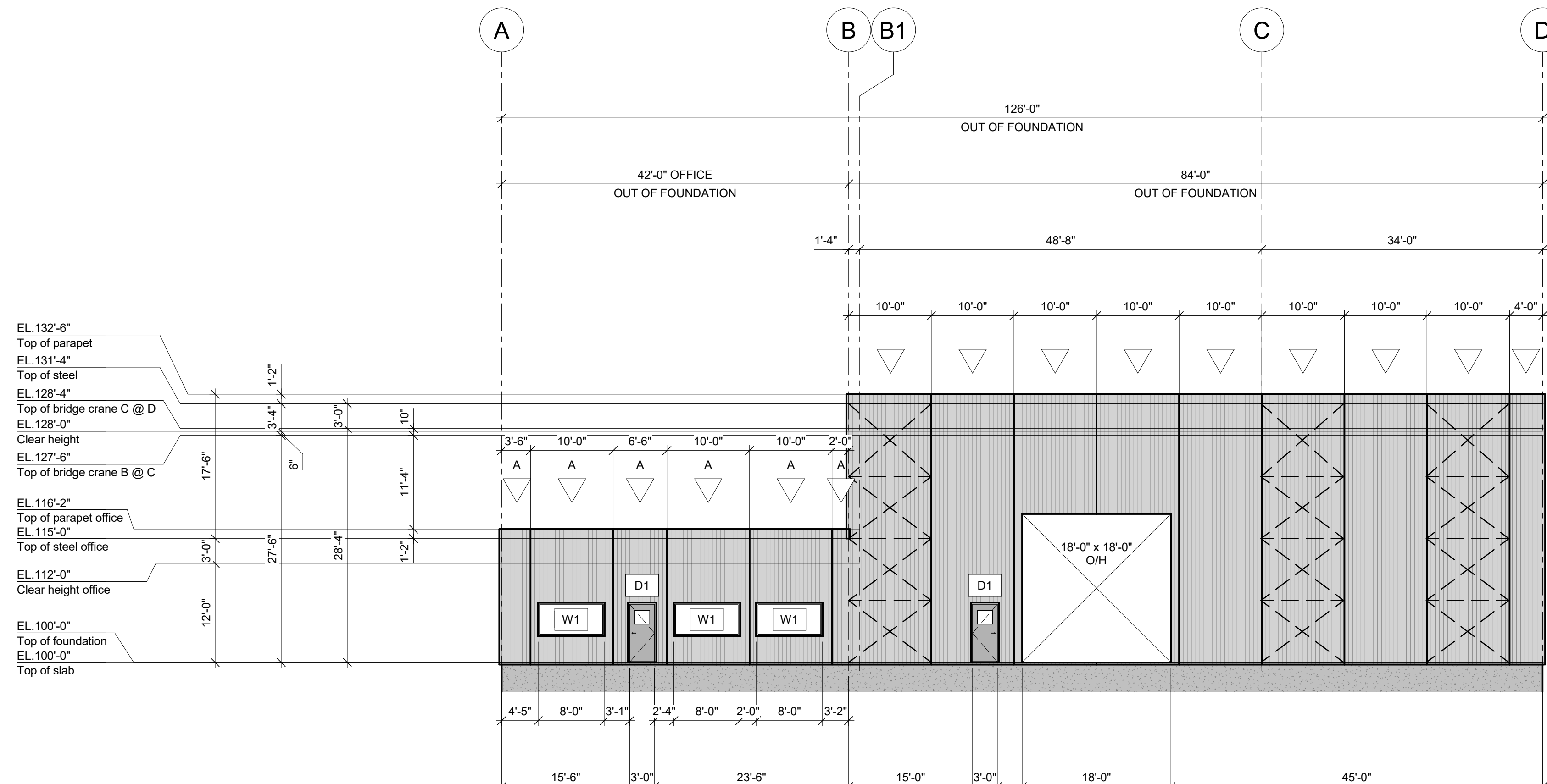
ELEVATION LINE 1 (SOUTH)
