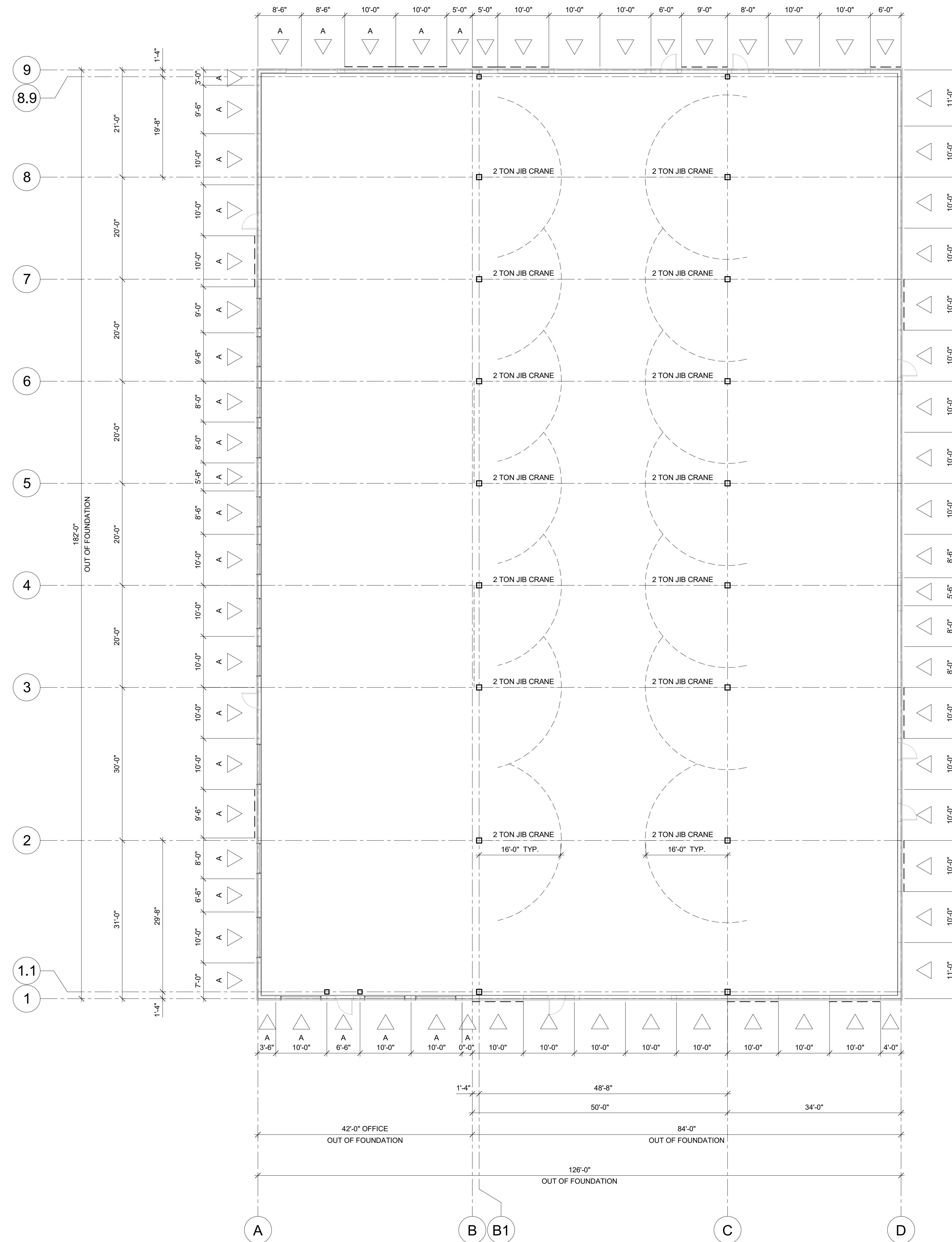
ANCHOR PLAN 3/32" = 1'-0"
