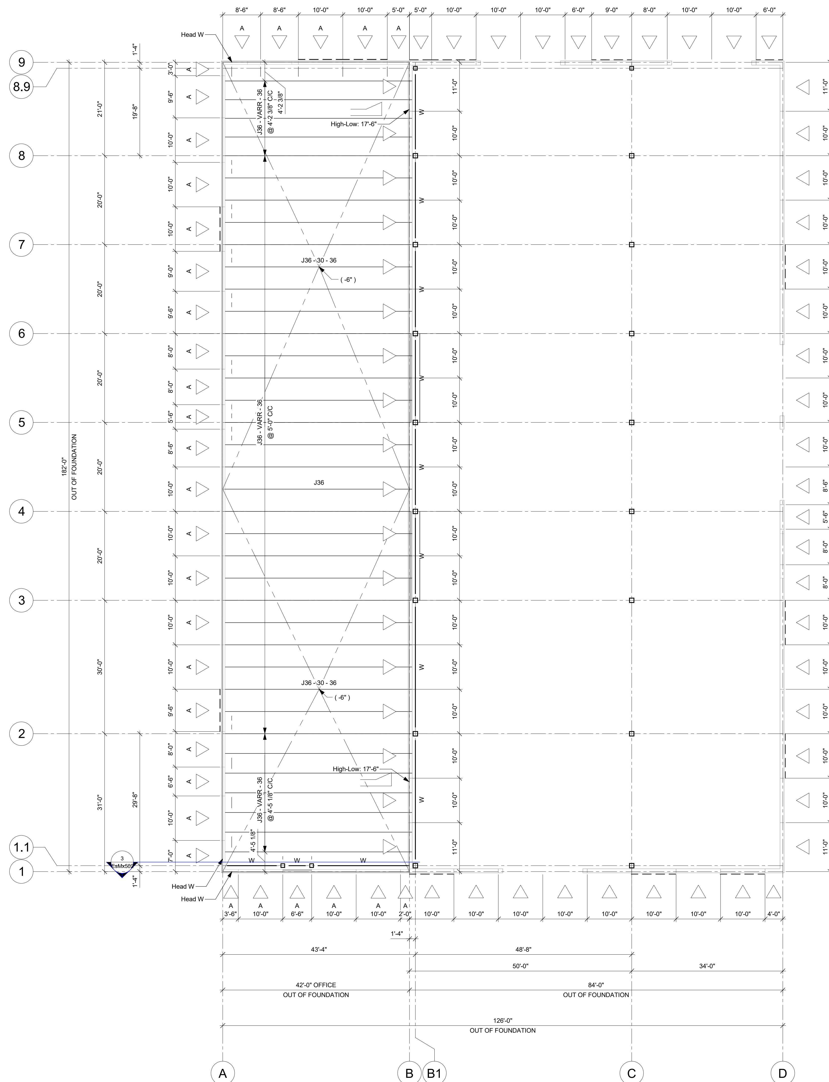
OFFICE ROOF PLAN 3/32" = 1'-0"
