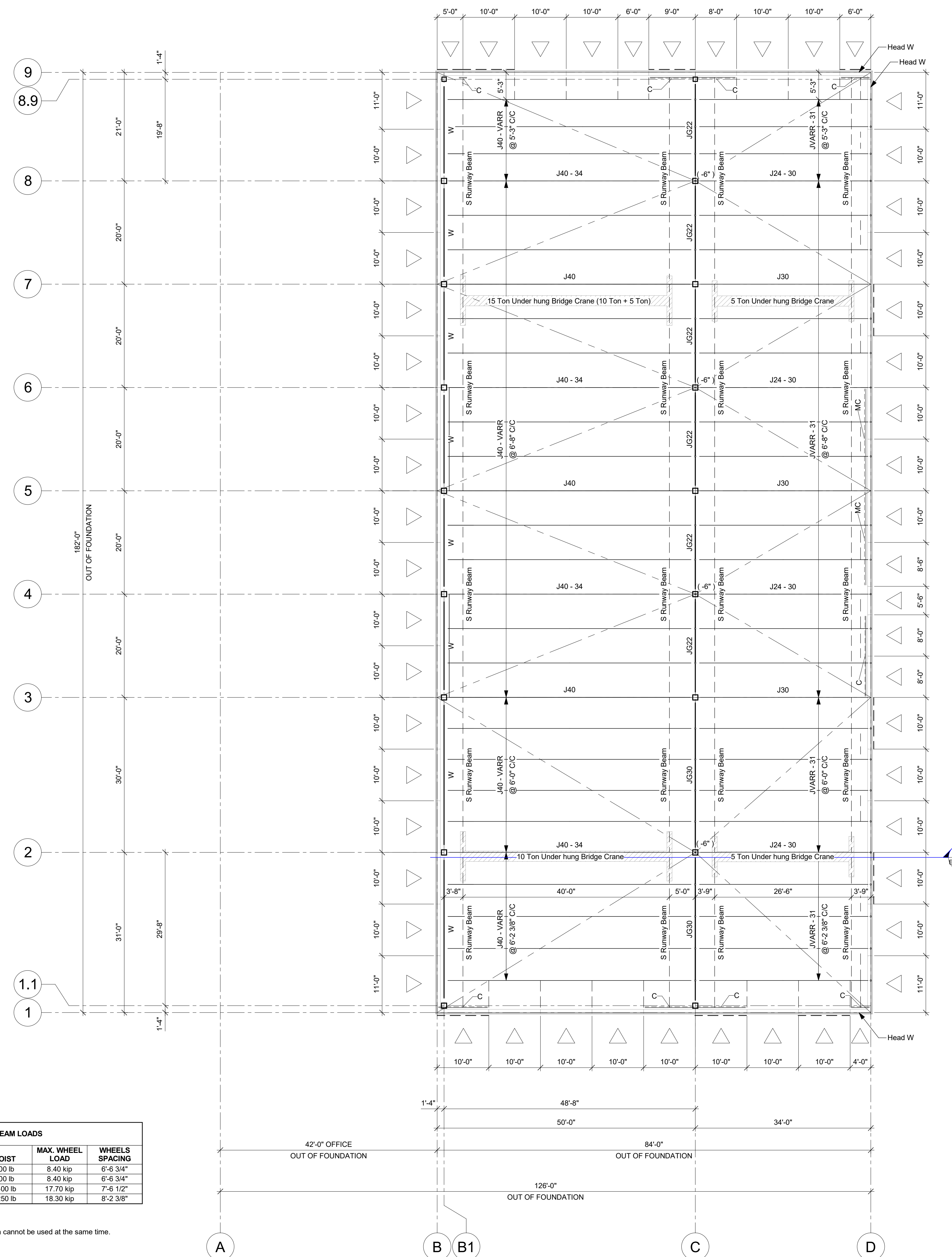
ROOF PLAN 3/32" = 1'-0"
