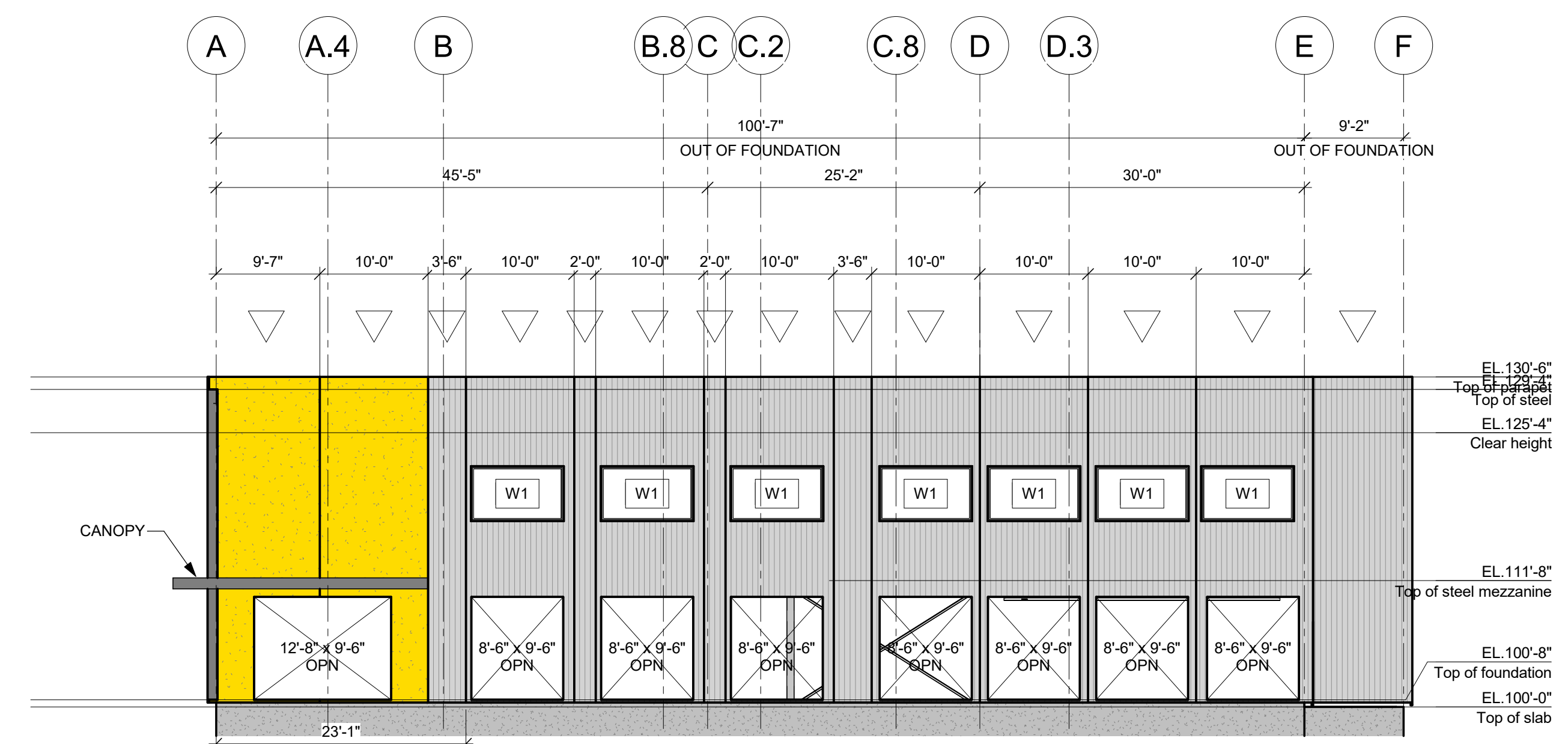
ELEVATION LINE 1 (WEST) 3/32" = 1'-0"
