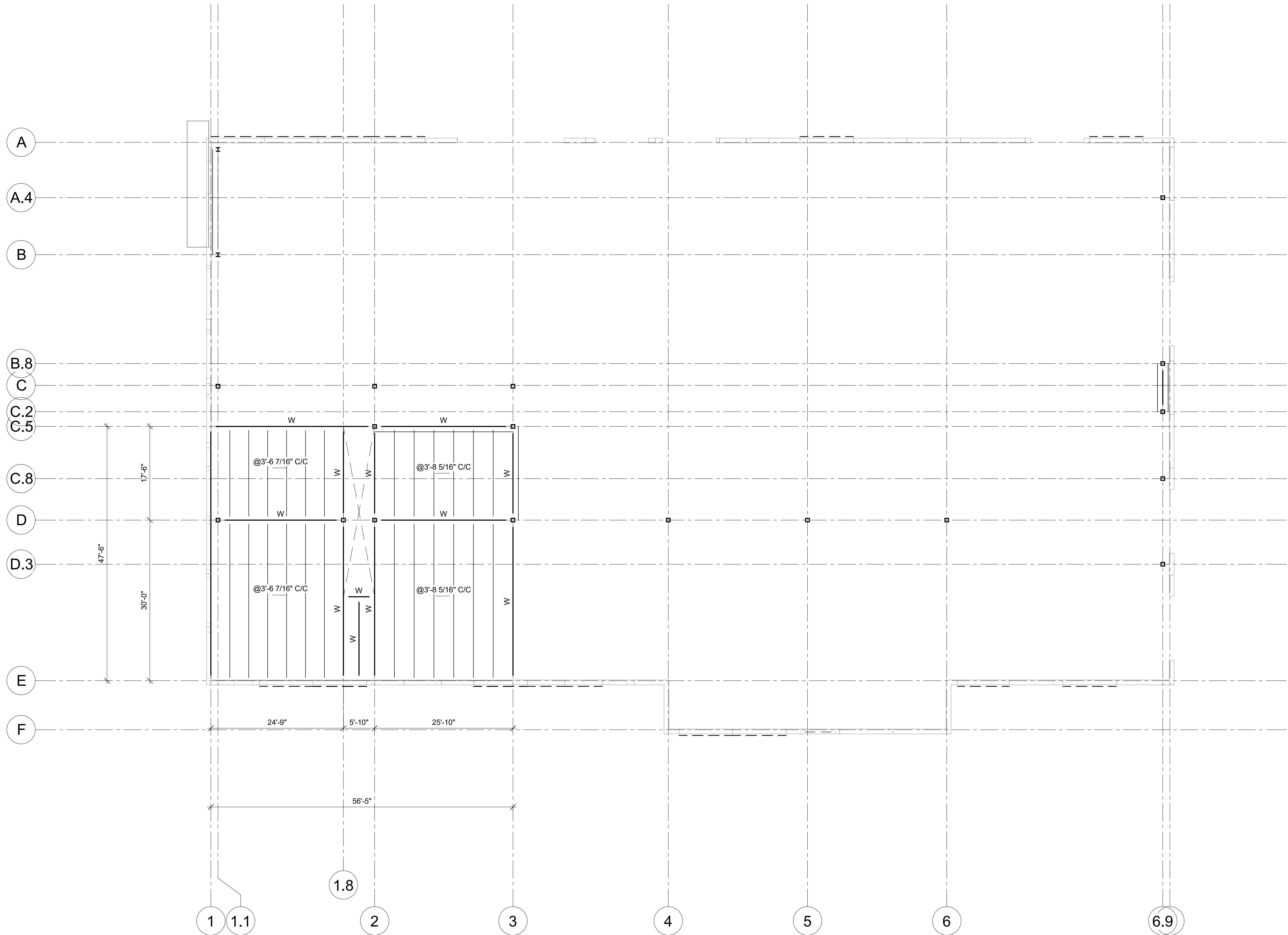
MEZZANINE PLAN 3/32" = 1'-0"
