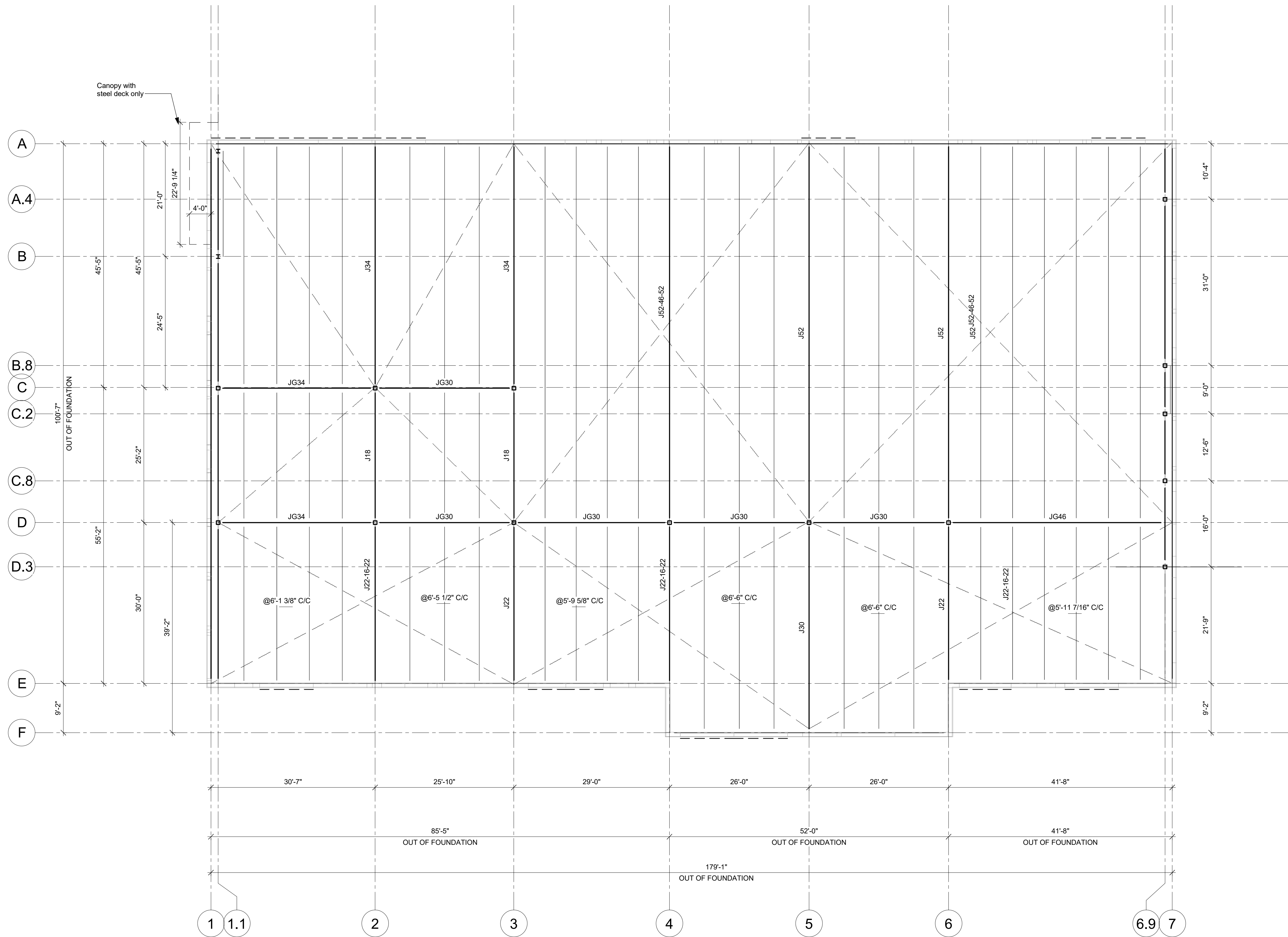
ROOF PLAN 1" = 10'-0"
