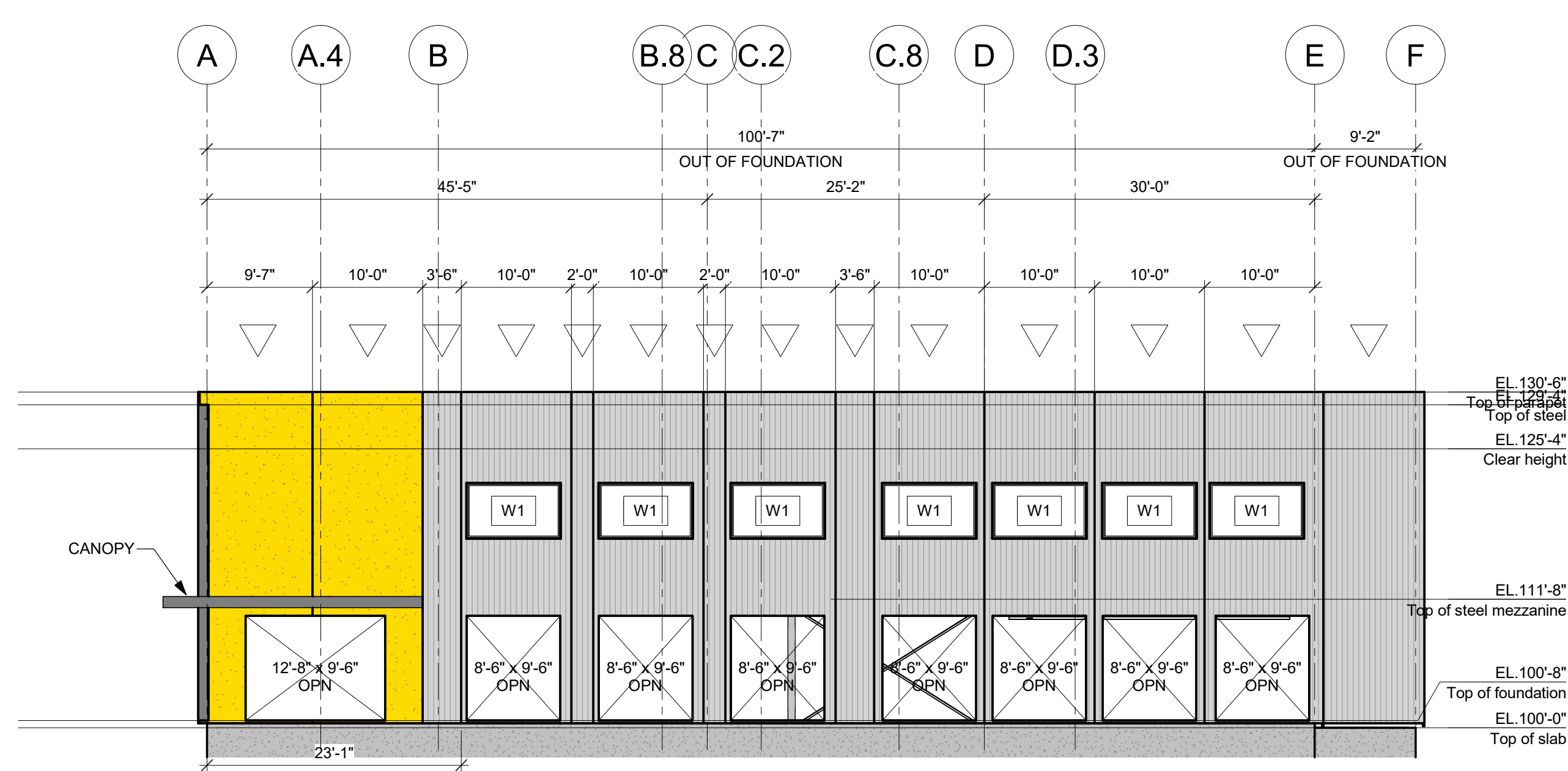
ELEVATION LINE 1 (WEST) 3/32" = 1'-0"
