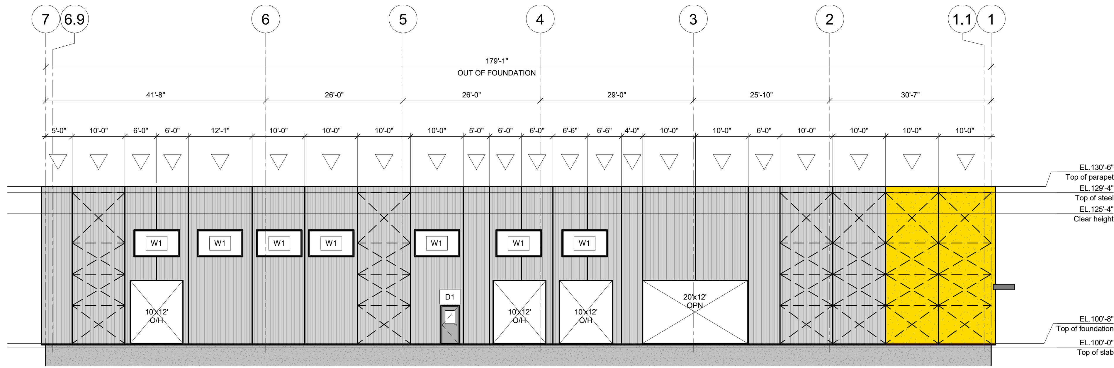
ELEVATION LINE A (NORTH) 3/32" = 1'-0"
