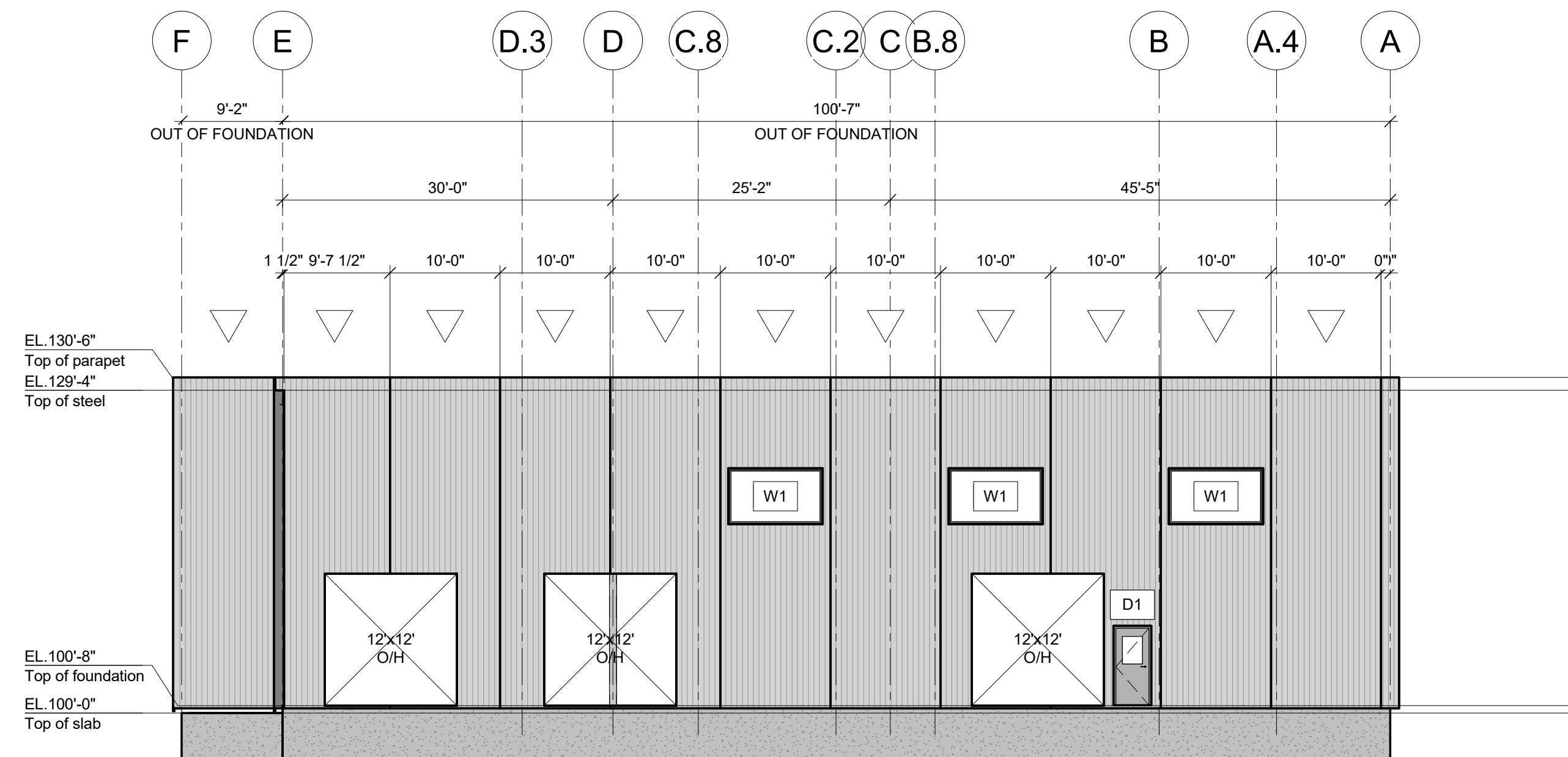
ELEVATION LINE 7 (EAST) 3/32" = 1'-0"
