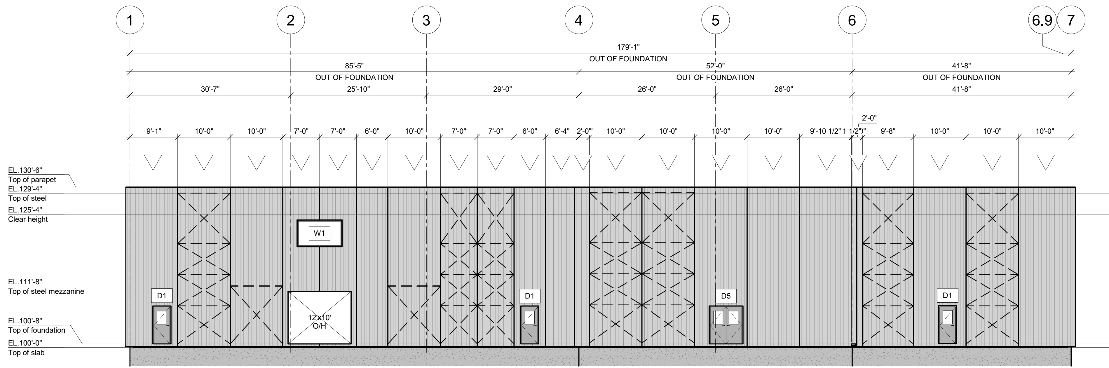
ELEVATION LINE E (SOUTH) 3/32" = 1'-0"
