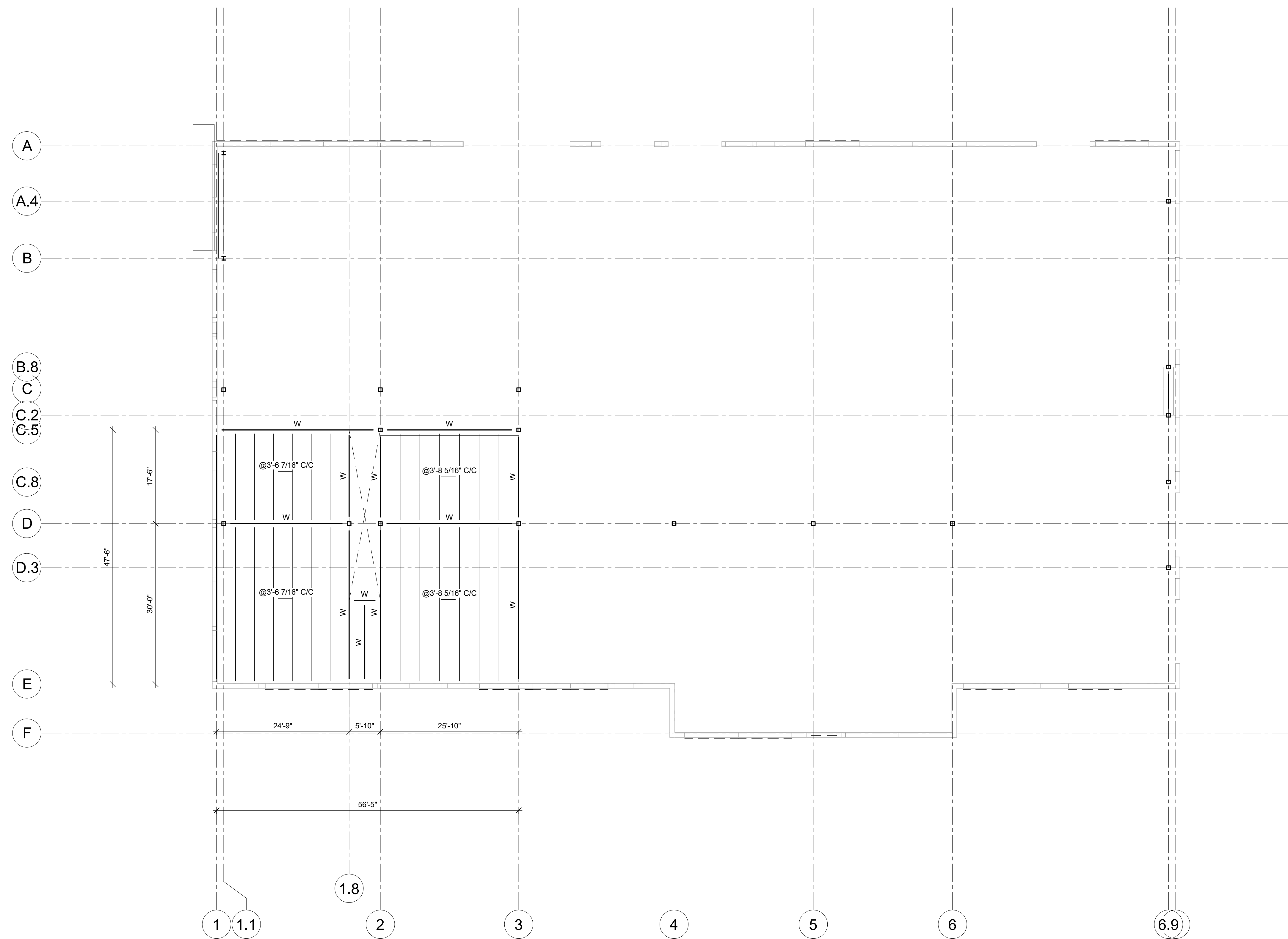
MEZZANINE PLAN 3/32" = 1'-0"
