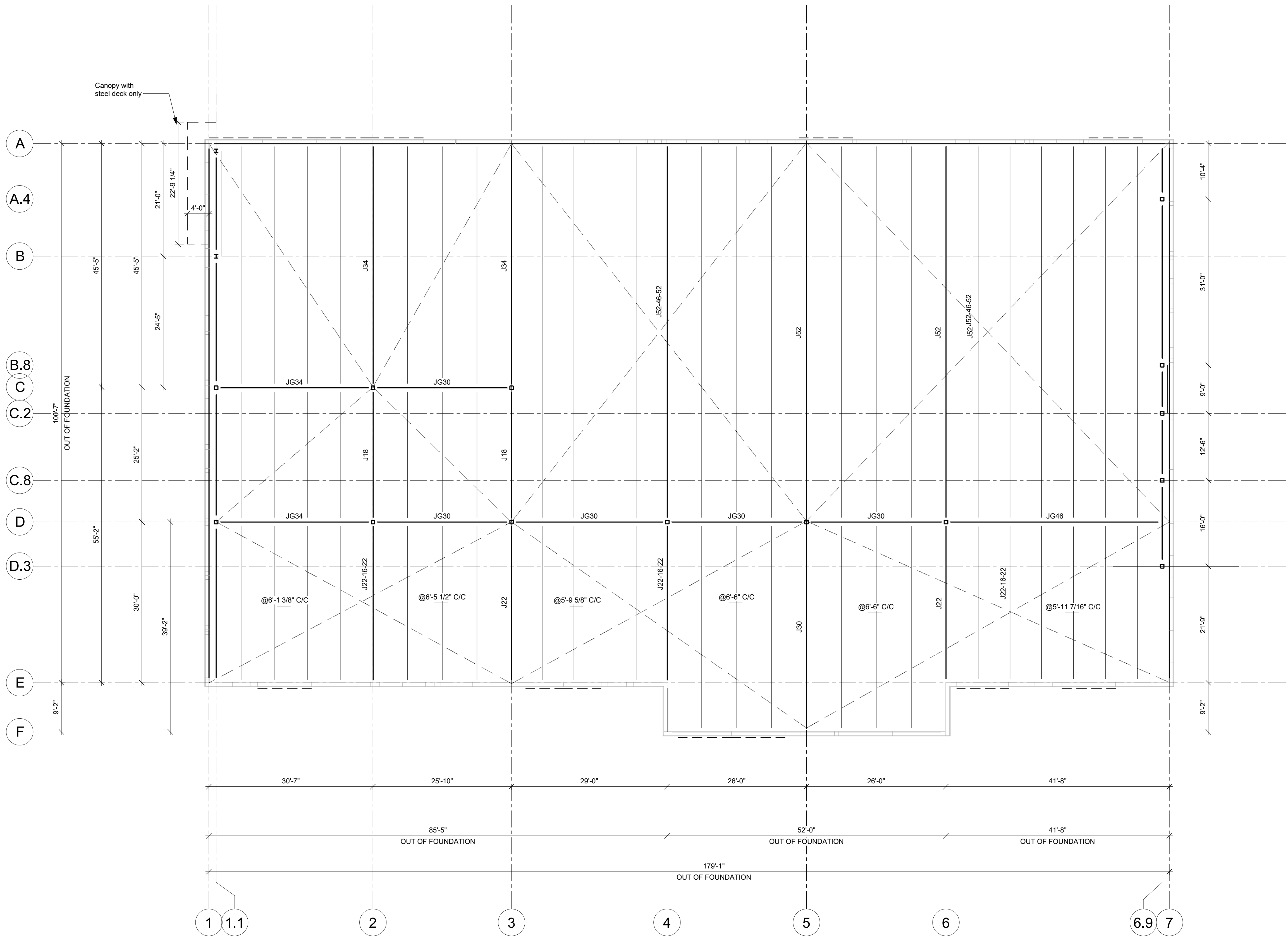
ROOF PLAN 1" = 10'-0"
