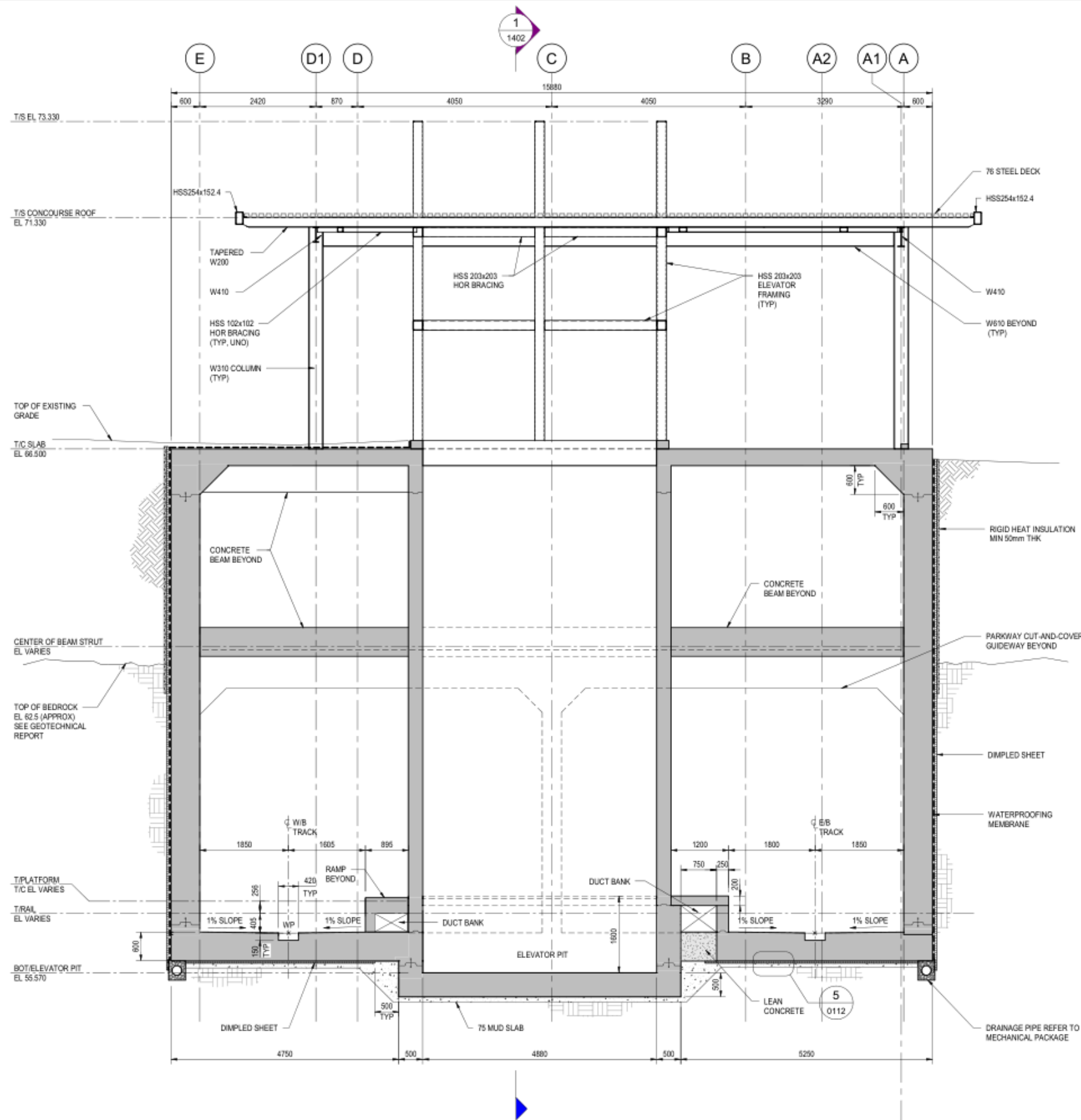
1 CROSS SECTION 1200 1:50
