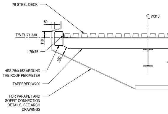
4 DETAIL 1230 1:20
