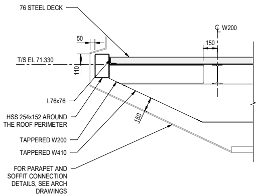
2 DETAIL 1230 1:20
