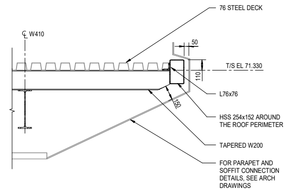
5 DETAIL 1230 1:20
