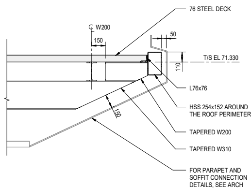
3 DETAIL 1230 1:20
