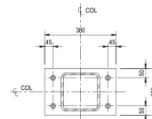
4 DETAIL 1270 1:10 BASE PLATE BPL3 (SEE NOTE 2)
