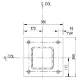
2 DETAIL 1270 1:10 BASE PLATE BPL1 (SEE NOTE 2)
