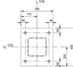
3 DETAIL 1270 1:10 BASE PLATE BPL2 (SEE NOTE 2)
