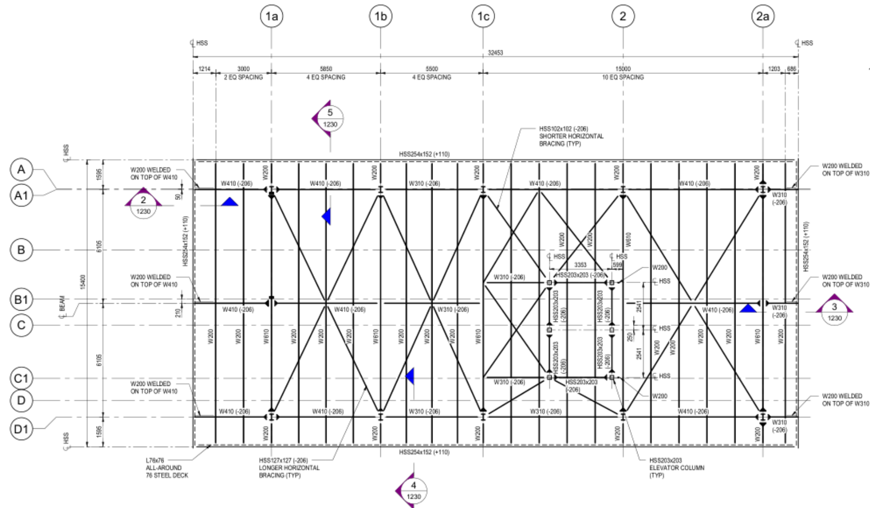
1 ROOF FRAMING PLAN - CONCOURSE (T/S EL 71.330) 1230 1:100
