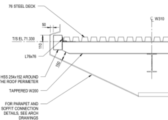
4 DETAIL 1230 1:20
