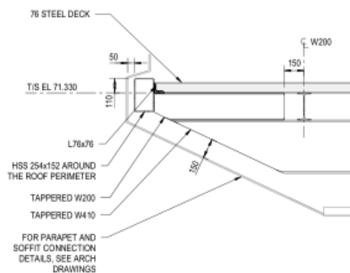
2 DETAIL 1230 1:20
