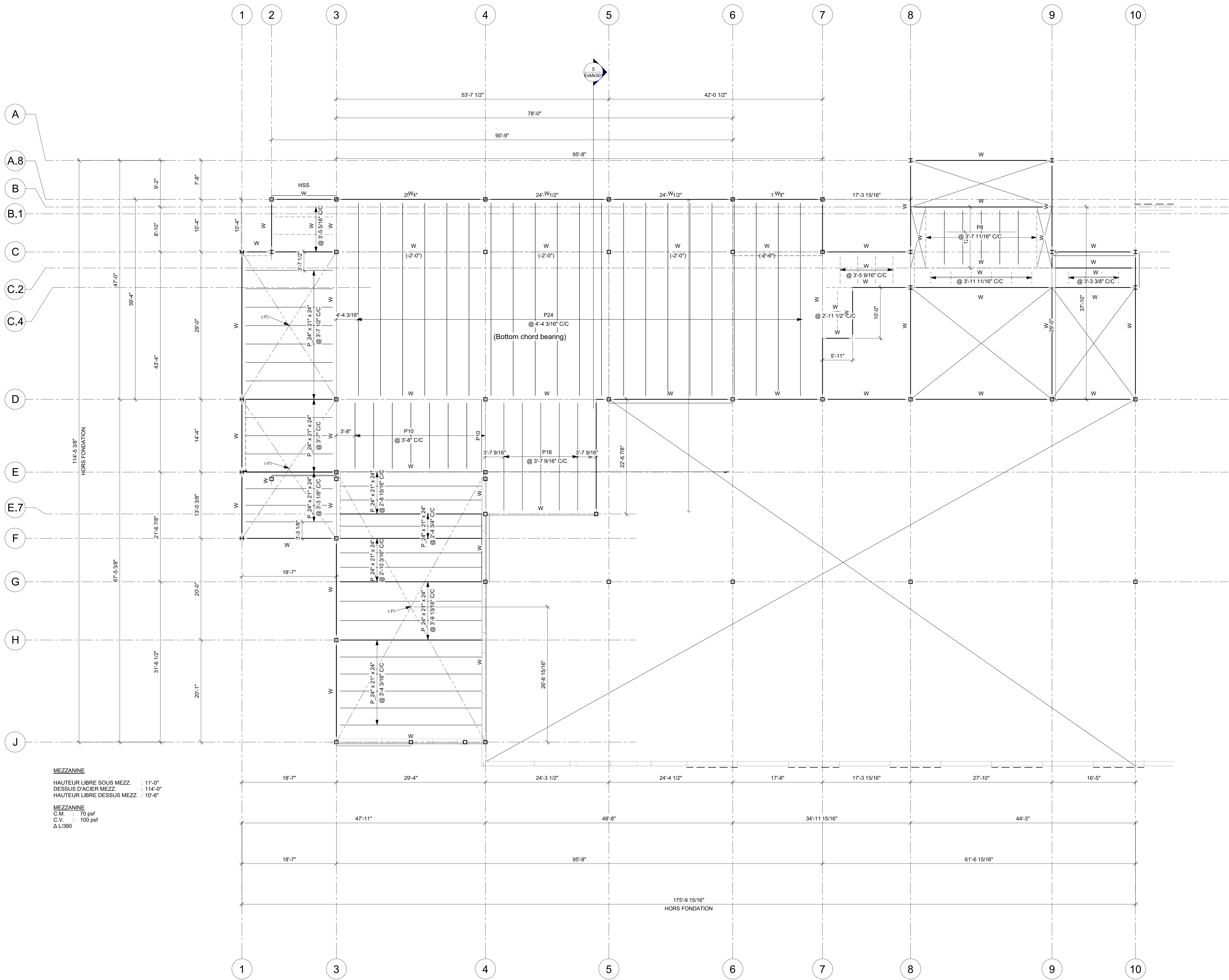
PLAN DE MEZZANINE 1/8" = 1'-0"
