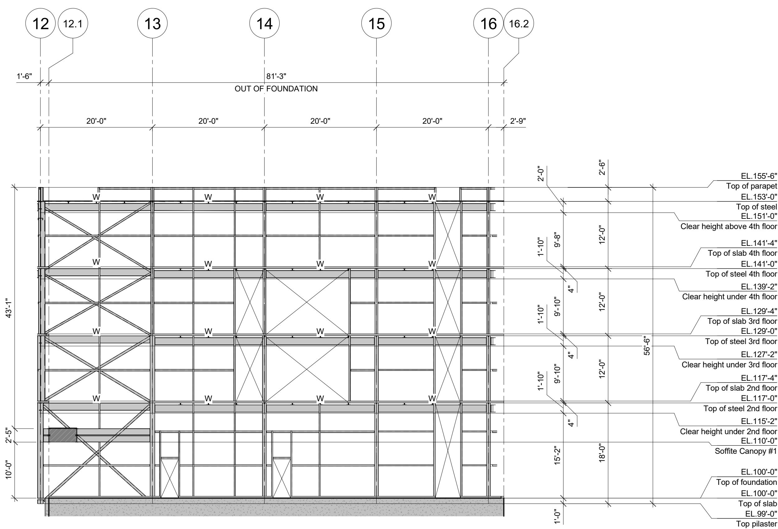
ELEVATION LINE F1 (EAST)
