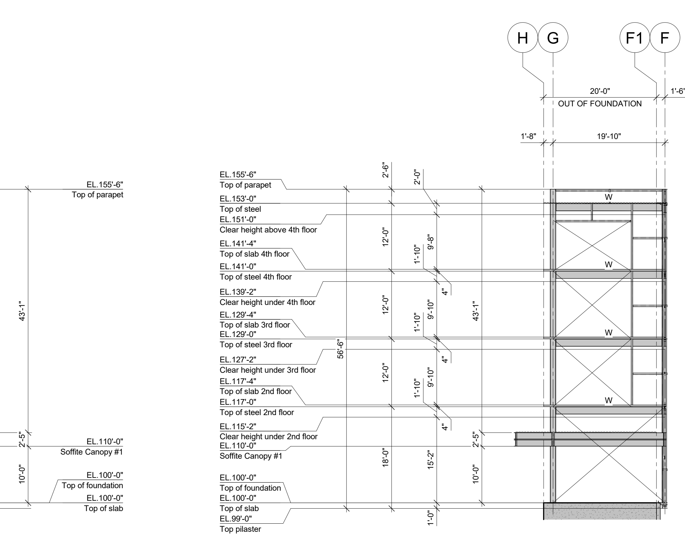
ELEVATION LINE 12.1 (NORTH)
