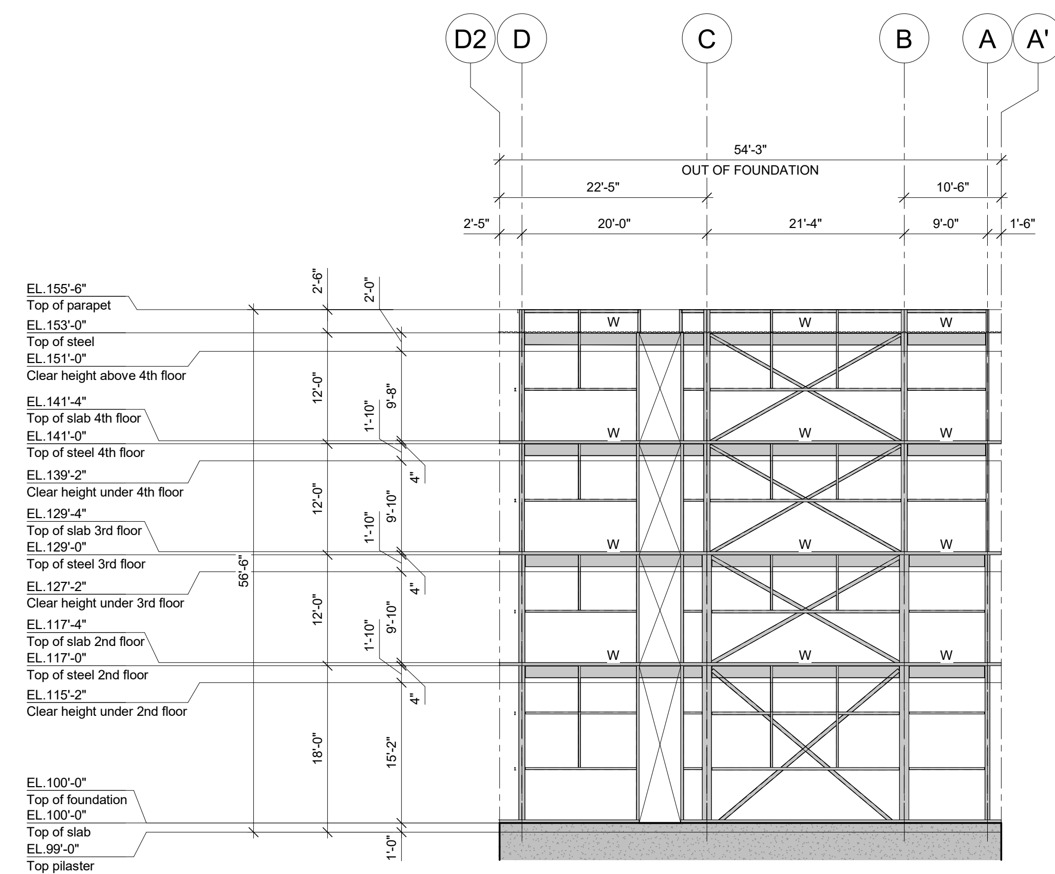
ELEVATION LINE 19 (NORTH)
