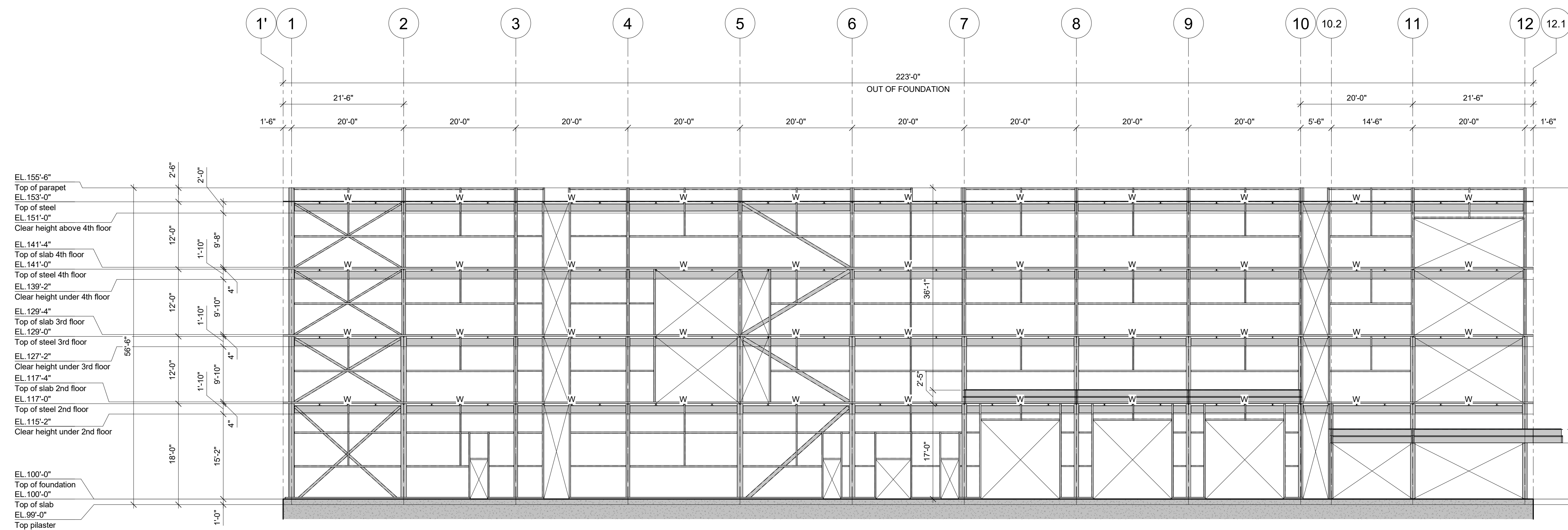
ELEVATION LINE H (EAST)
