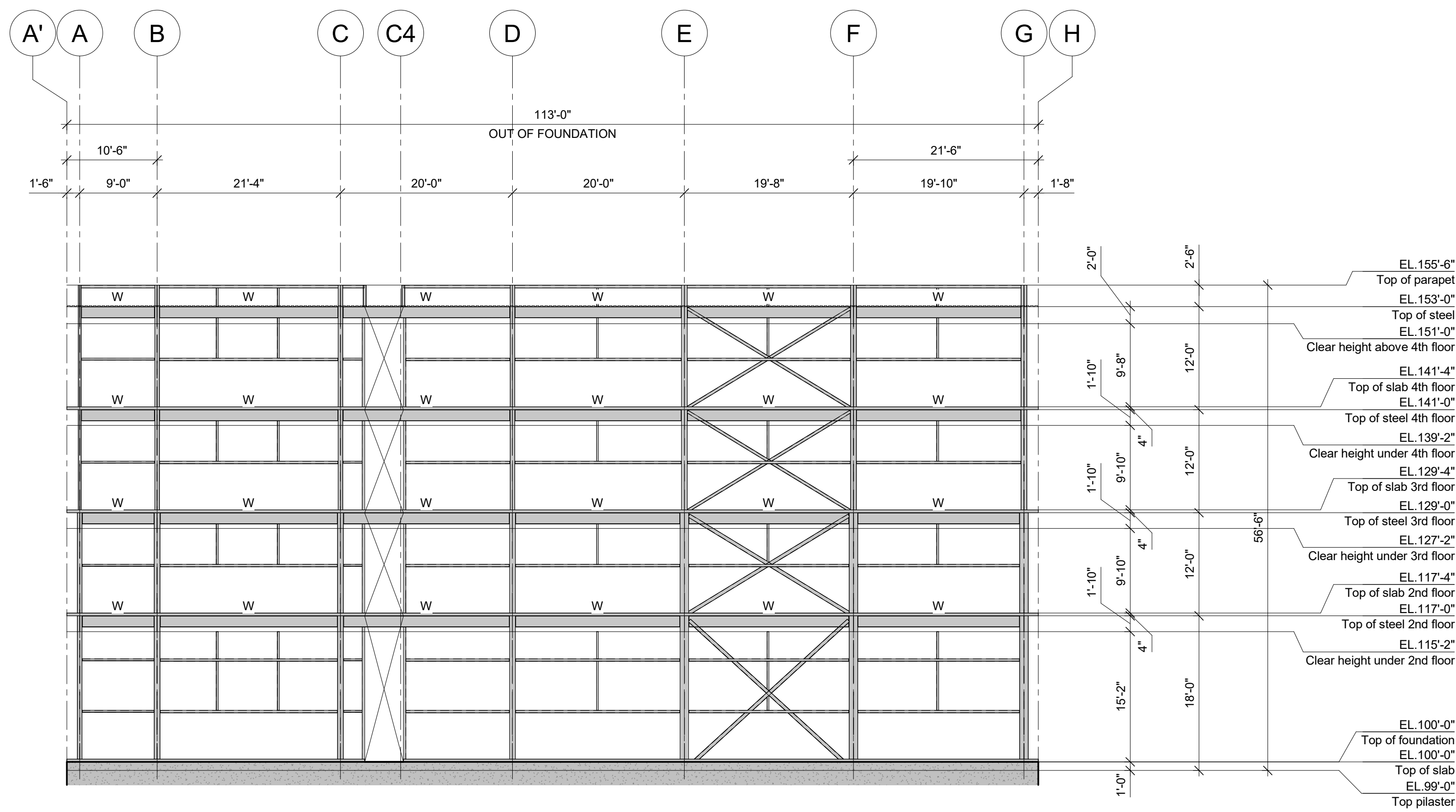
ELEVATION LINE 1' (SOUTH) 3/32" = 1'-0"
