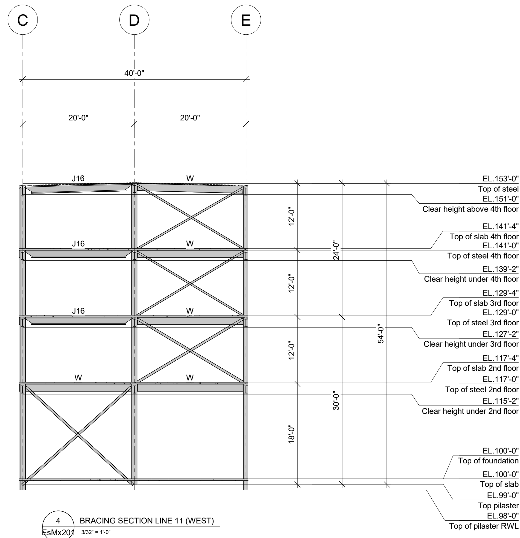
4 BRACING SECTION LINE 11 (WEST) 3/32" = 1'-0"
