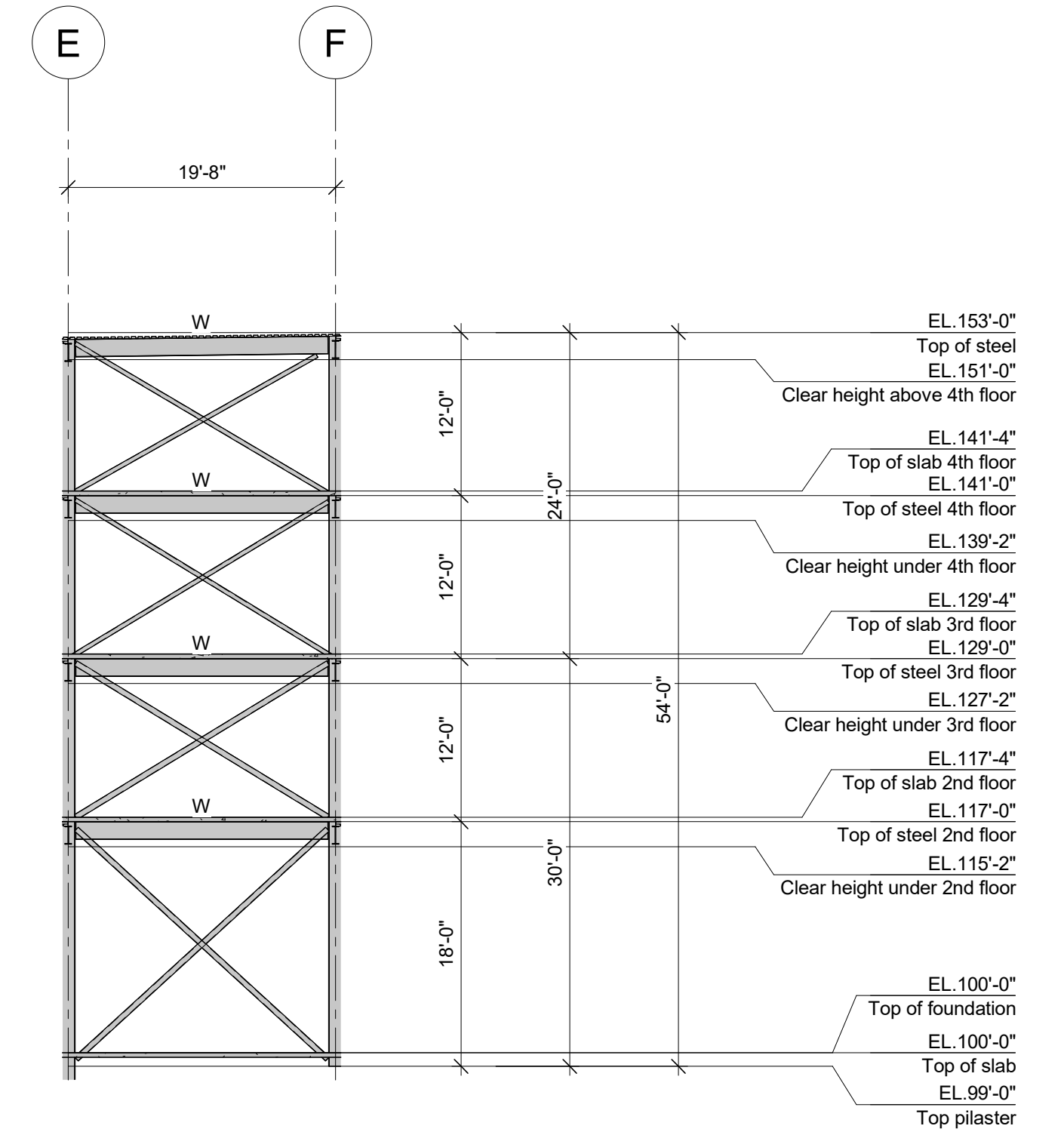
3 BRACING SECTION LINE 7 (WEST) 3/32" = 1'-0"
