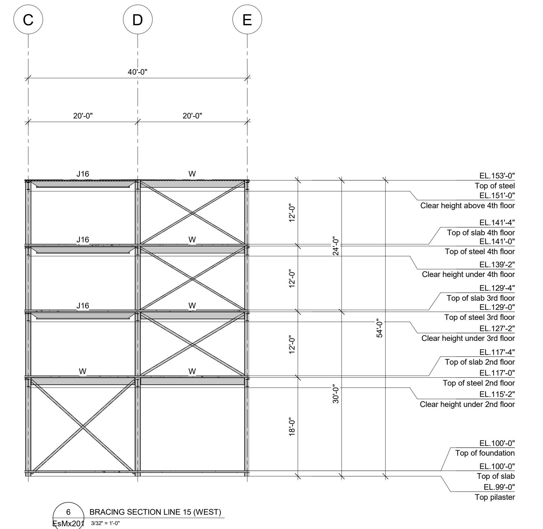
6 BRACING SECTION LINE 15 (WEST) 3/32" = 1'-0"
