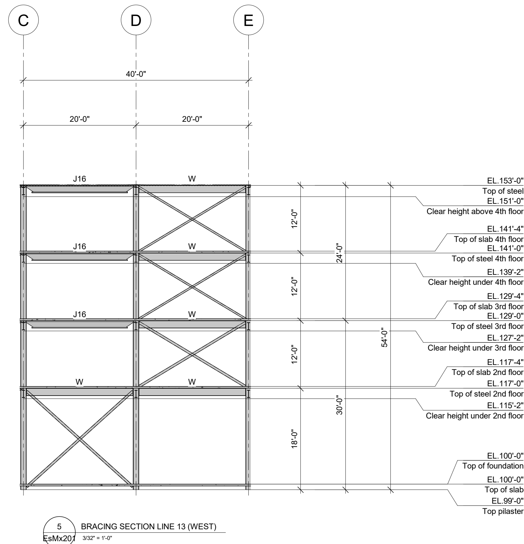
5 BRACING SECTION LINE 13 (WEST) 3/32" = 1'-0"
