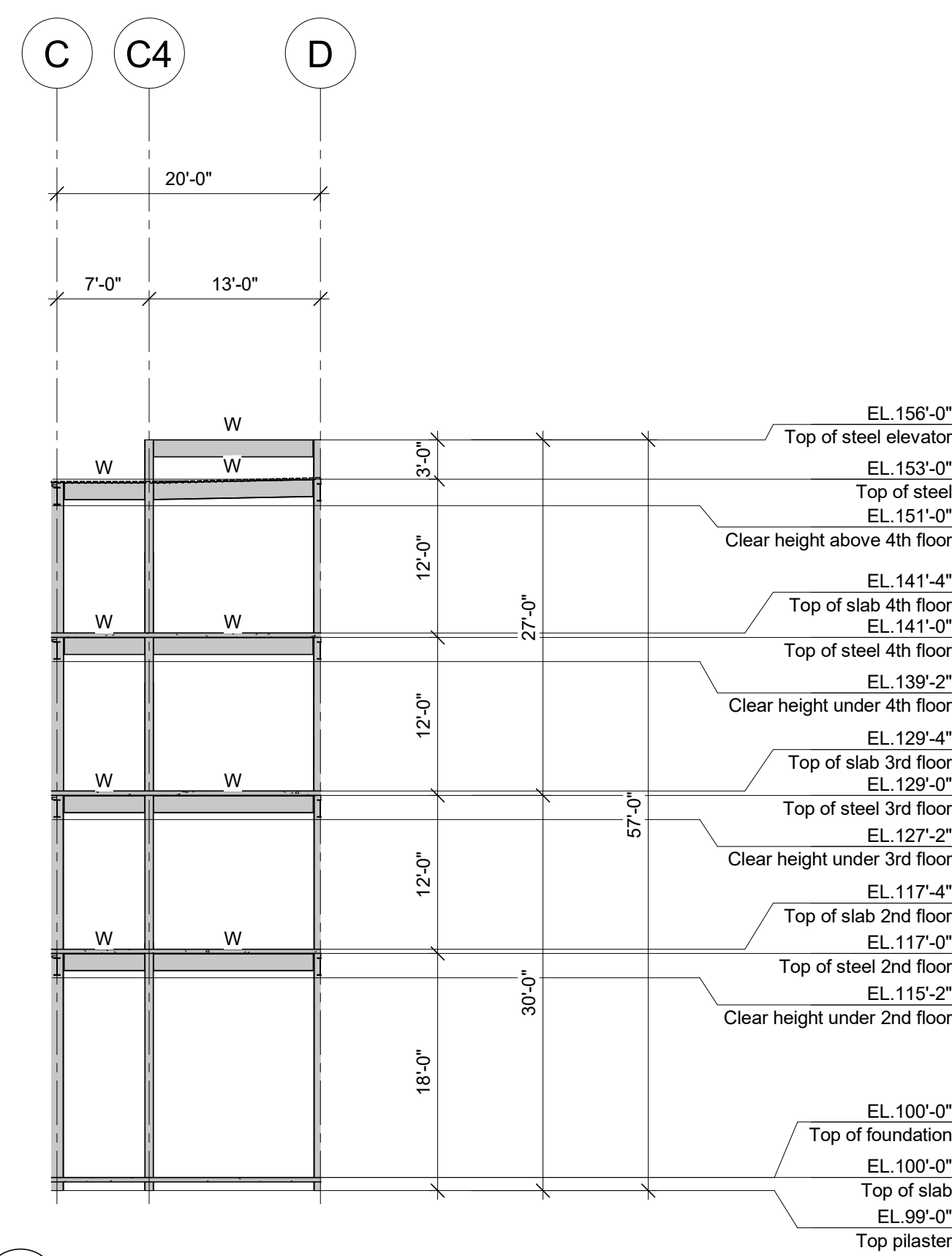
7 ELEVATOR SECTION LINE 8 (WEST) 3/32" = 1'-0"
