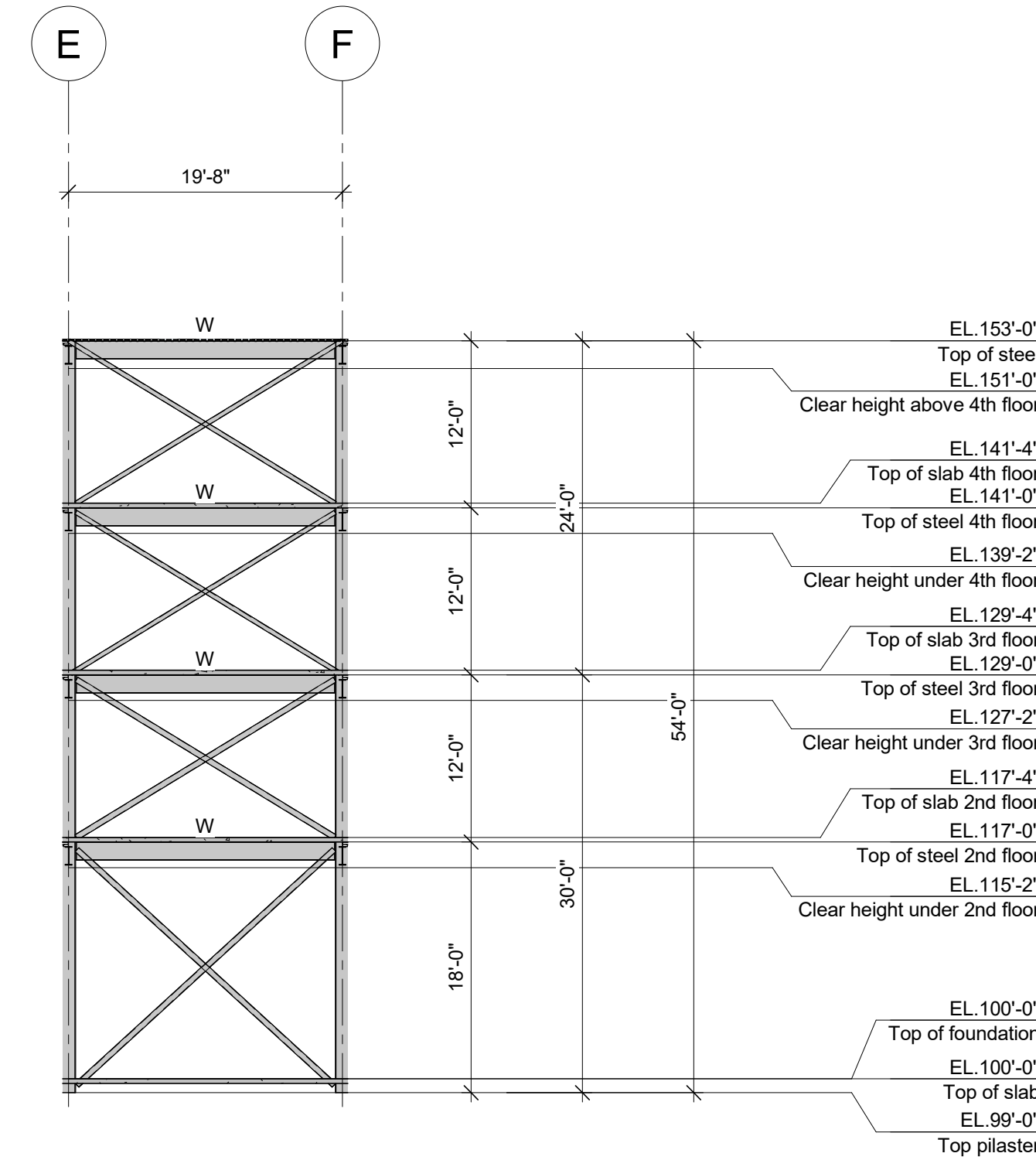
2 BRACING SECTION LINE 5 (WEST) 3/32" = 1'-0"
